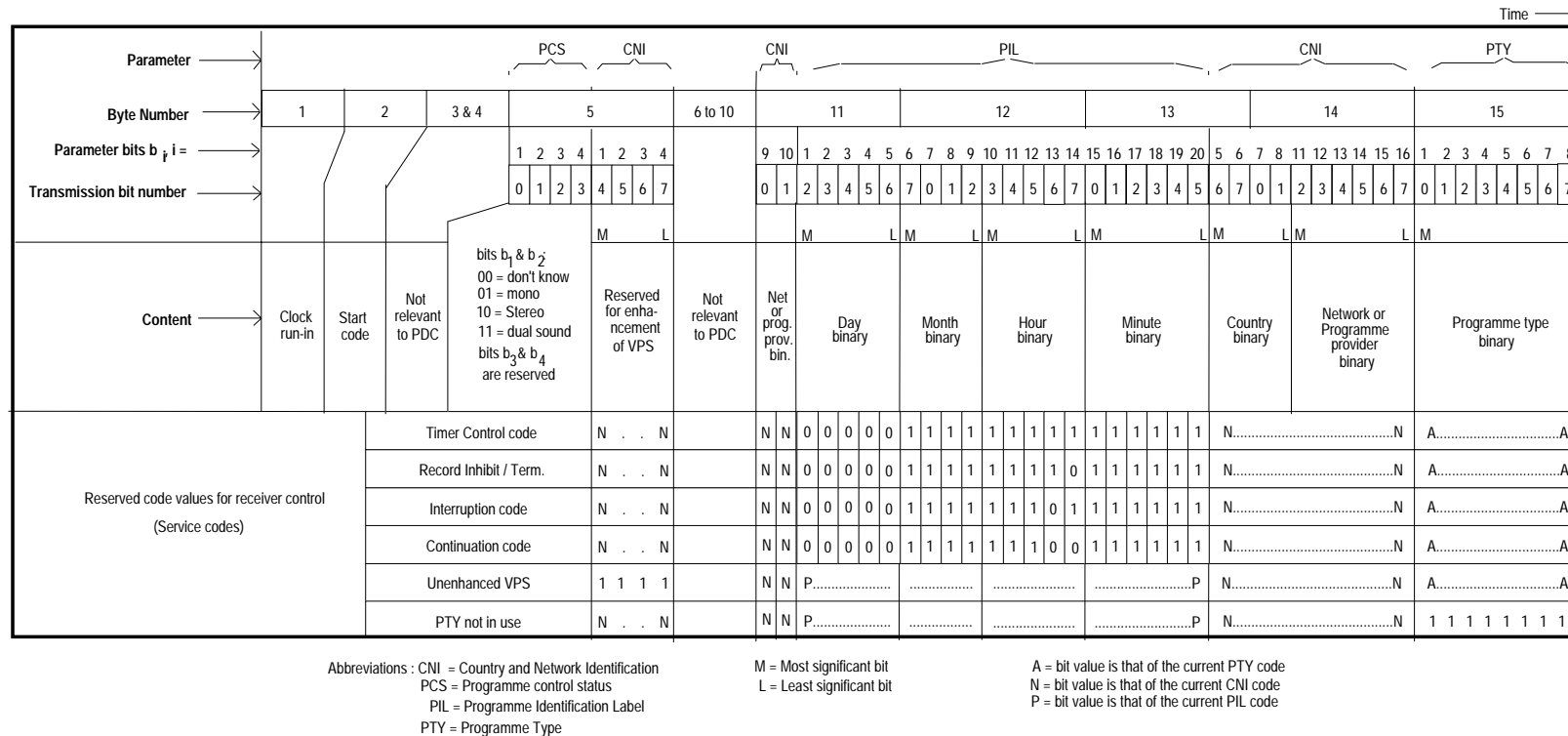
Figure 9: Data format of the programme delivery data in the dedicated TV line
