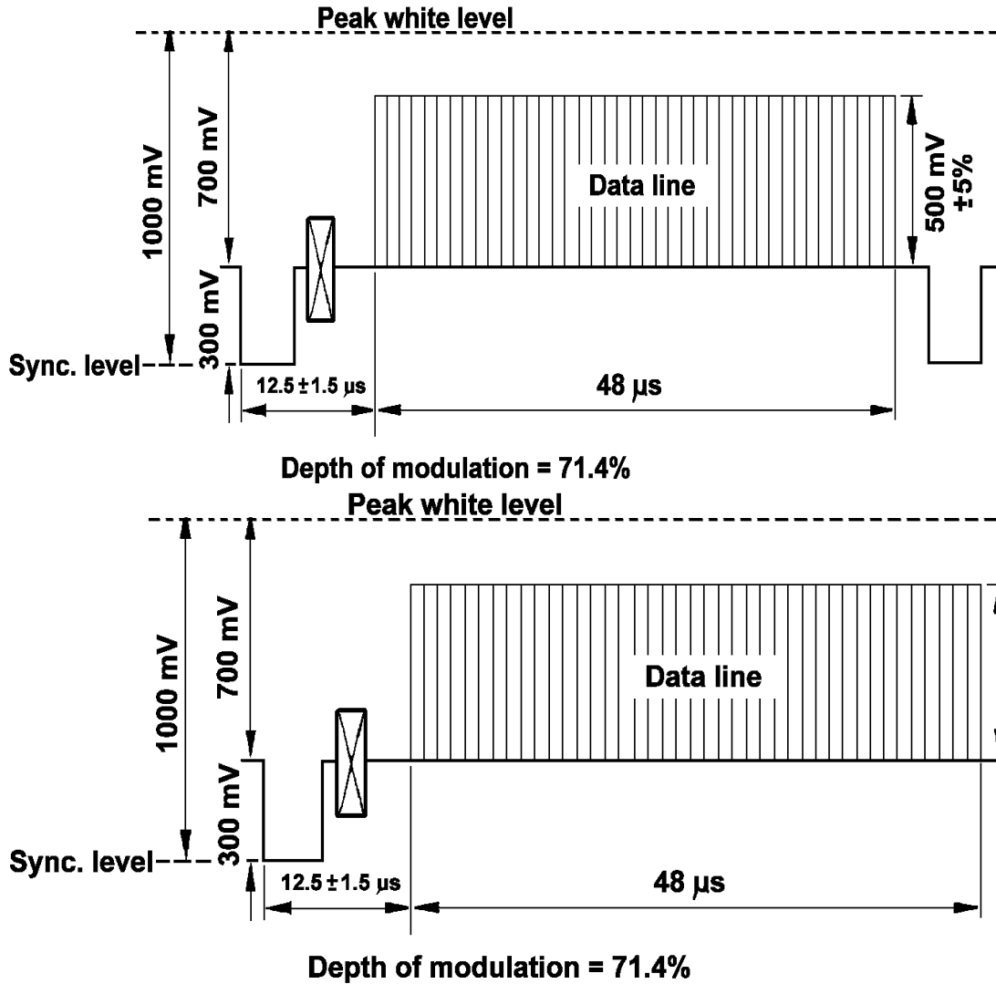
Figure 8: Insertion of the data line into the video signal
