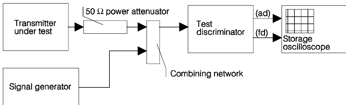
Figure 2: Measurement arrangement
