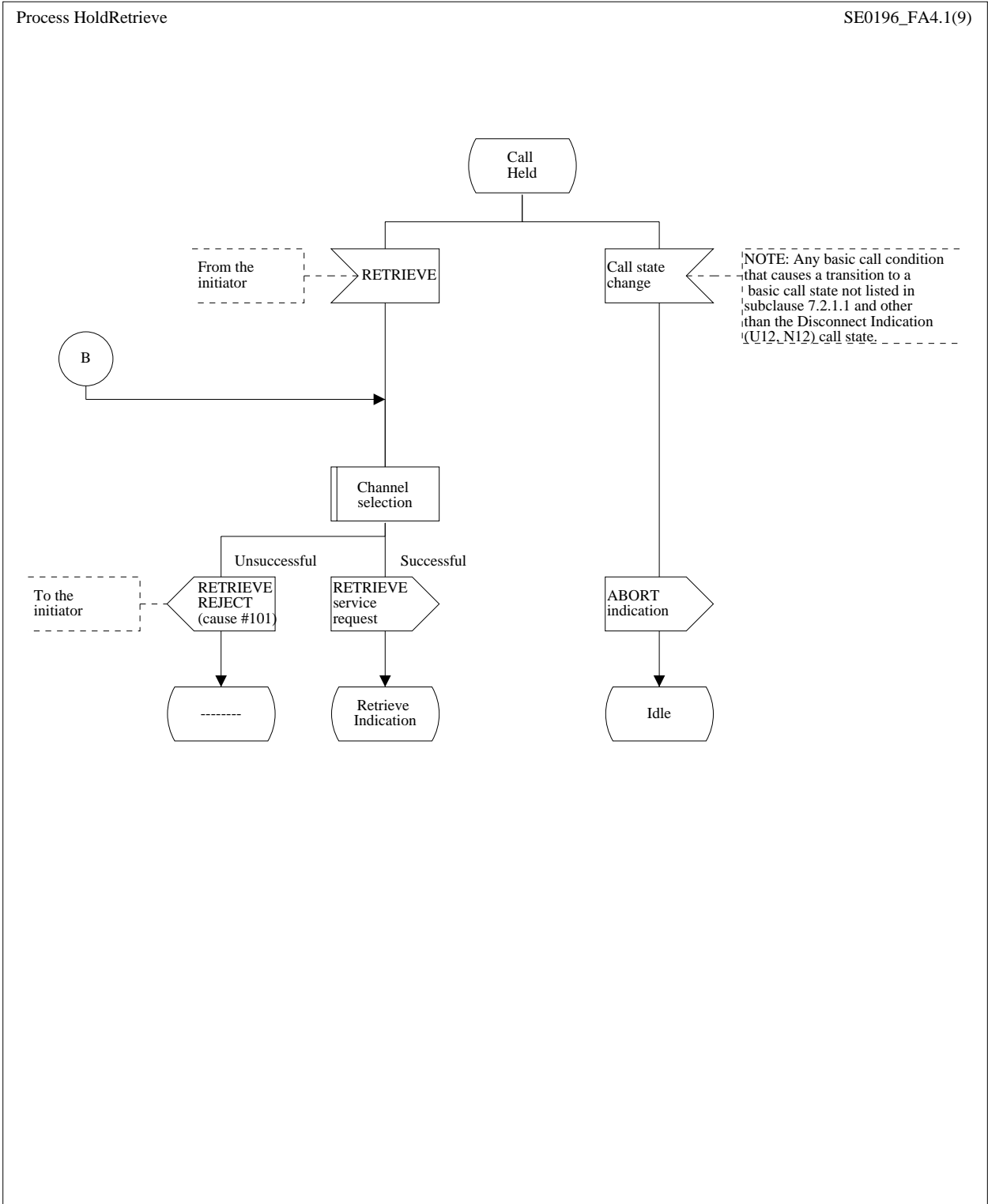
Figure A.4 (sheet 1 of 2): Retrieve function responding entity SDL diagrams
