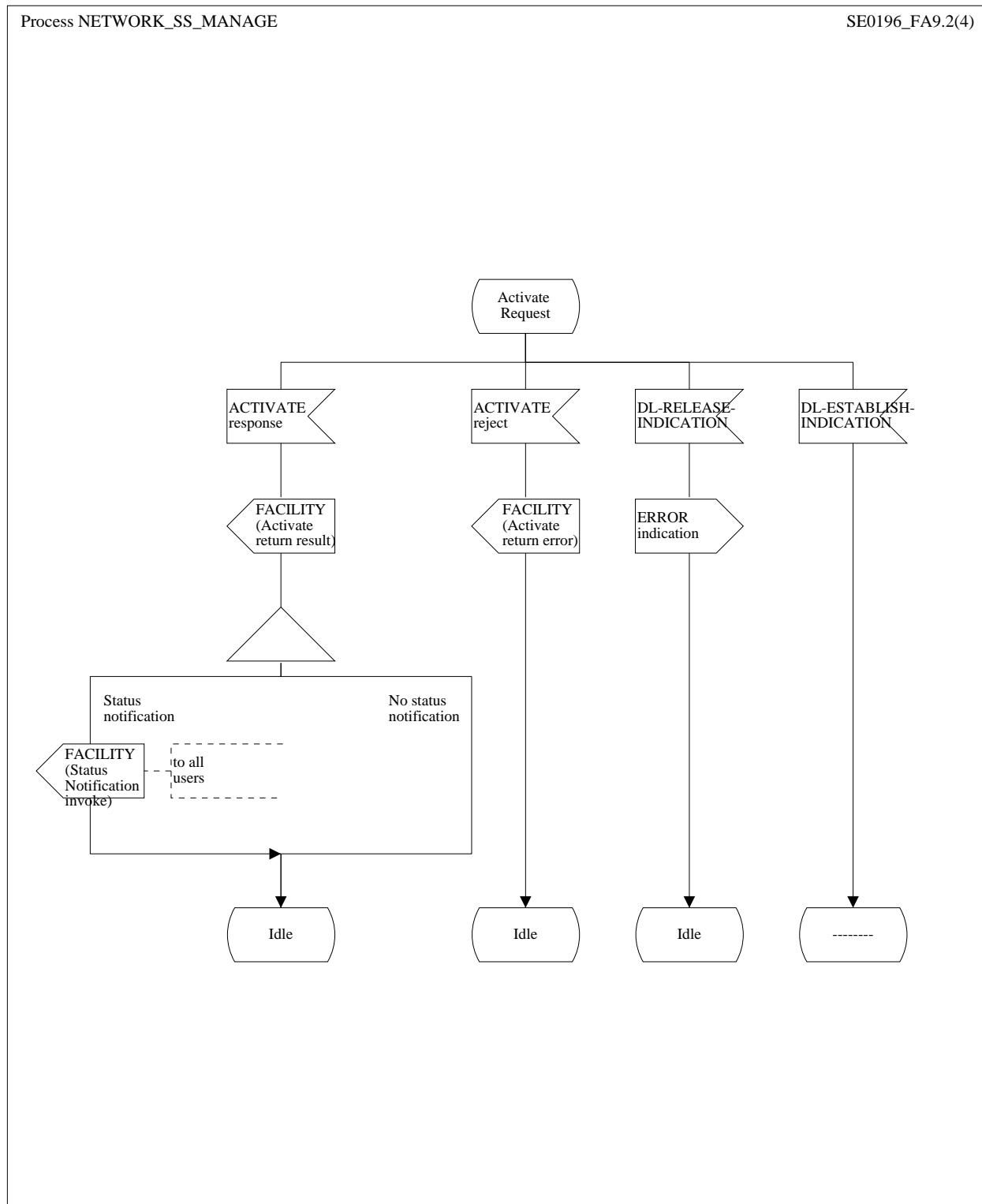
Figure A.9 (sheet 2 of 4): Supplementary service management procedures - network SDL diagrams
