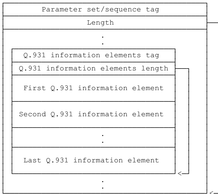
Figure F.1: Encapsulation of Q.931 information elements
