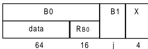
Figure 22: Half slot B-field protected format
