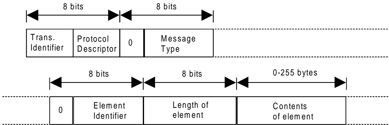
Figure 11: NWK Layer Message Structure (NLMS)
