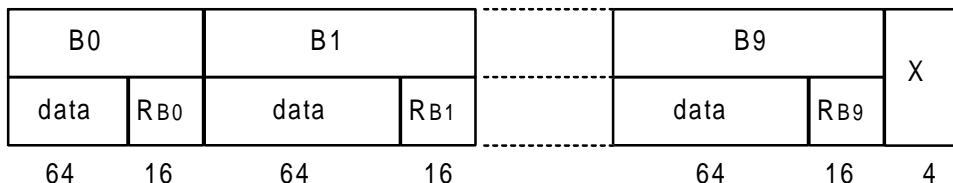
Figure 23b: Double slot B-field protected format
