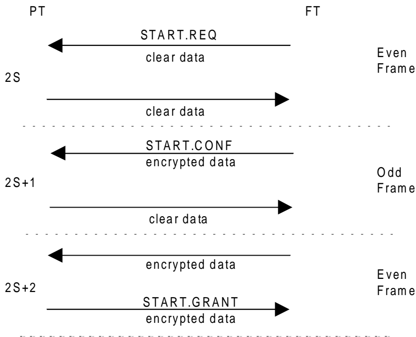
Figure 17: Encryption start - good link example
