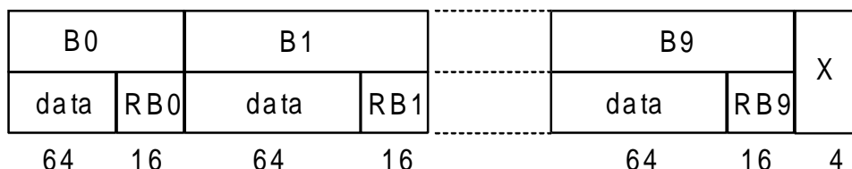
Figure 23b: Double slot B-field protected format
