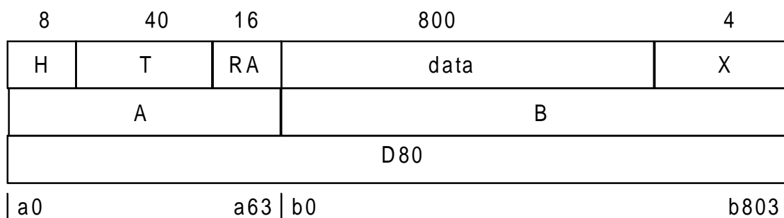
Figure 23a: Double slot field structures
