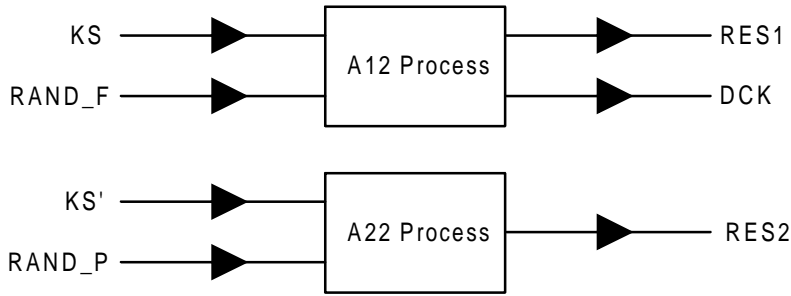
Figure 8: Derivation of RES1, DCK and RES2
