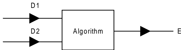
Figure 10: A algorithm
