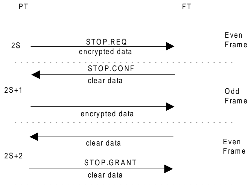
Figure 19: Encryption stop - good link example
