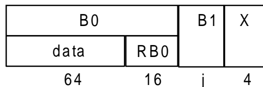
Figure 22: Half slot B-field protected format
