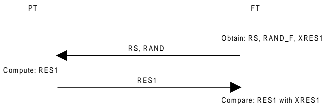
Figure 2: Authentication of PT
