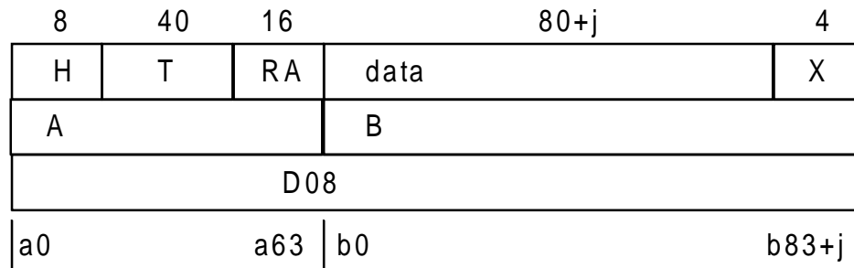
Figure 21: Half slot field structures
