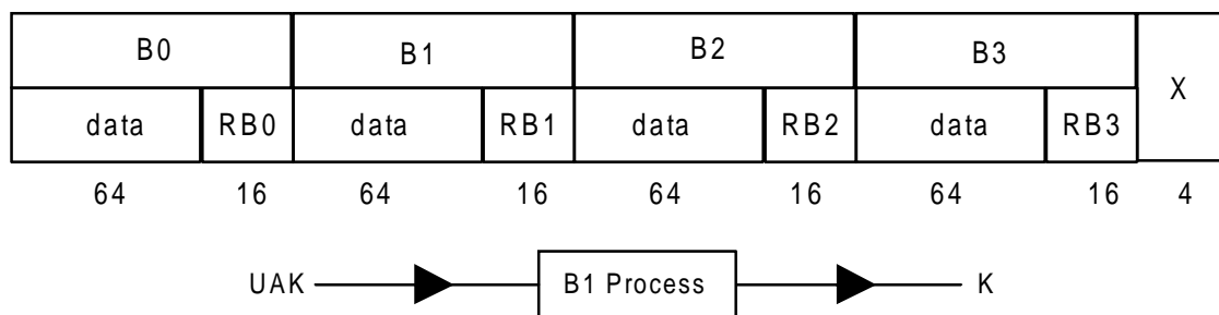
Figure 4: Derivation of K from UAK
