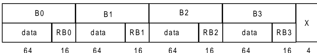
Figure 15: B-field protected format
