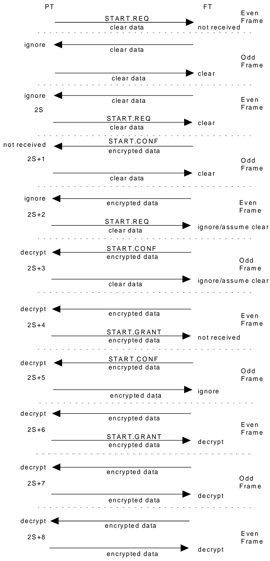
Figure 18: Encryption start - poor link example
