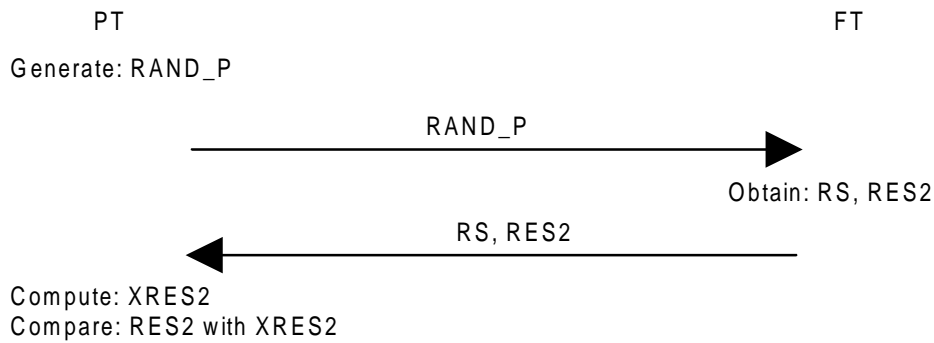
Figure 3: Authentication of FT
