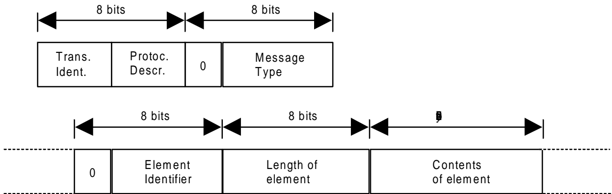
Figure 11: NWK Layer Message Structure (NLMS)
