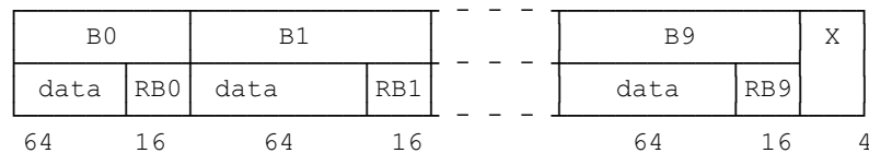
Figure 23b: Double slot B-field protected format
