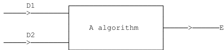
Figure 10: A algorithm
