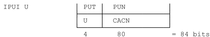
Figure 26: IPUI U
