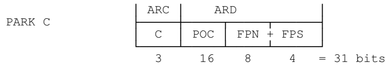
Figure 17: PARK C
