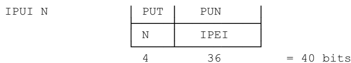
Figure 20: IPUI N
