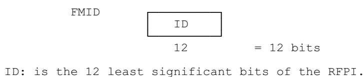
Figure 29: FMID structure
