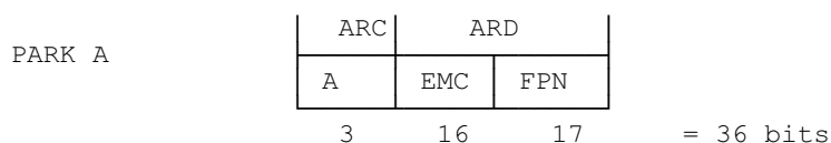
Figure 15: PARK A
