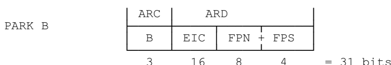
Figure 16: PARK B
