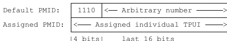
Figure 30: PMID structure
