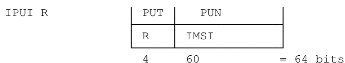
Figure 27: IPUI R
