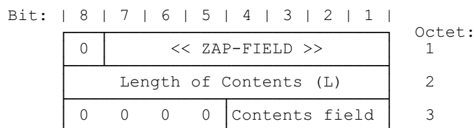
ZAP-FIELD information element
