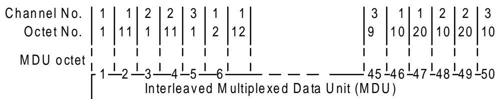
Example of interleaved packing (MCS Ref: P2/16)
