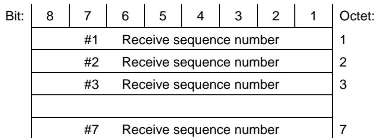
Frame format type FU6b
