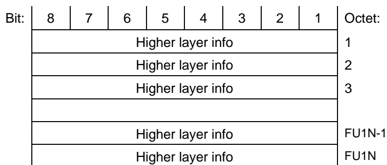
Frame Format Type FU1
