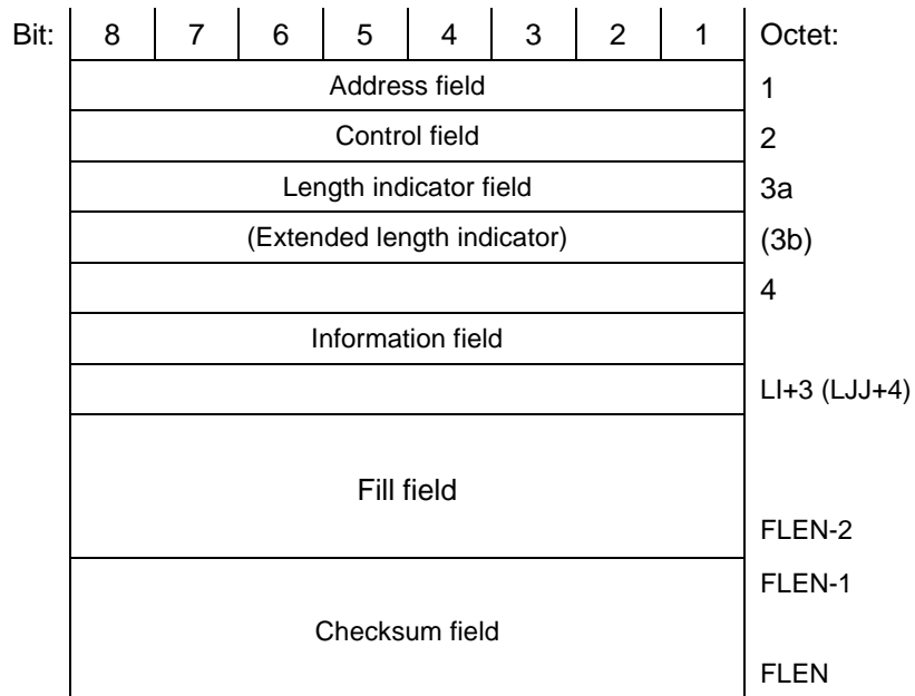
Frame format type FA
