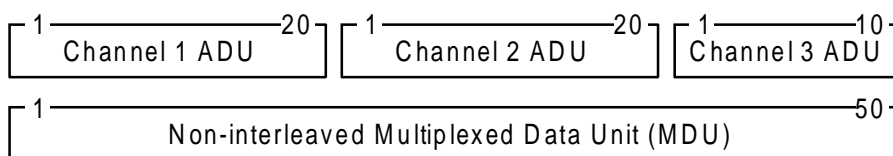
Example of non-interleaved packing (MCS Ref: P2/16)
