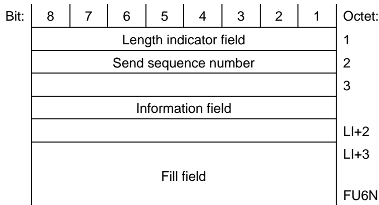
Frame format type FU6a
