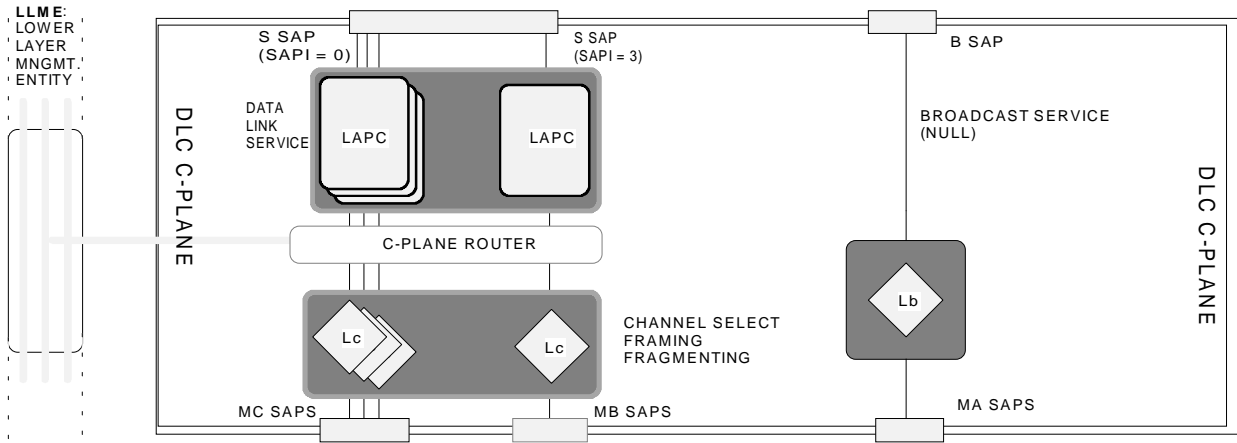
Figure 1: C-plane model
