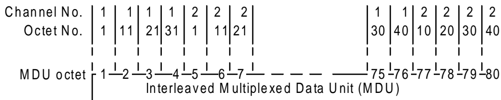
Example of interleaved packing (MCS Ref: N2/32)
