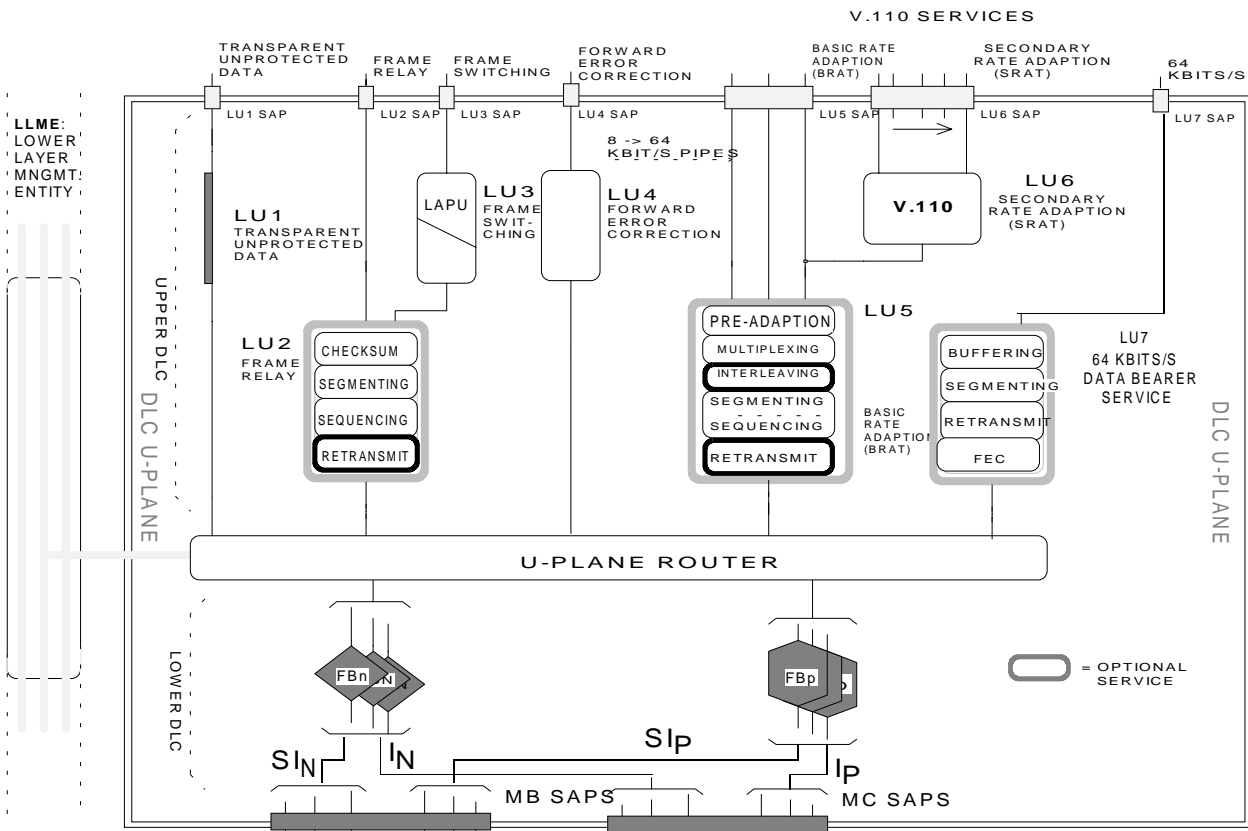
Figure 2: U-plane model
