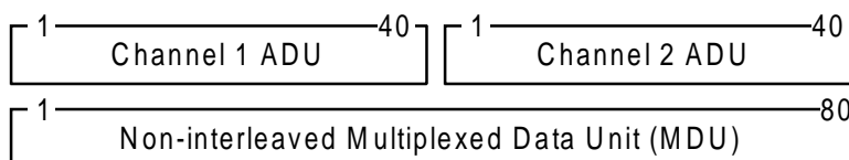
Example of non-interleaved packing (MCS Ref: N2/32)
