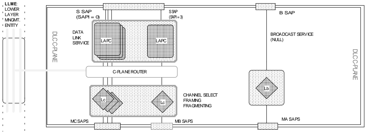
Figure 1 : C-plane model
