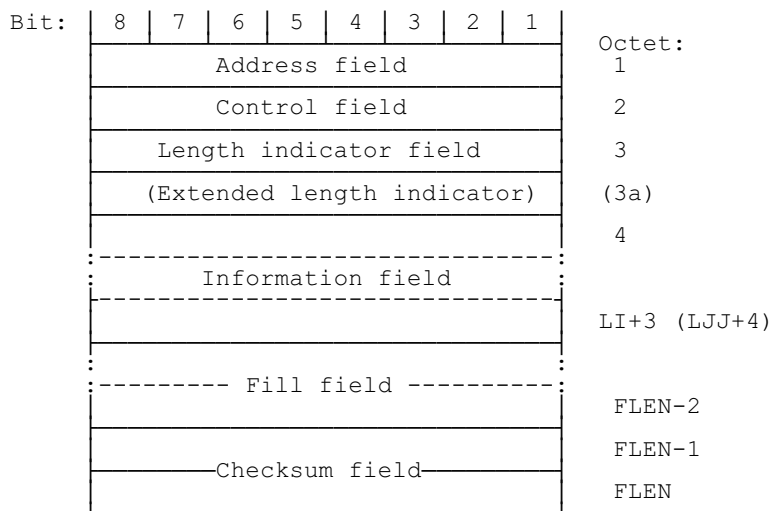
Frame format type FA
