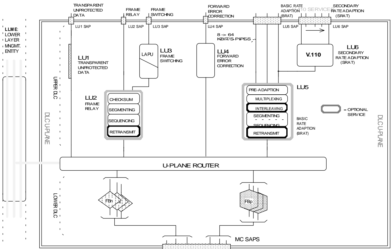
Figure 2 : U-plane model
