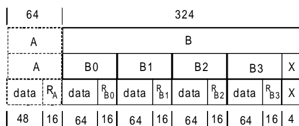
Figure 22: Protected B-field format (full slot)
