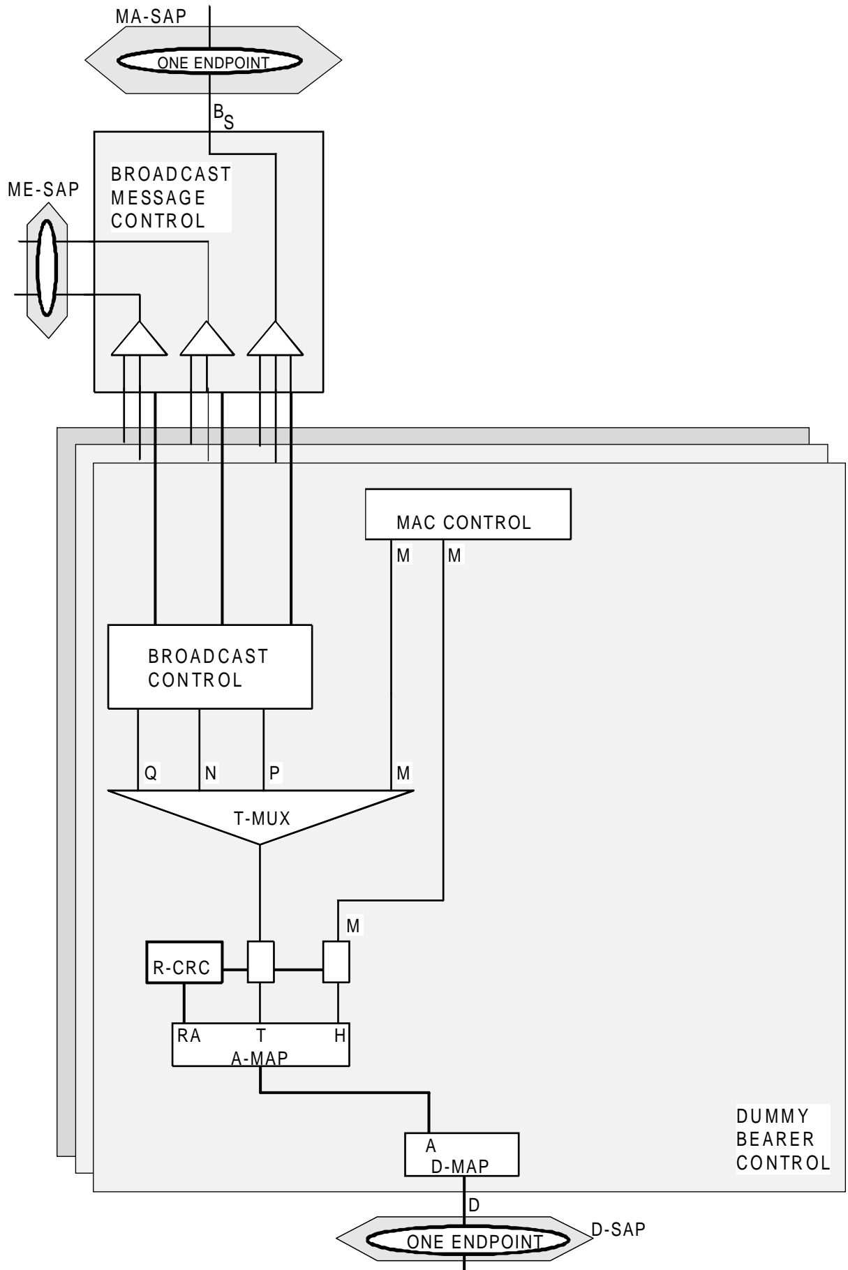
Figure 11: DBC multiplexing
