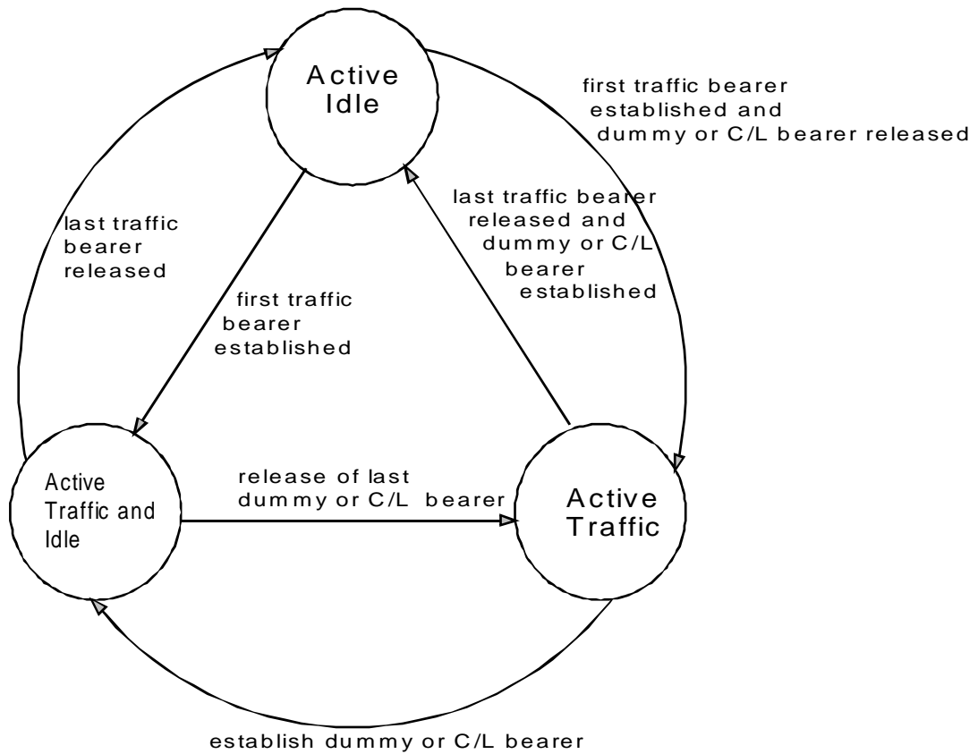
Figure 8: RFP state diagram
