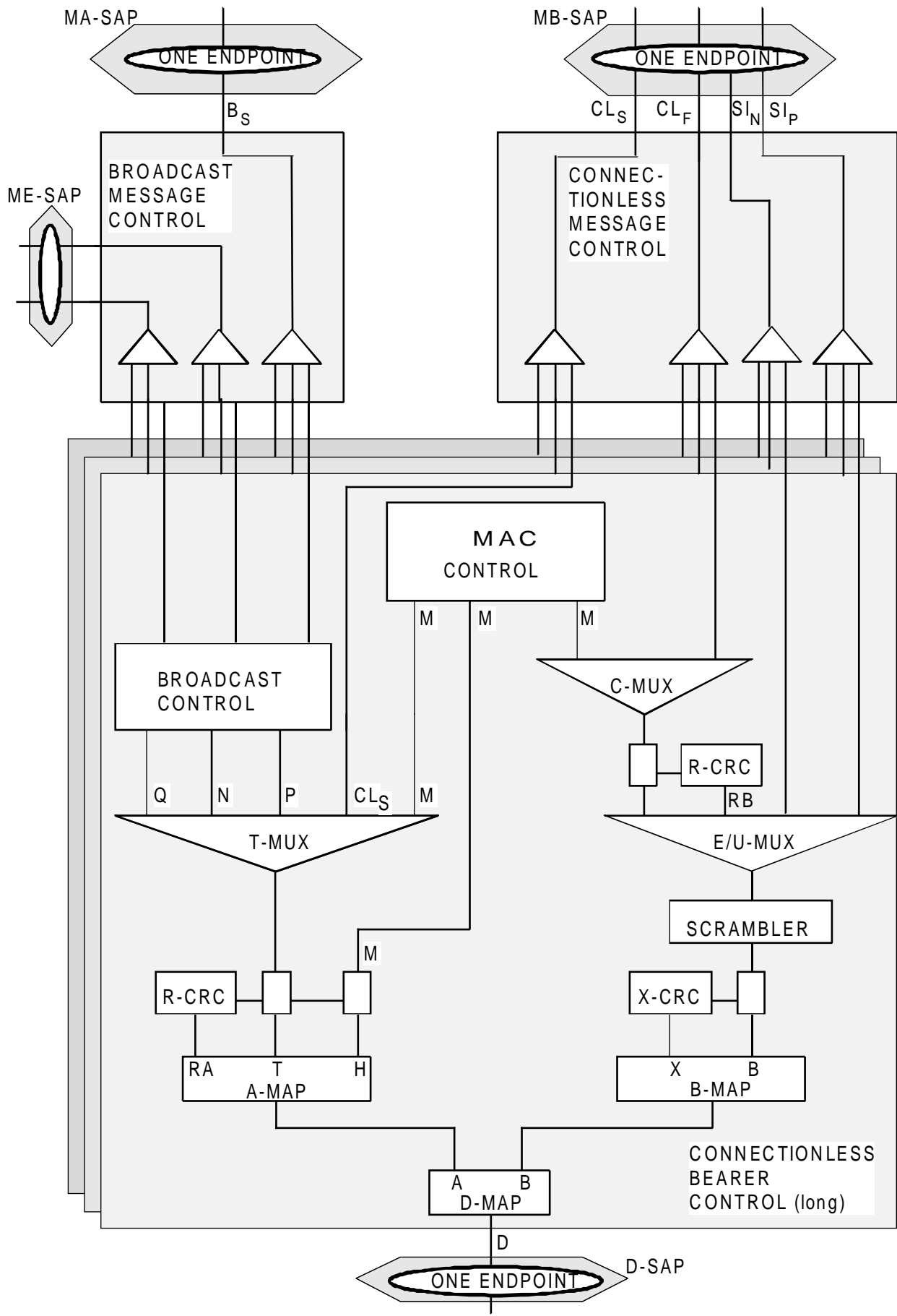
Figure 10: CBC multiplexing (long)
