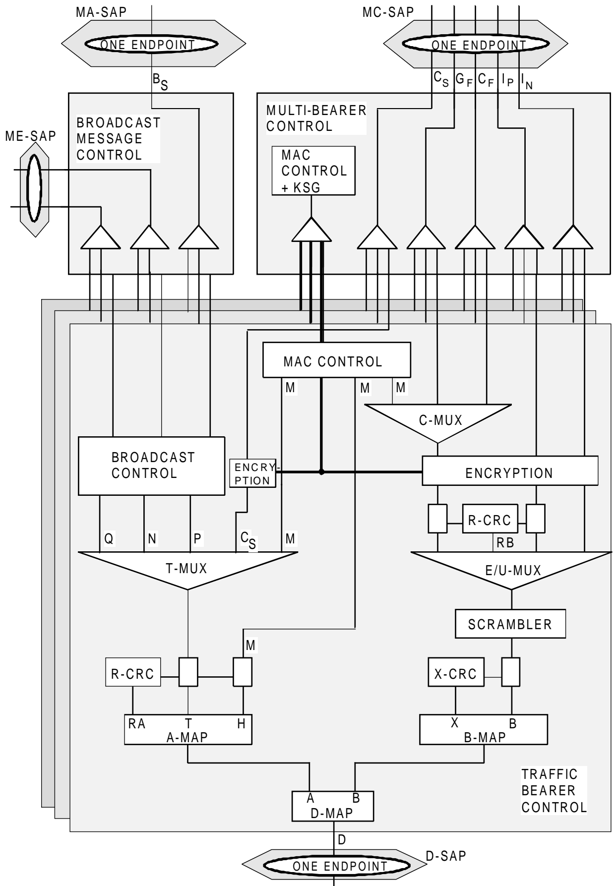
Figure 9: TBC multiplexing
