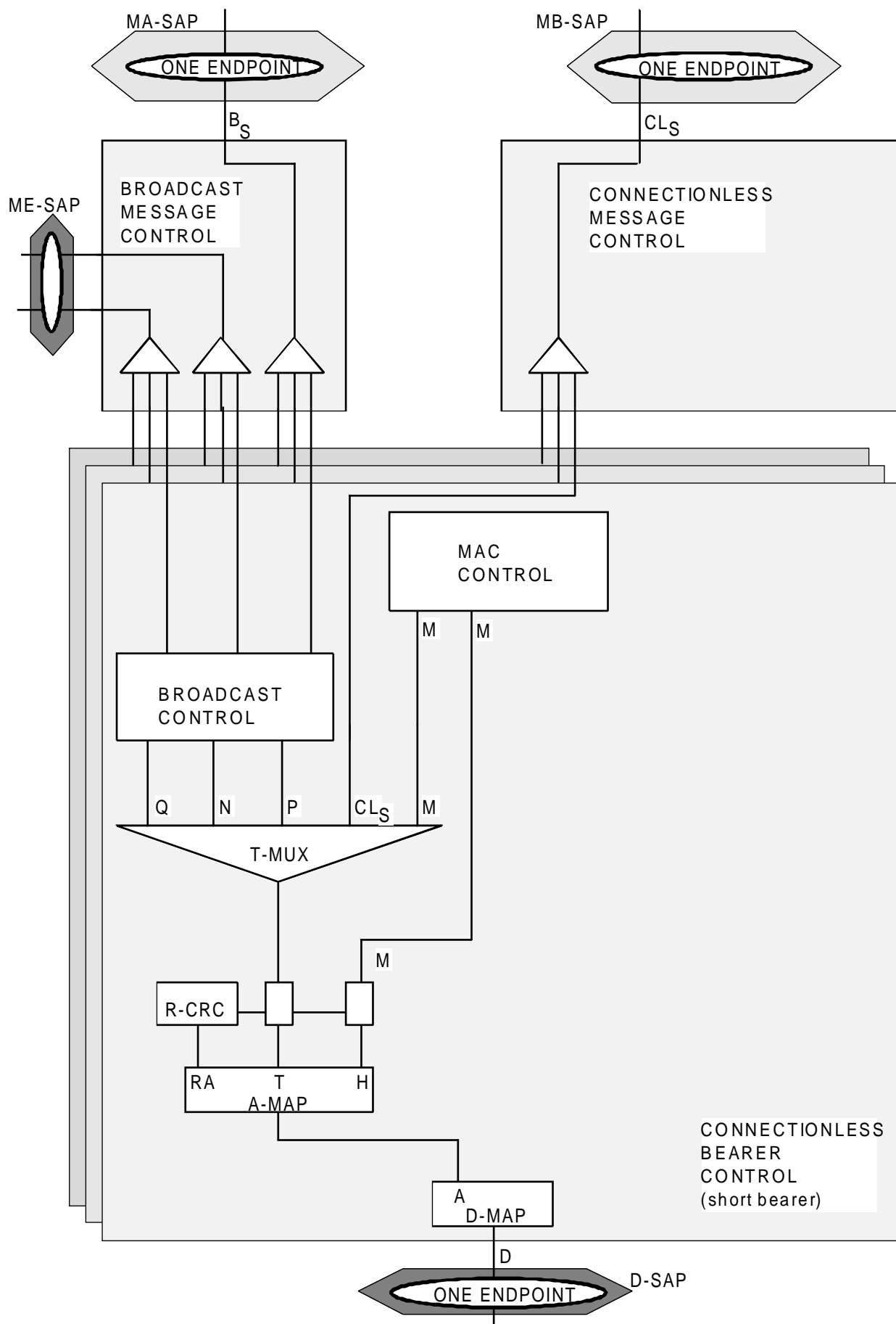
Figure 12: CBC multiplexing (short)
