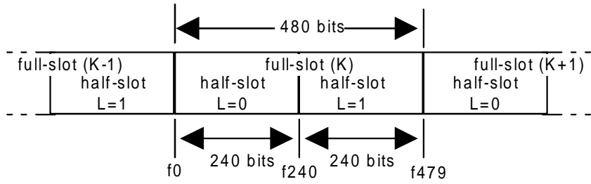
Figure 2: Half-slot format
