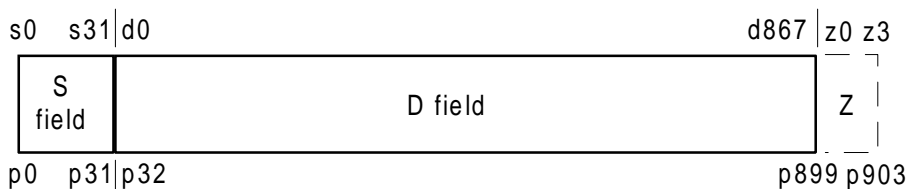
Figure 15: Packet P80
