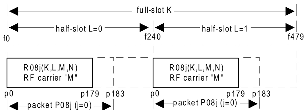
Figure 10: Low rate physical channel R08j for j = 0.
