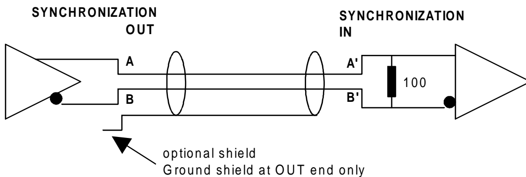
Figure C.1: Interconnection of synchronized devices
