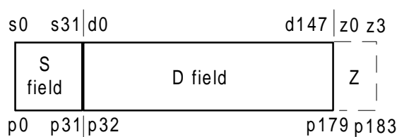
Figure 14: Packet P08j for j = 0
