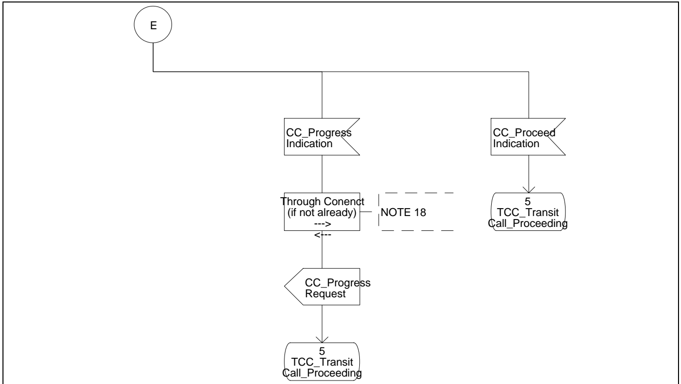
Figure 11 - Transit Call Control SDL Diagram (Part 10)
