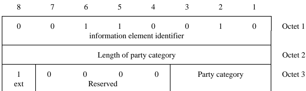
Figure 34 - Party category information element
