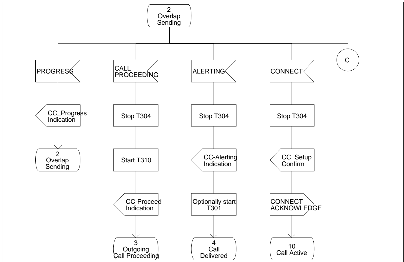
Figure 8 - Protocol Control SDL (Part 5)
