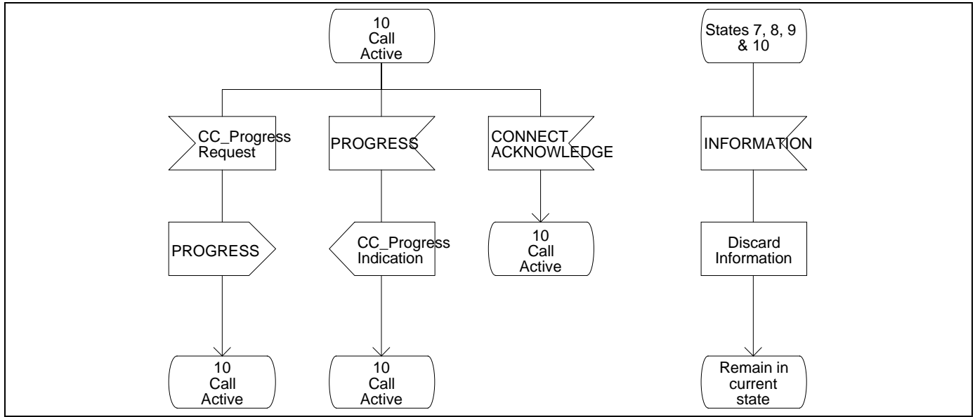
Figure 8 - Protocol Control SDL (Part 11)
