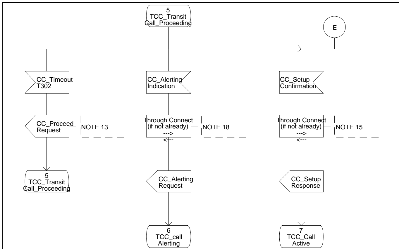
Figure 11 - Transit Call Control SDL Diagram (Part 9)
