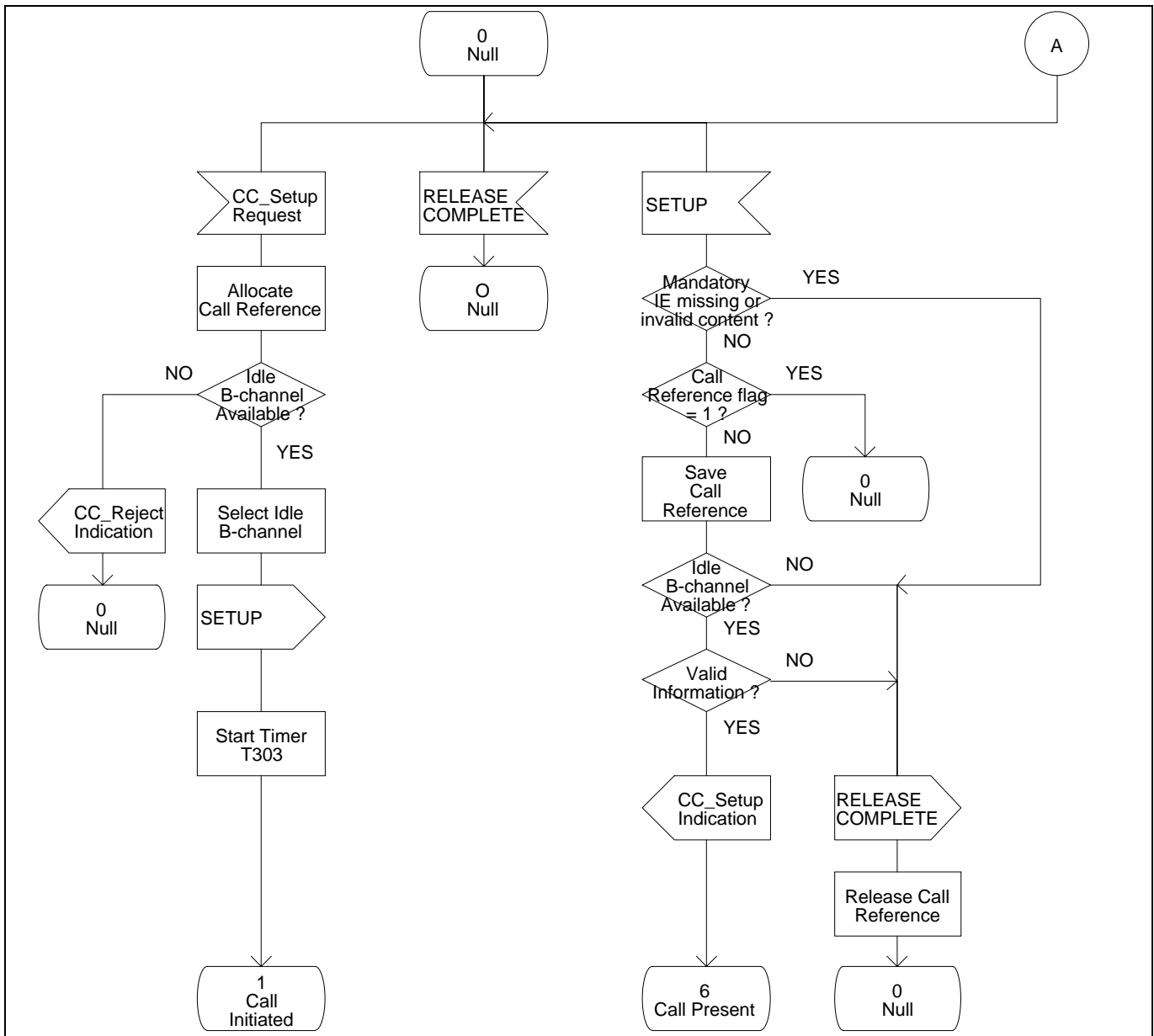
Figure 8 - Protocol Control SDL Diagram (Part 1)
