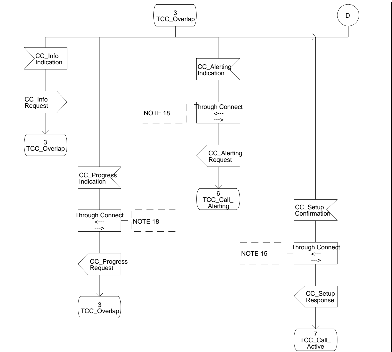
Figure 11 - Transit Call Control SDL Diagram (Part 6)
