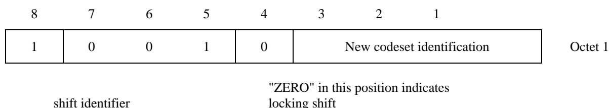
Figure 20 - Locking Shift Element
