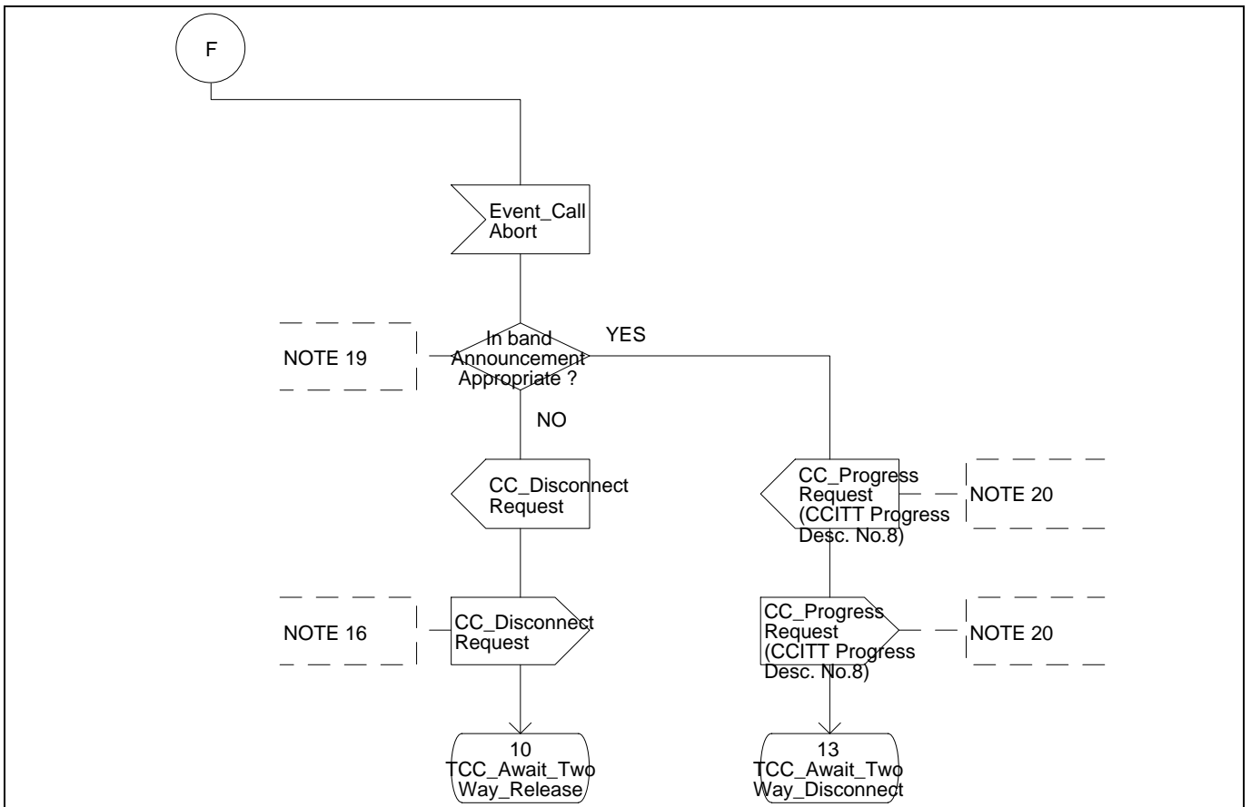
Figure 11 - Transit Call Control SDL Diagram (Part 14)
