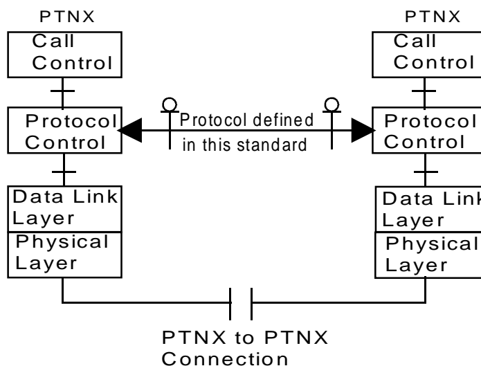
Figure 3 - Control Plane Protocol Model
