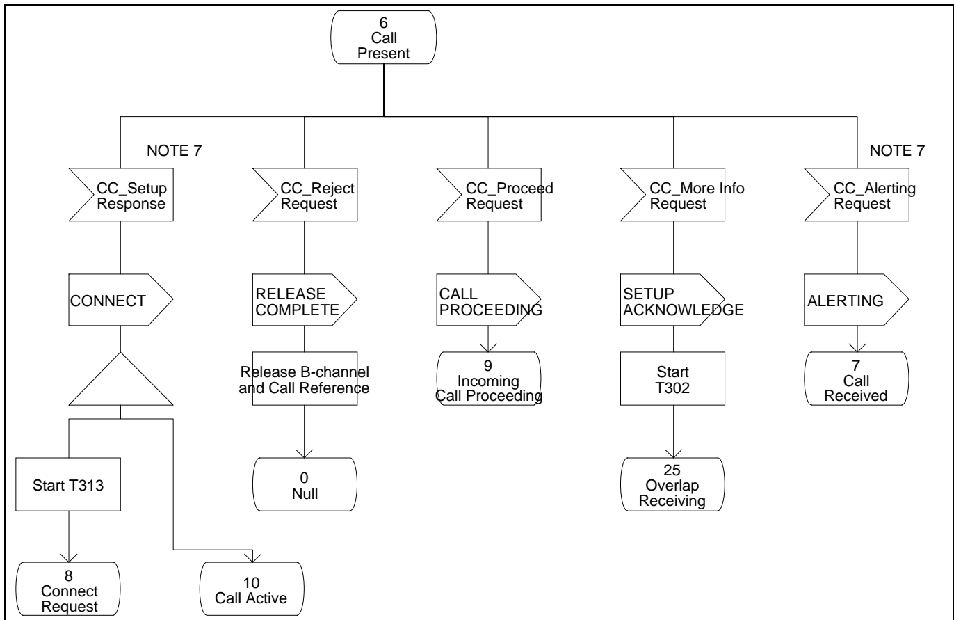
Figure 8 - Protocol Control SDL (Part 9)
