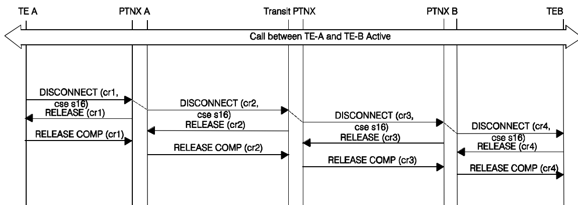
Figure B.5 - Normal Call Clearing by Originator
