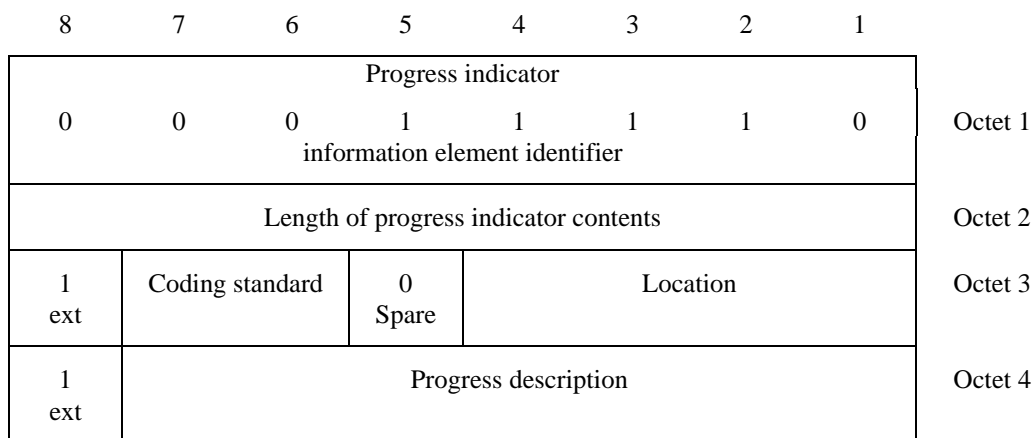
Figure 30 - Progress indicator information element
