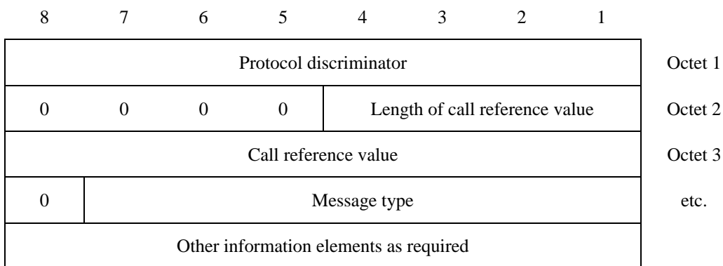
Figure 12 - General Message Organisation Example
