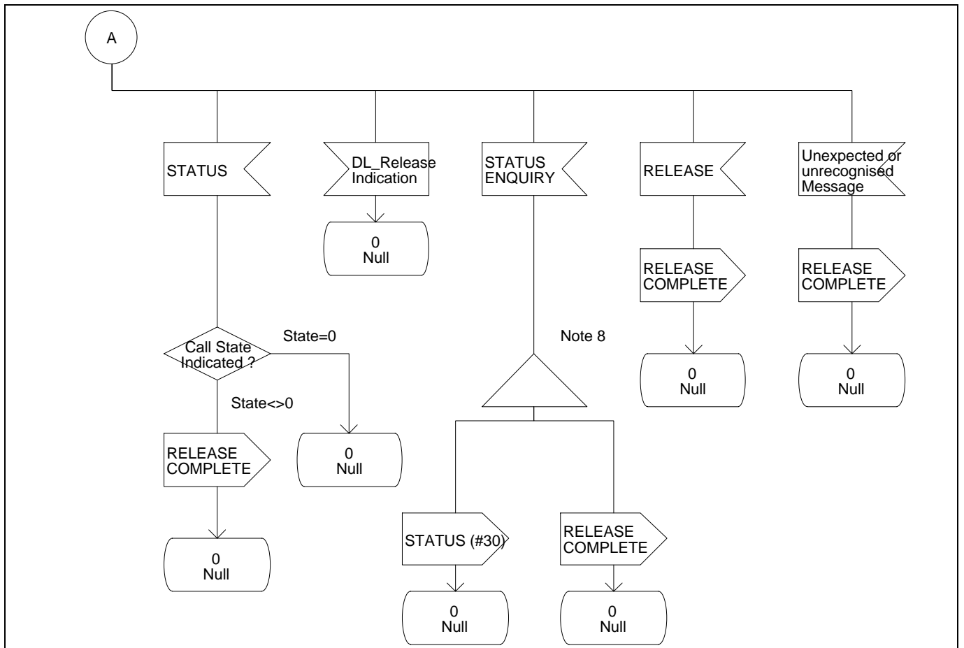
Figure 8 - Protocol Control SDL (Part 2)
