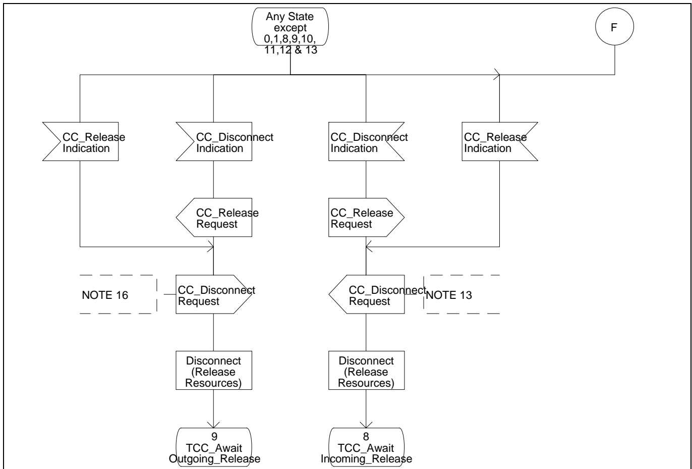
Figure 11 - Transit Call Control SDL Diagram (Part 13)
