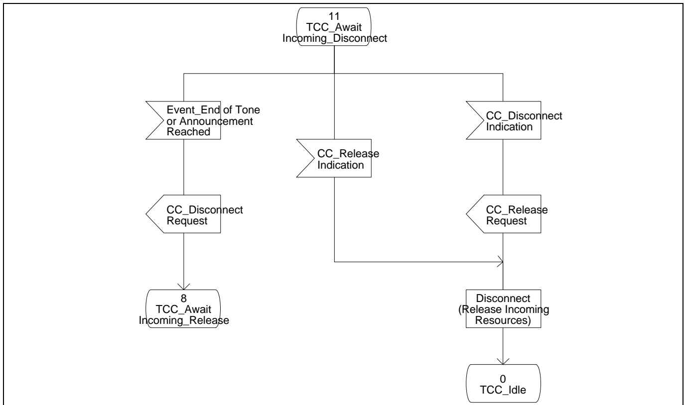
Figure 11 - Transit Call Control SDL Diagram (Part 15)
