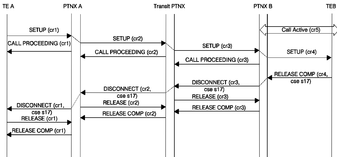
Figure B.2 - Enbloc Setup, Unsuccessful Call
