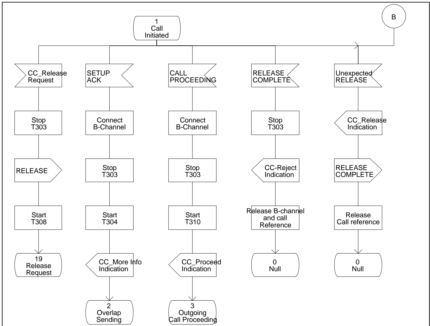
Figure 8 - Protocol Control SDL (Part 3)
