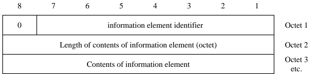
Figure 19 - Variable Length information element Format
