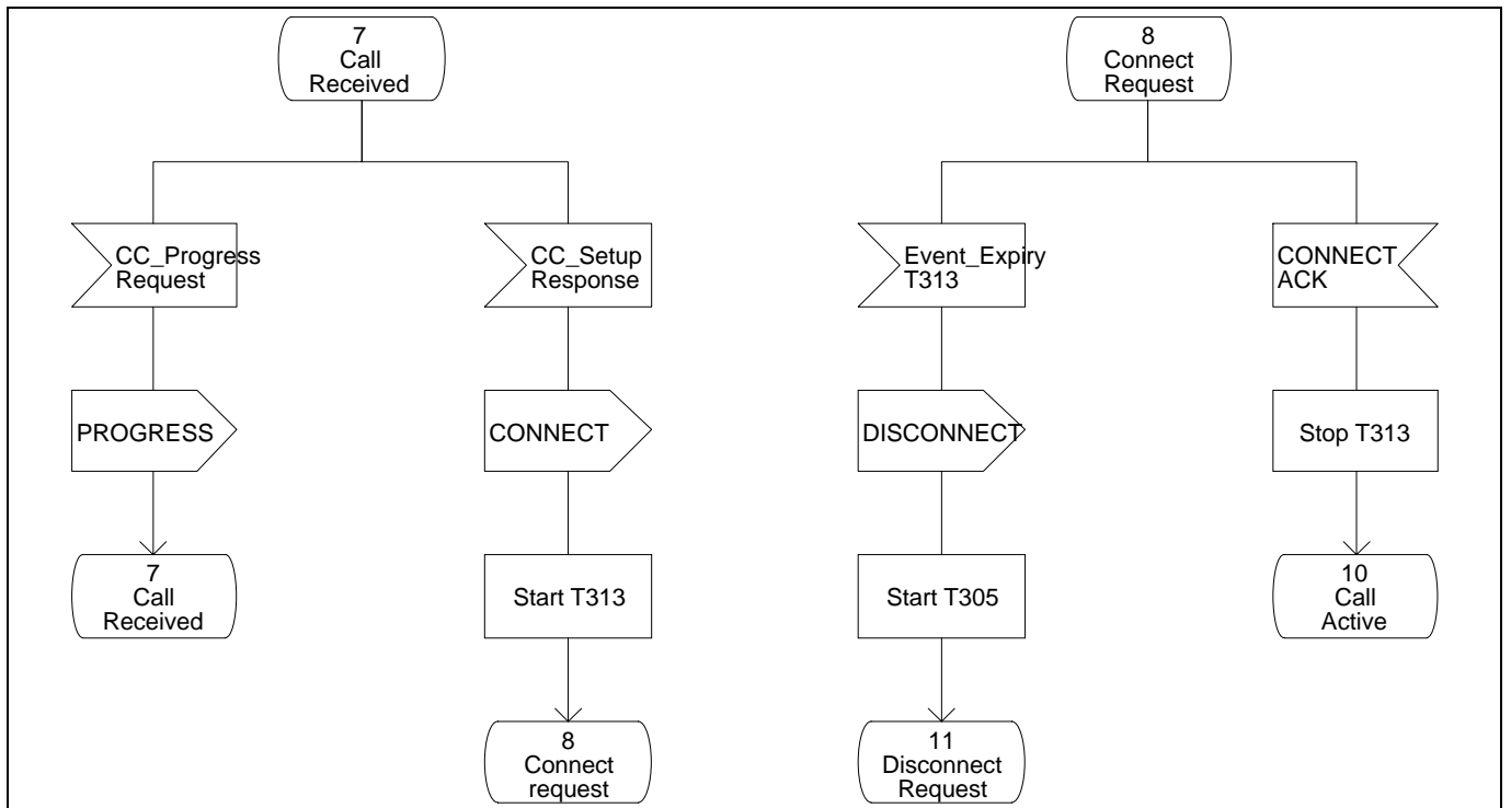
Figure 8 - Protocol Control SDL (Part 10)
