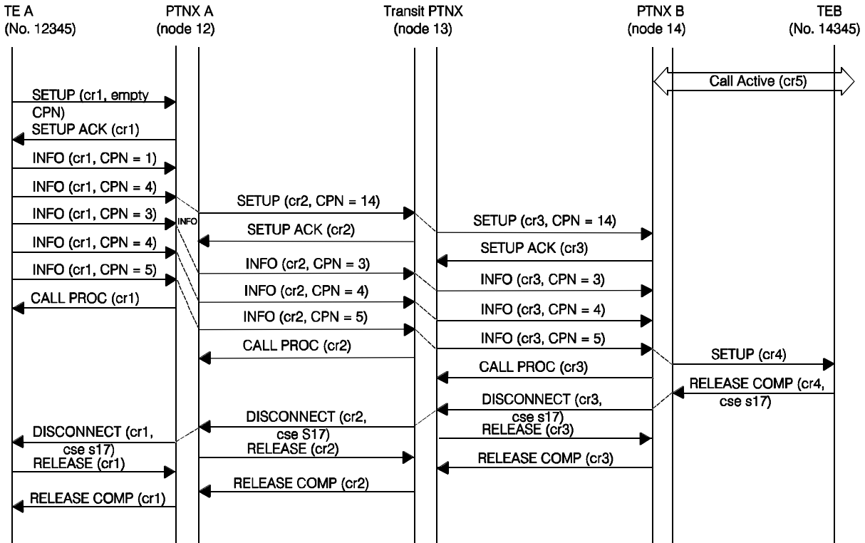
Figure B.4 - Overlap Setup, Unsuccessful Call
