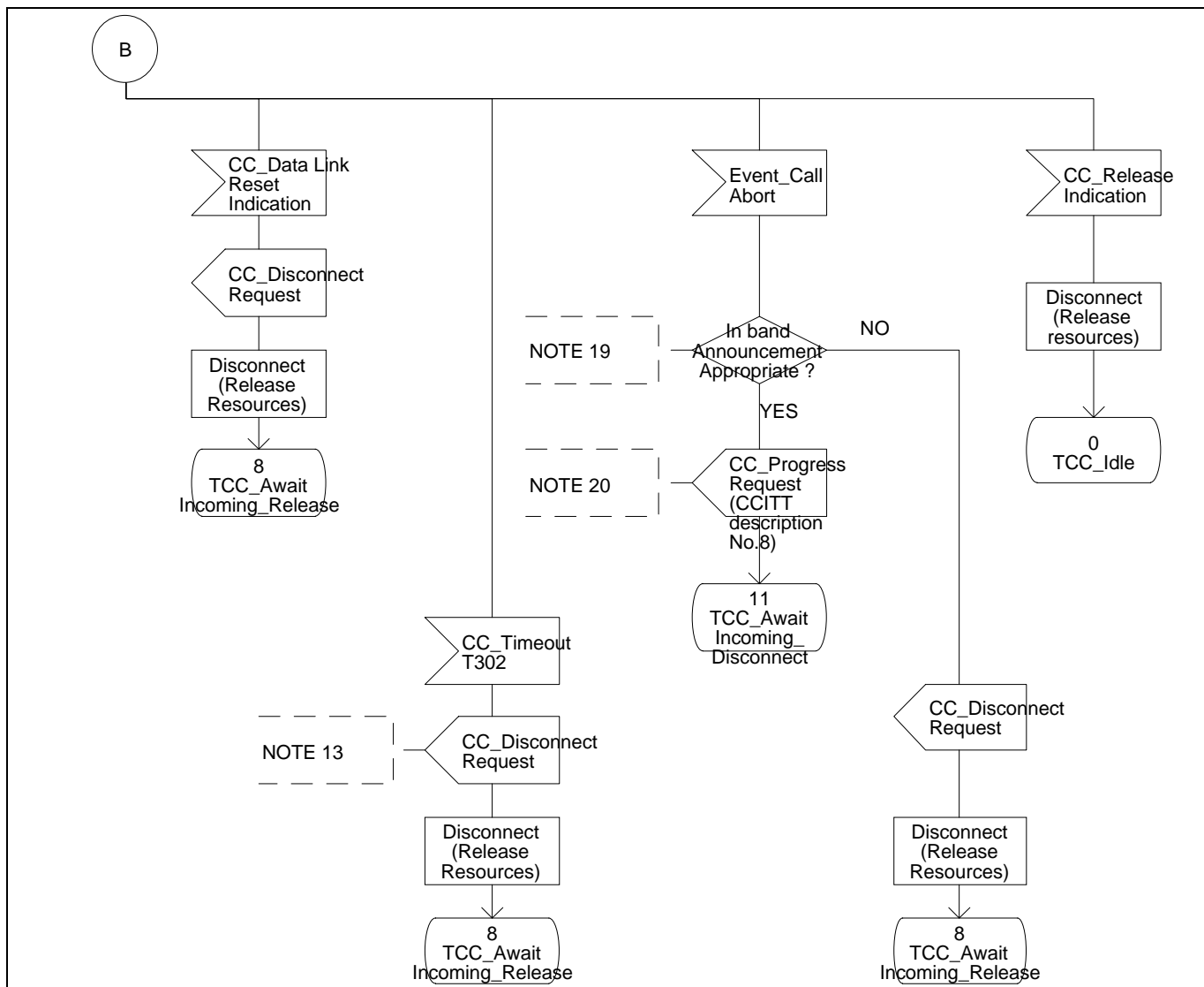
Figure 11 - Transit Call Control SDL Diagram (Part 3)
