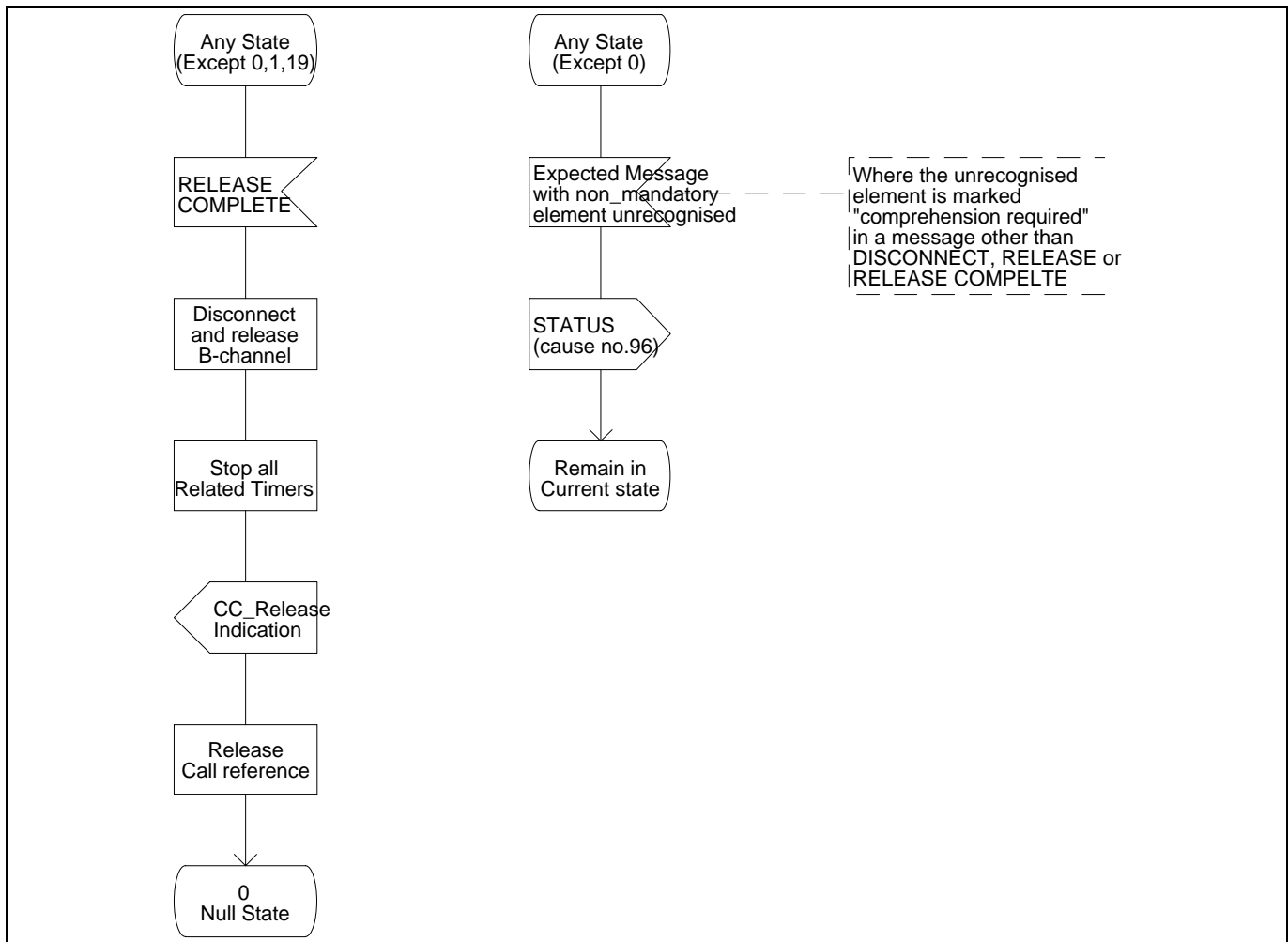
Figure 8 - Protocol Control SDL (Part 19)
