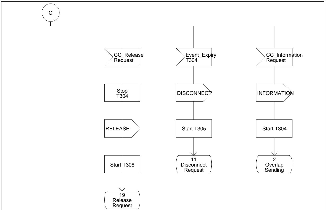
Figure 8 - Protocol Control SDL (Part 6)
