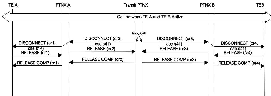
Figure B.6 - Call Abort by Transit PTNX
