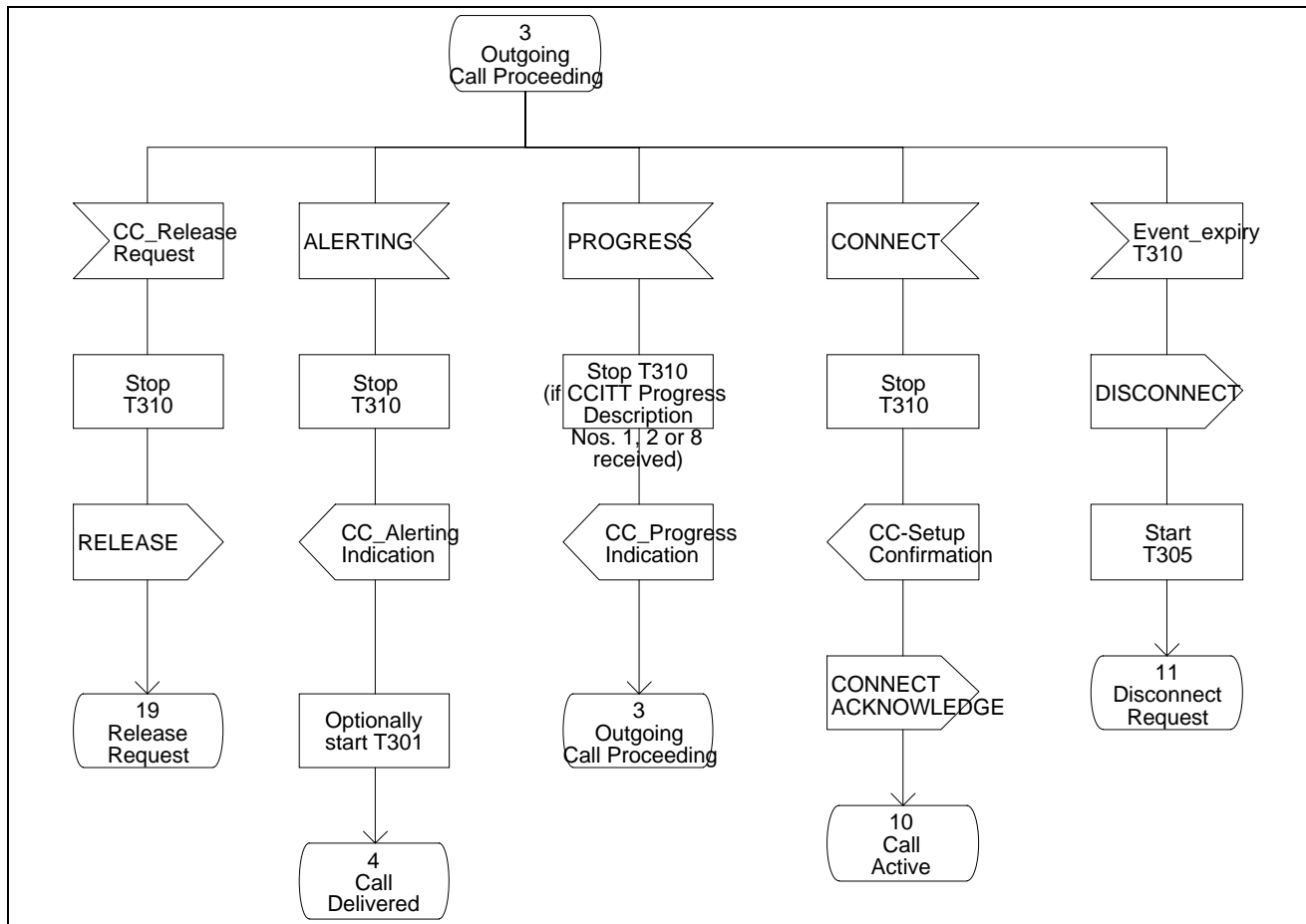
Figure 8 - Protocol Control SDL (Part 7)
