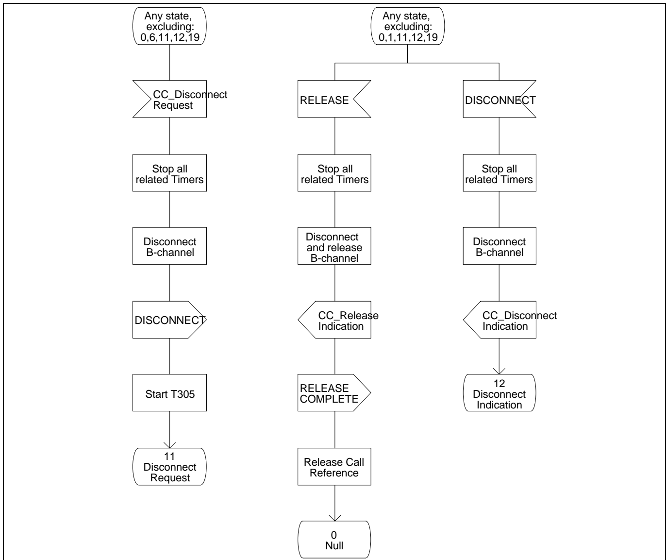
Figure 8 - Protocol Control SDL (Part 15)
