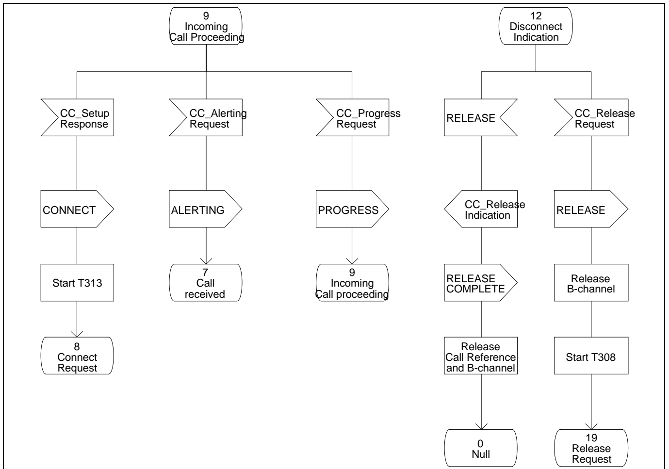
Figure 8 - Protocol Control SDL (Part 12)
