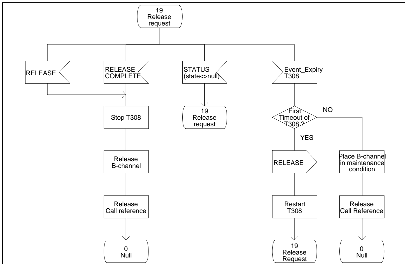
Figure 8 - Protocol Control SDL (Part 14)
