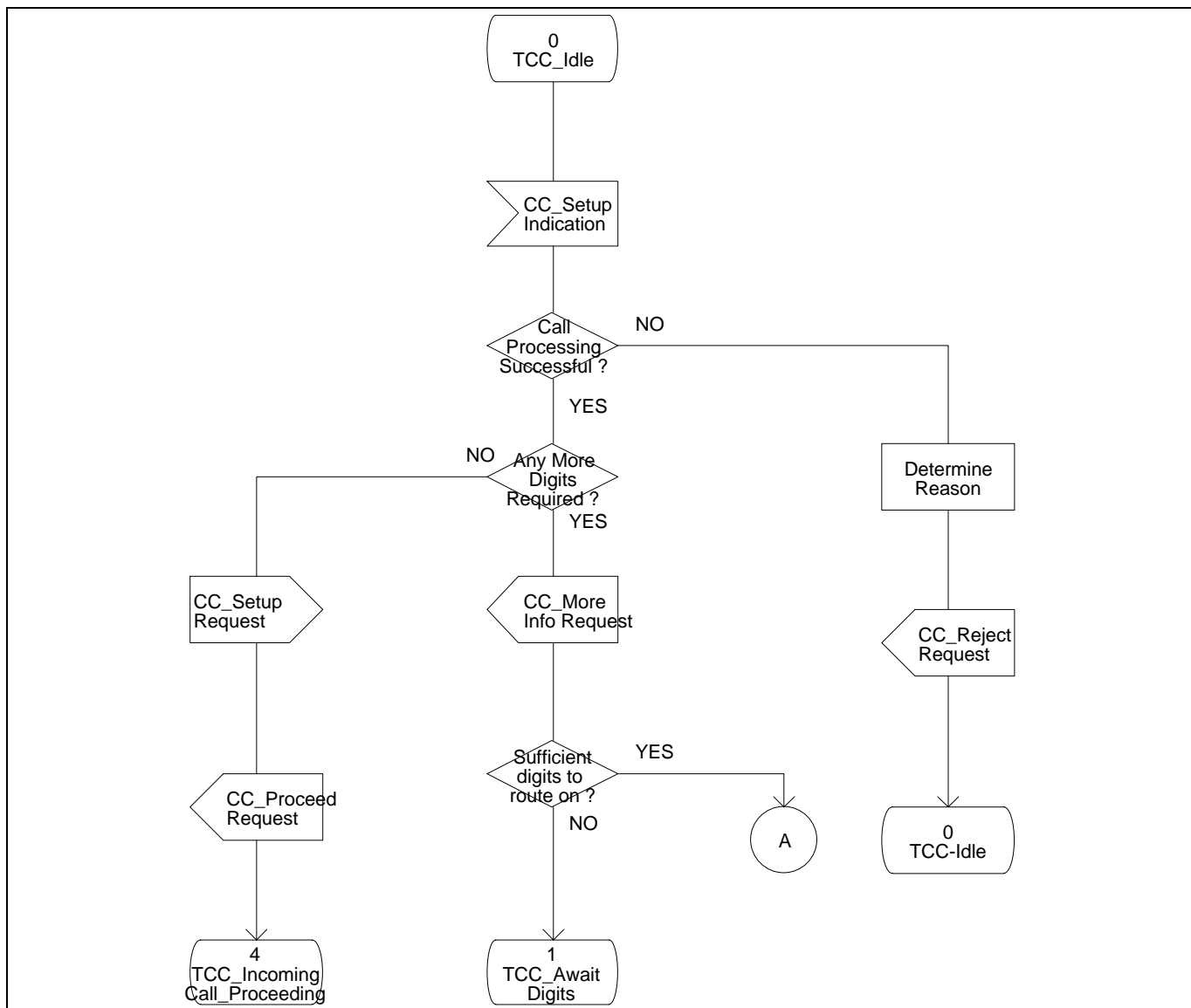
Figure 11 - Transit Call Control SDL Diagram (Part 1)
