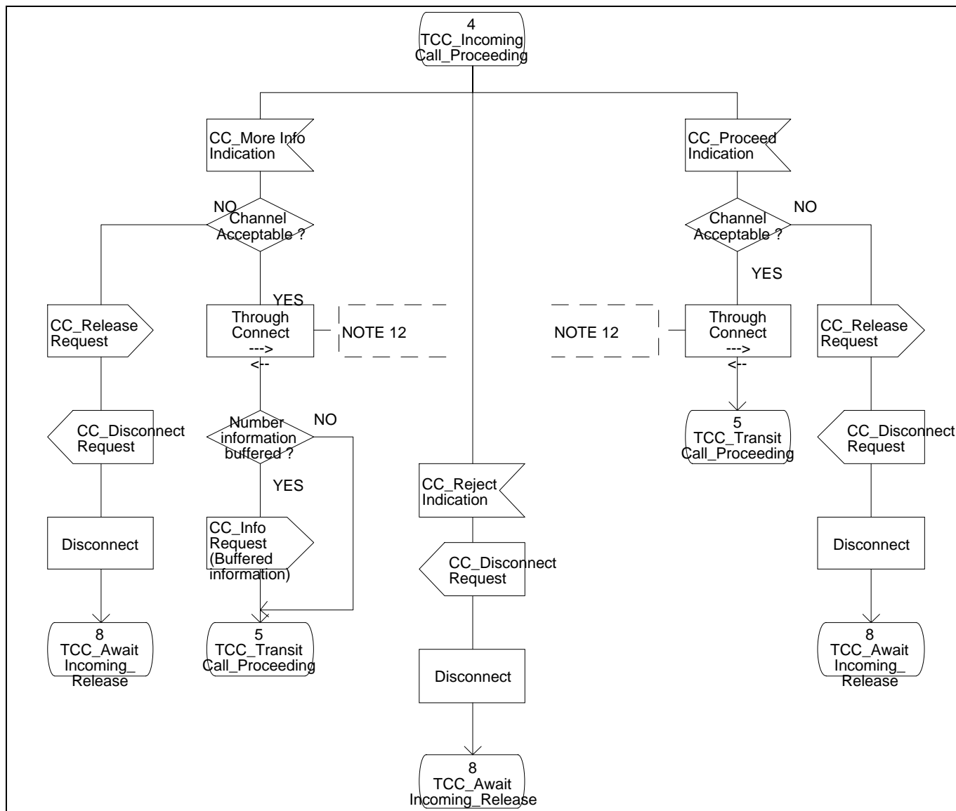
Figure 11 - Transit Call Control SDL Diagram (Part 8)
