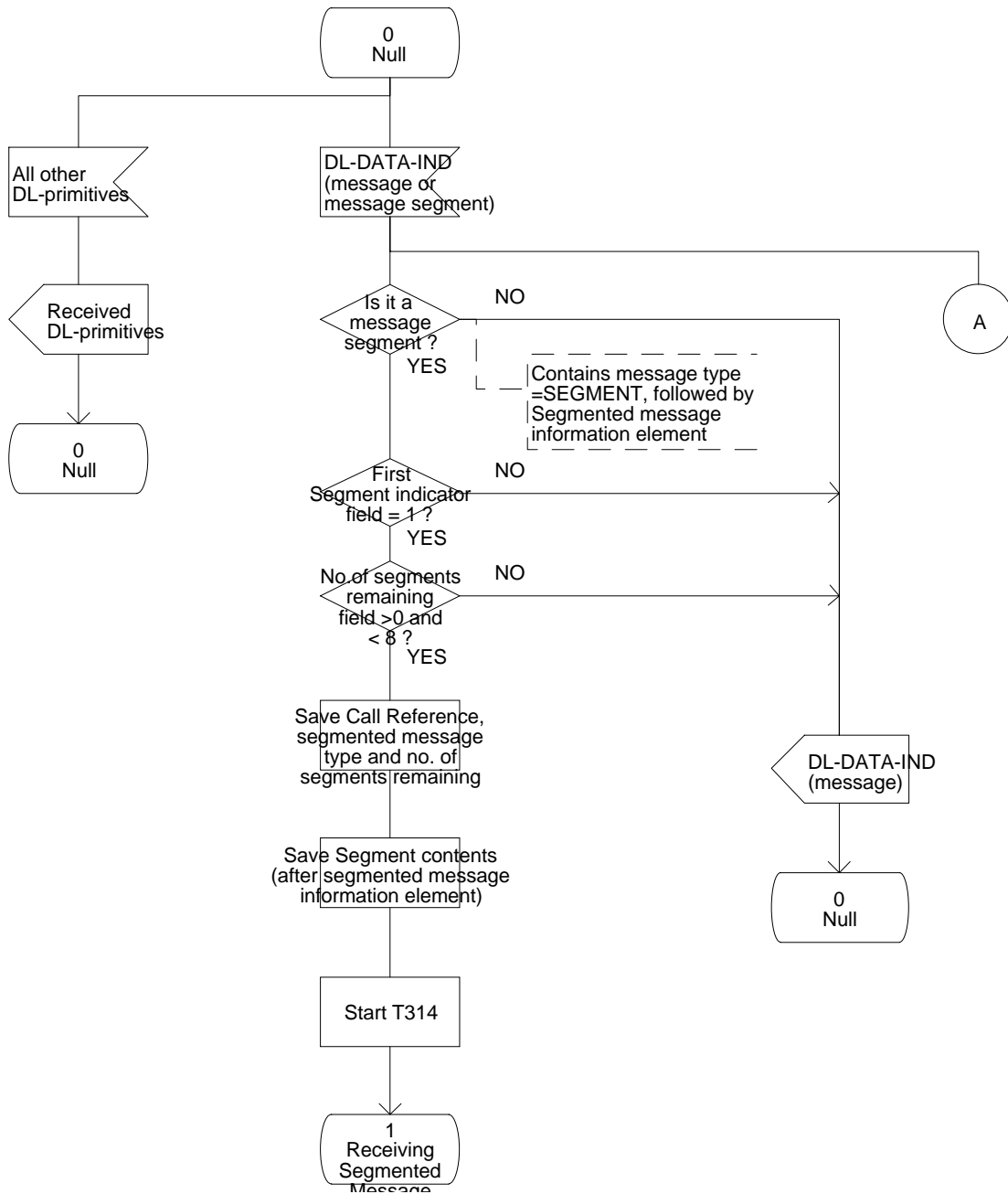
Figure 6 - Re-assembly Process SDL (Part 1)
