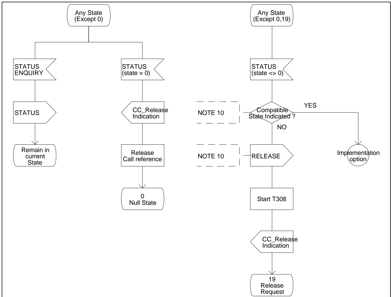
Figure 8 - Protocol Control SDL (Part 17)
