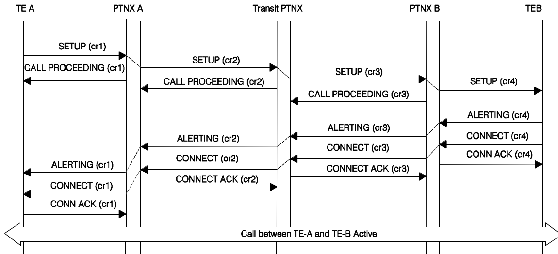
Figure B.1 - Enbloc Setup, Successful Call
