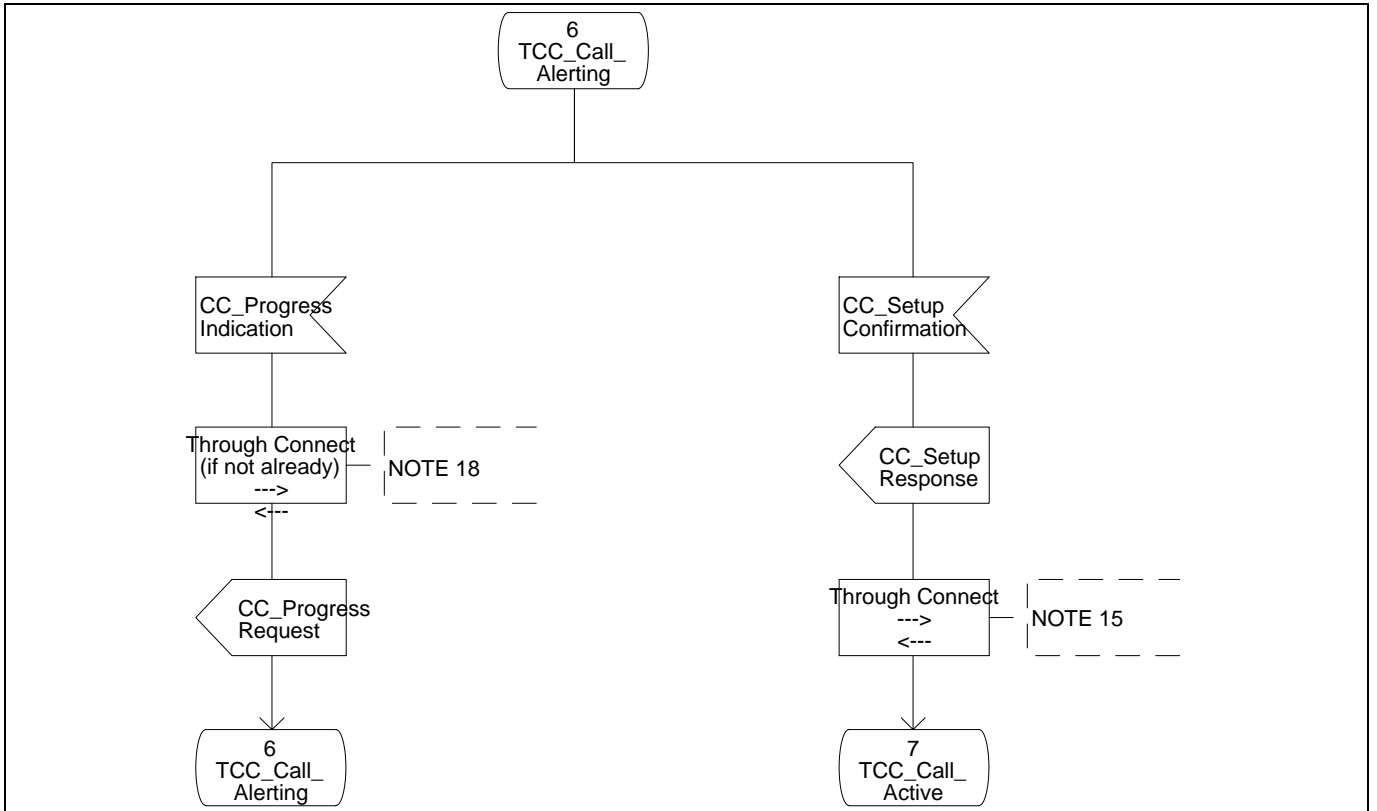
Figure 11 - Transit Call Control SDL Diagram (Part 11)
