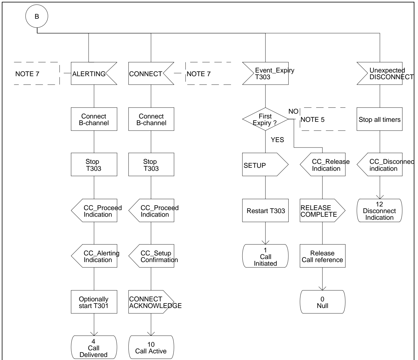
Figure 8 - Protocol Control SDL (Part 4)
