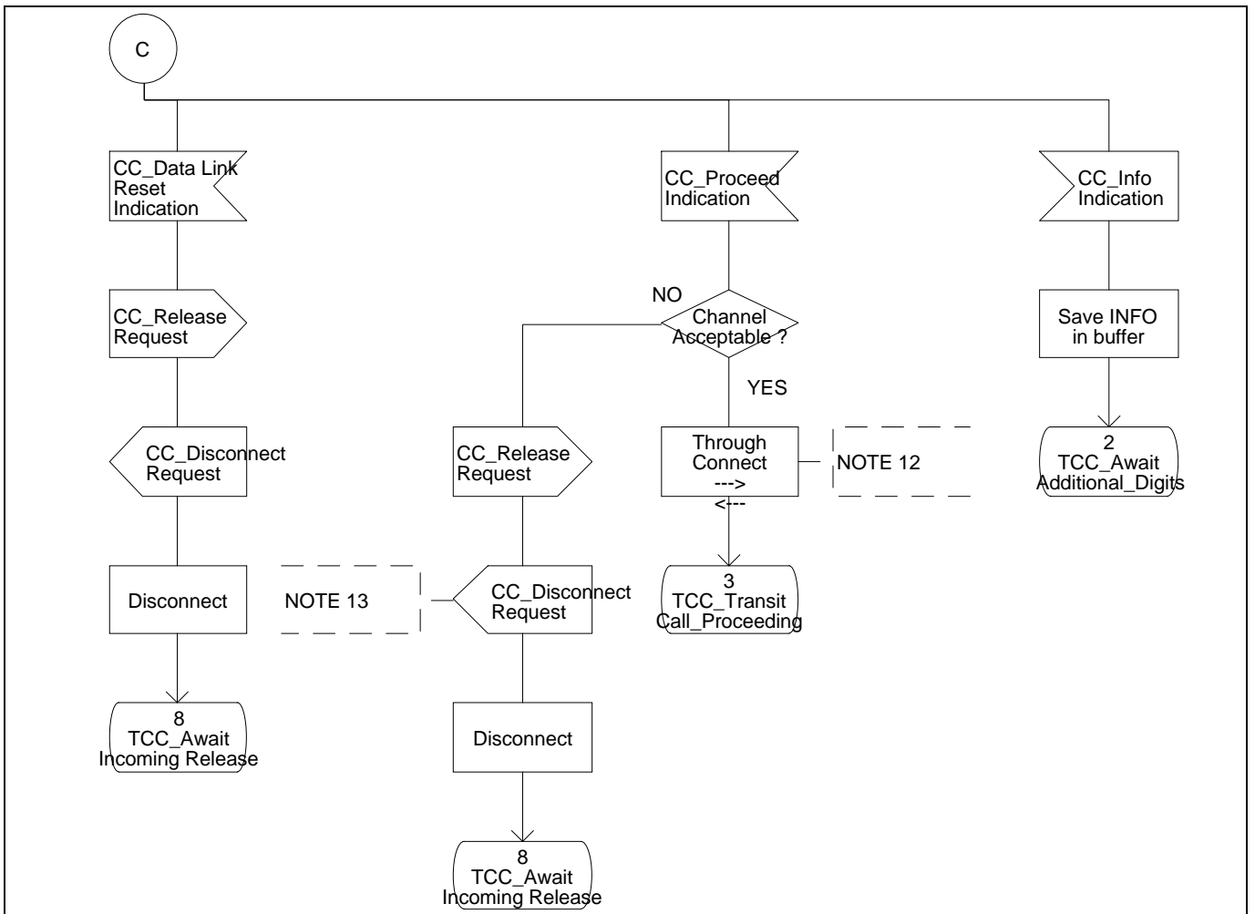
Figure 11 - Transit Call Control SDL Diagram (Part 5)
