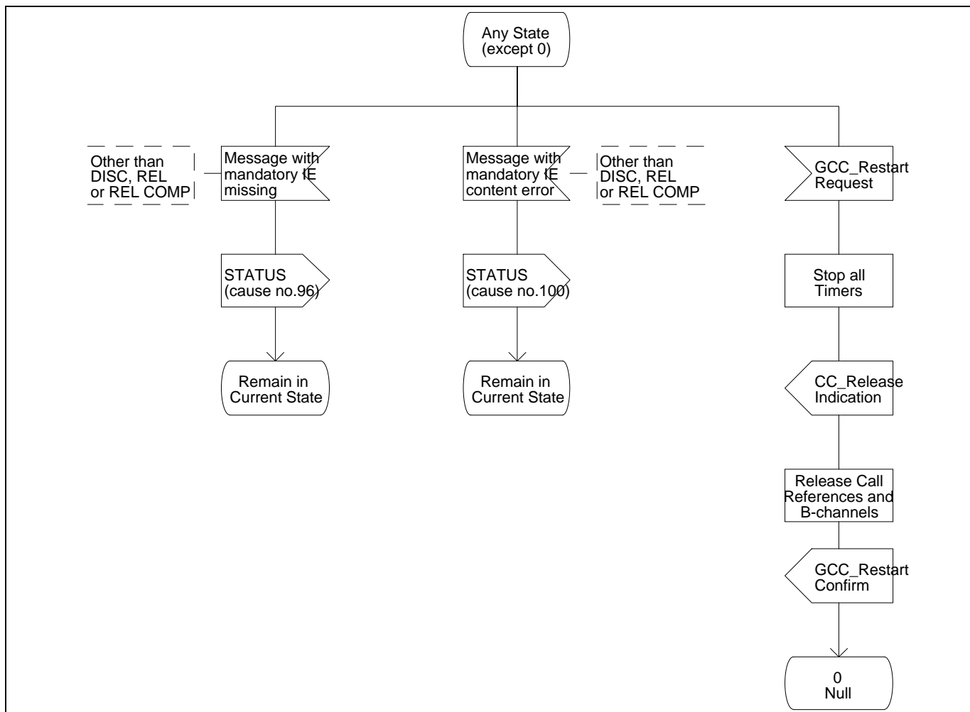
Figure 8 - Protocol Control SDL (Part 20)
