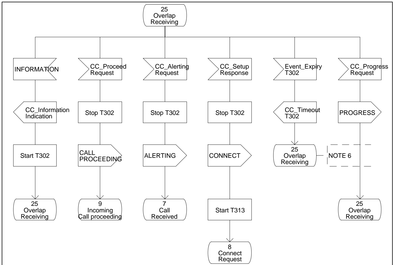
Figure 8 - Protocol Control SDL (Part 16)
