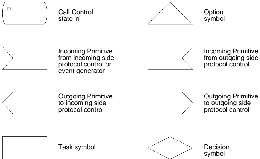
Figure 10 - Key to Transit Call Control SDL Diagram
