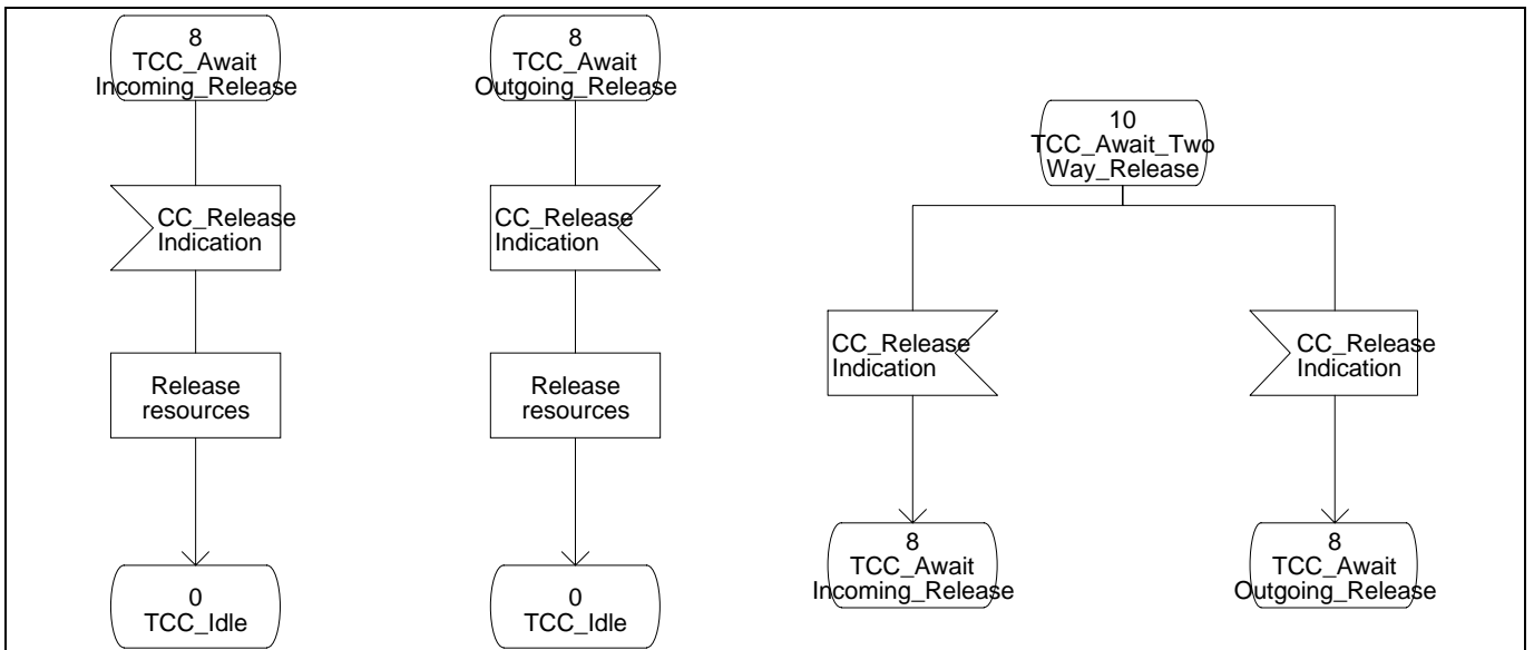
Figure 11 - Transit Call Control SDL Diagram (Part 12)
