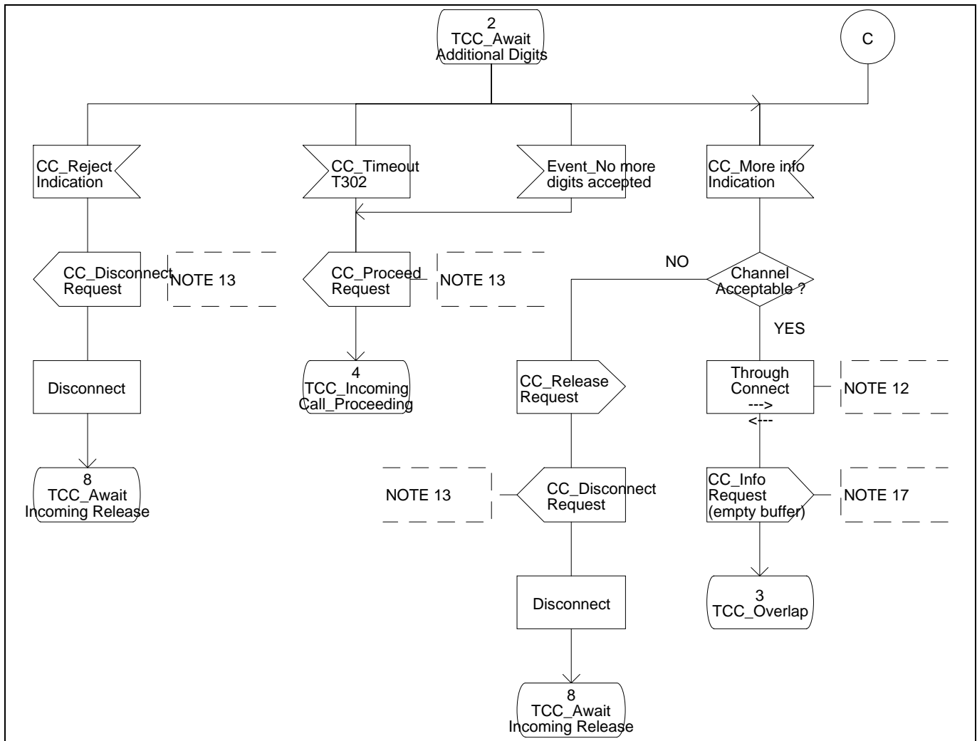
Figure 11 - Transit Call Control SDL Diagram (Part 4)
