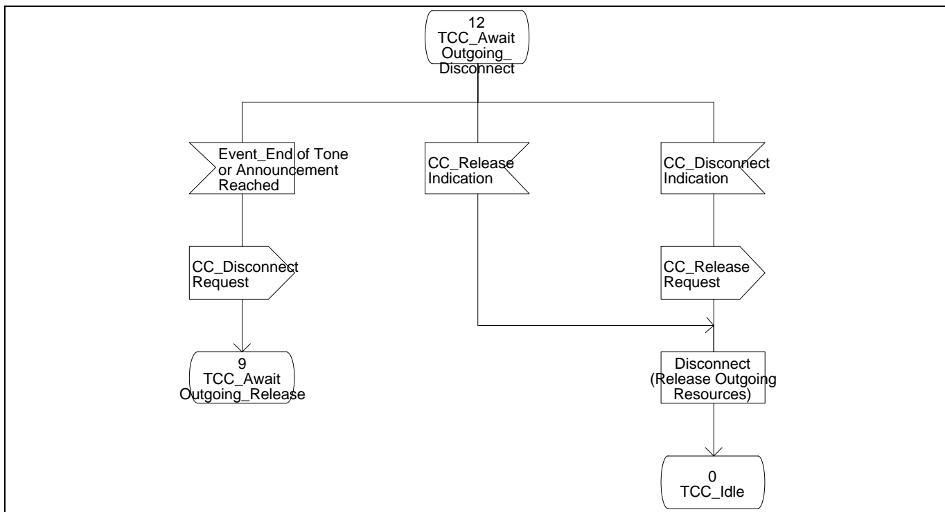
Figure 11 - Transit Call Control SDL Diagram (Part 16)
