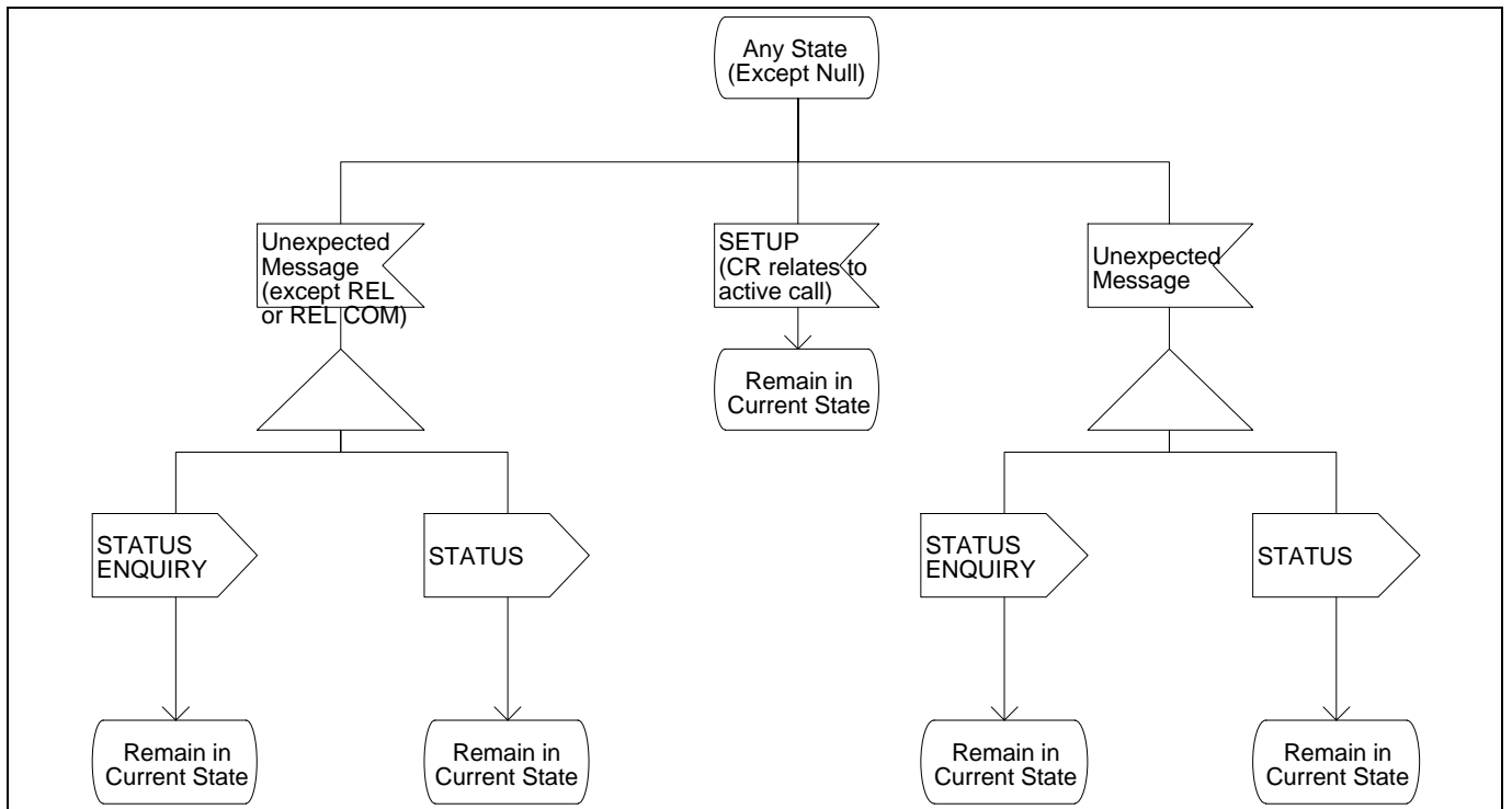
Figure 8 - Protocol Control SDL (Part 18)
