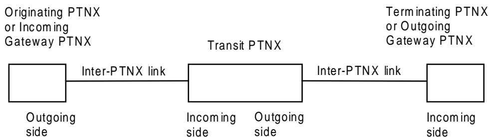
Figure 1 - Illustration of Terminology through Example of a Call Routed over Two Inter-PTNX Links
