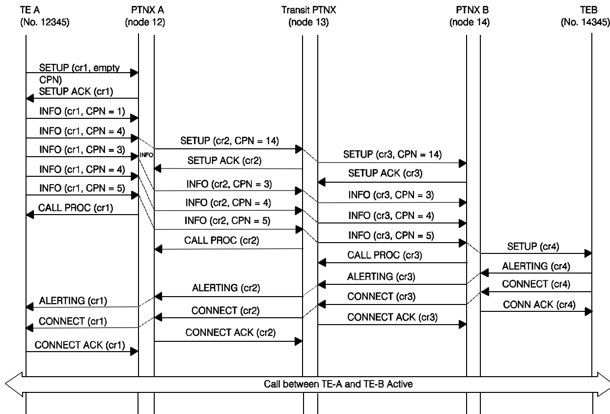
Figure B.3 - Overlap Setup, Successful Call
