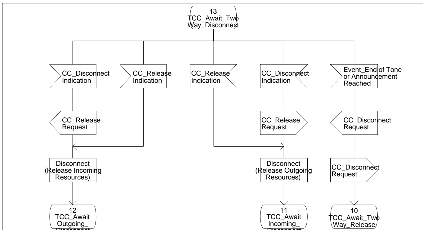
Figure 11 - Transit Call Control SDL Diagram (Part 17)
