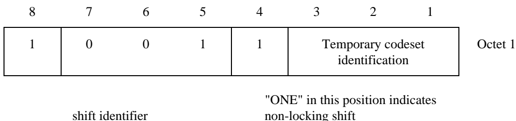
Figure 21 - Non-locking Shift Element
