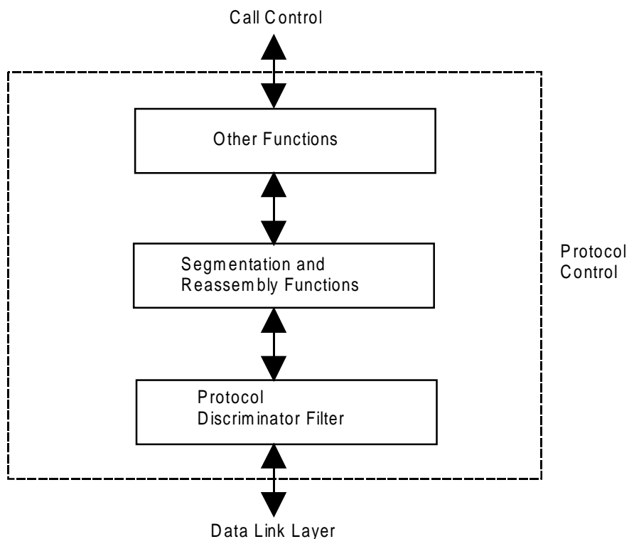
Figure 4 - Logical Architecture of Protocol Control Showing Segmentation and Re-assembly Functions
