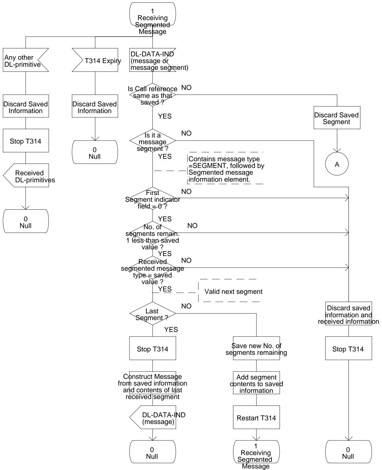
Figure 6 - Re-assembly Process SDL (Part 2)
