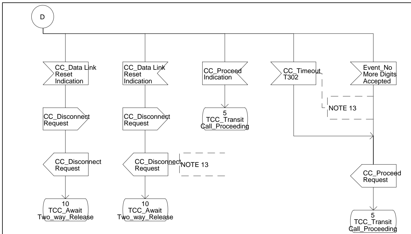
Figure 11 - Transit Call Control SDL Diagram (Part 7)
