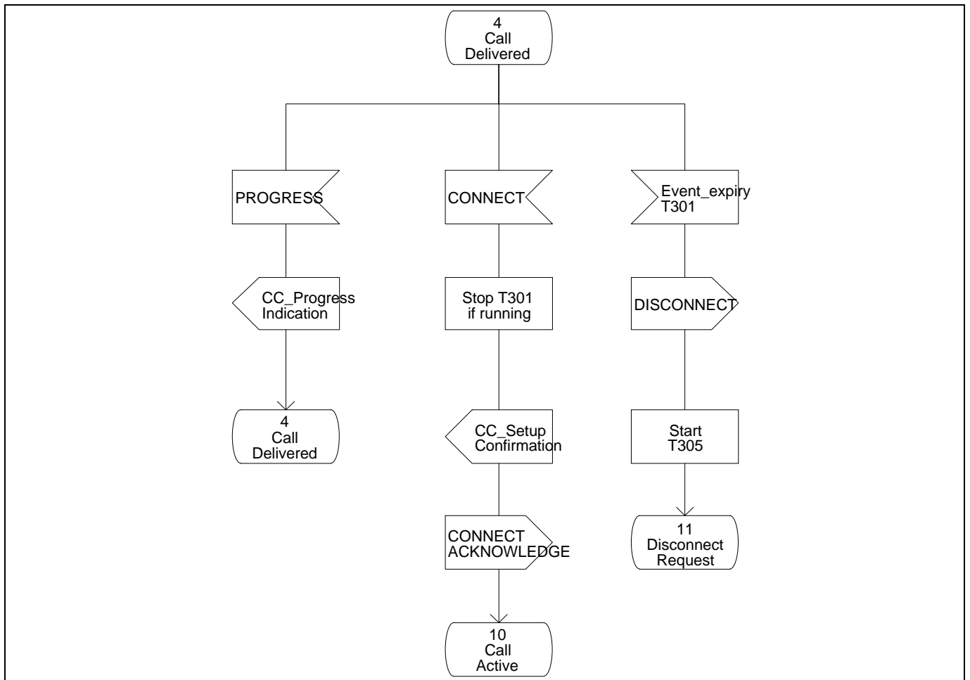
Figure 8 - Protocol Control SDL (Part 8)
