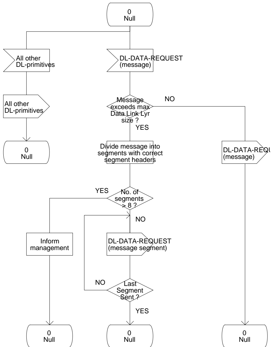
Figure 5 - Segmentation Process SDL
