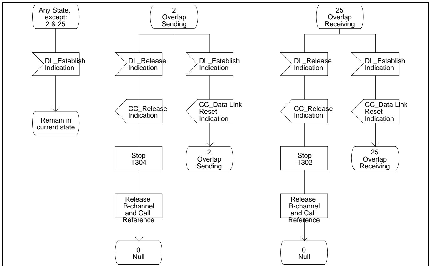
Figure 8 - Protocol Control SDL (Part 21)
