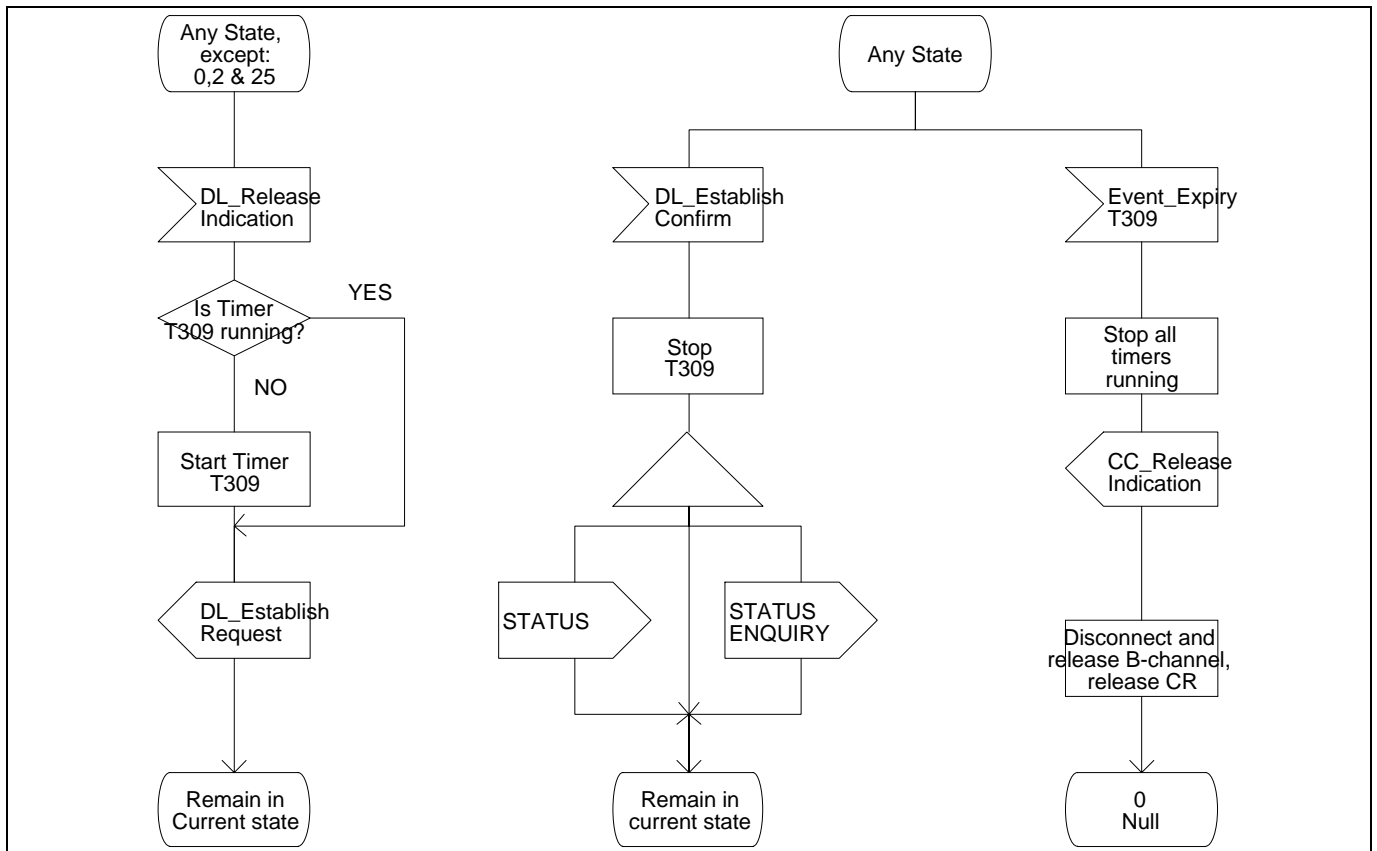
Figure 8 - Protocol Control SDL (Part 22)
