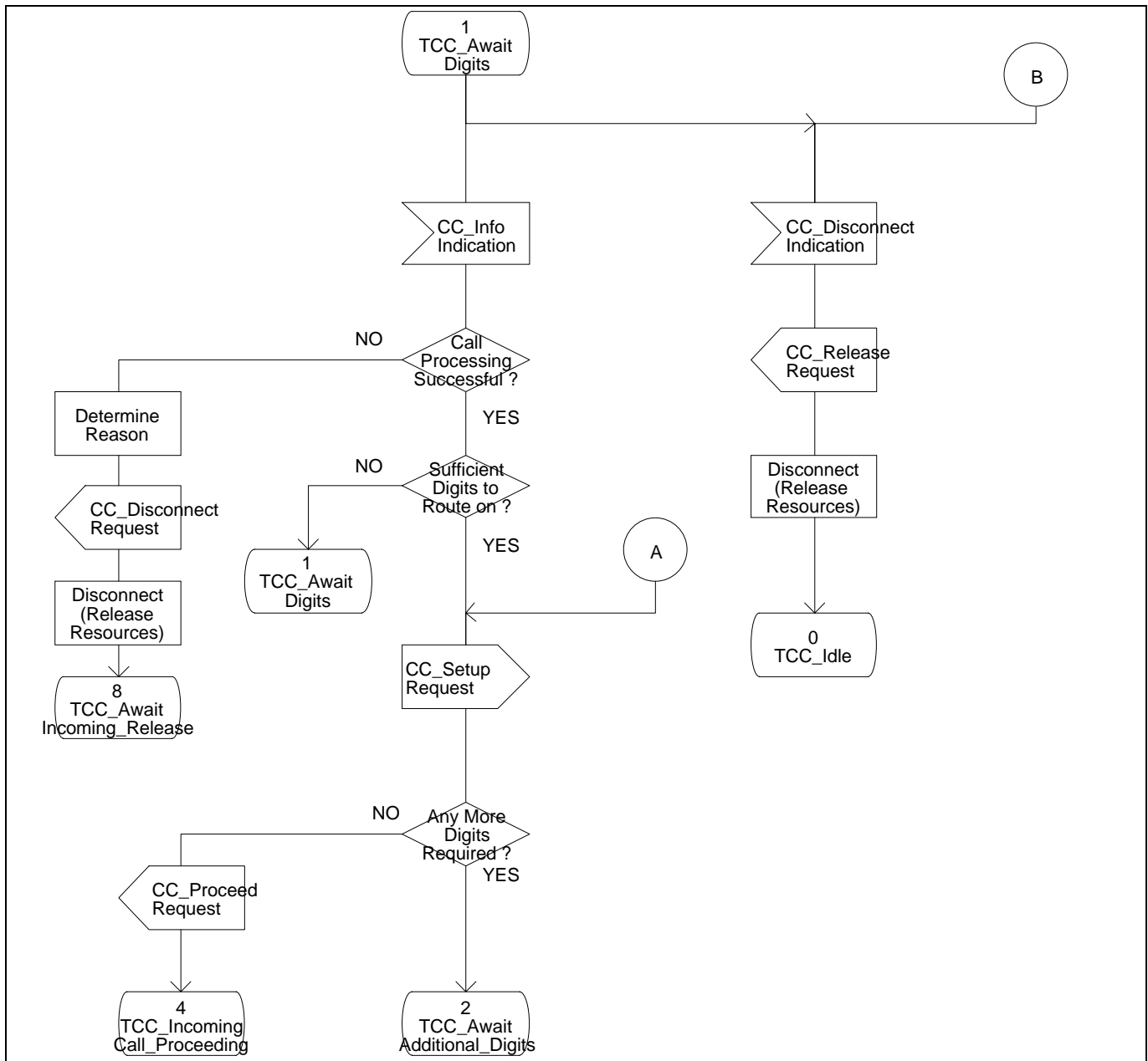
Figure 11 -Transit Call Control SDL Diagram (Part 2)
