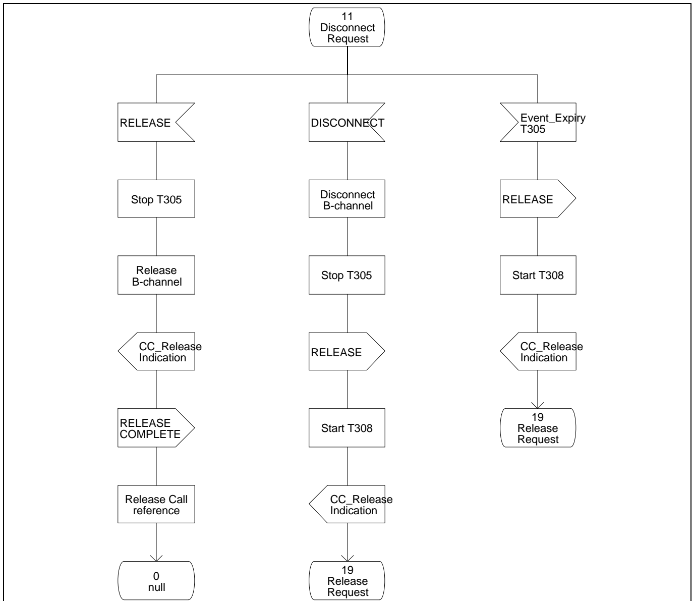
Figure 8 - Protocol Control SDL (Part 13)
