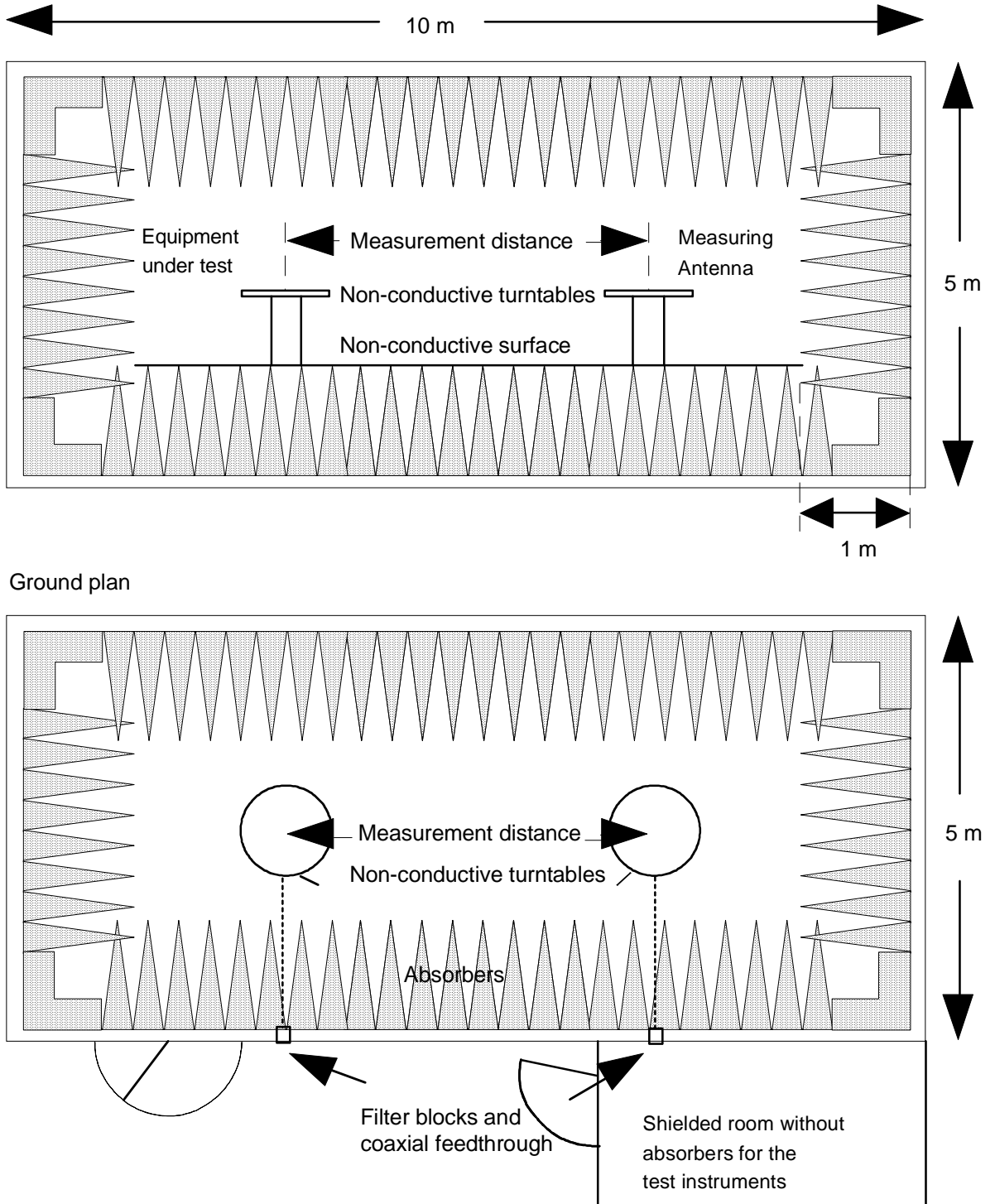
Figure E.4: Example of construction of an anechoic shielded chamber
