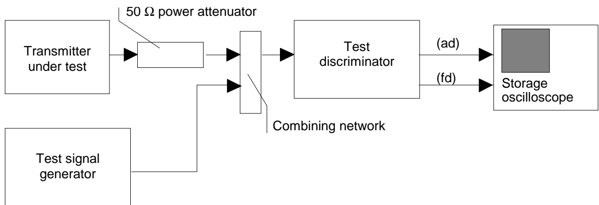
Figure 5: Measurement arrangement
