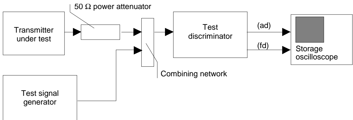
Figure 5: Measurement arrangement
