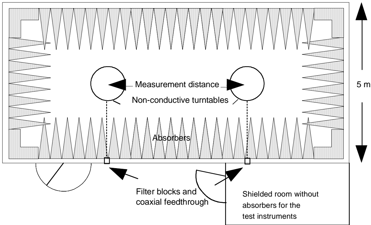
Figure E.4: Example of construction of an anechoic shielded chamber
