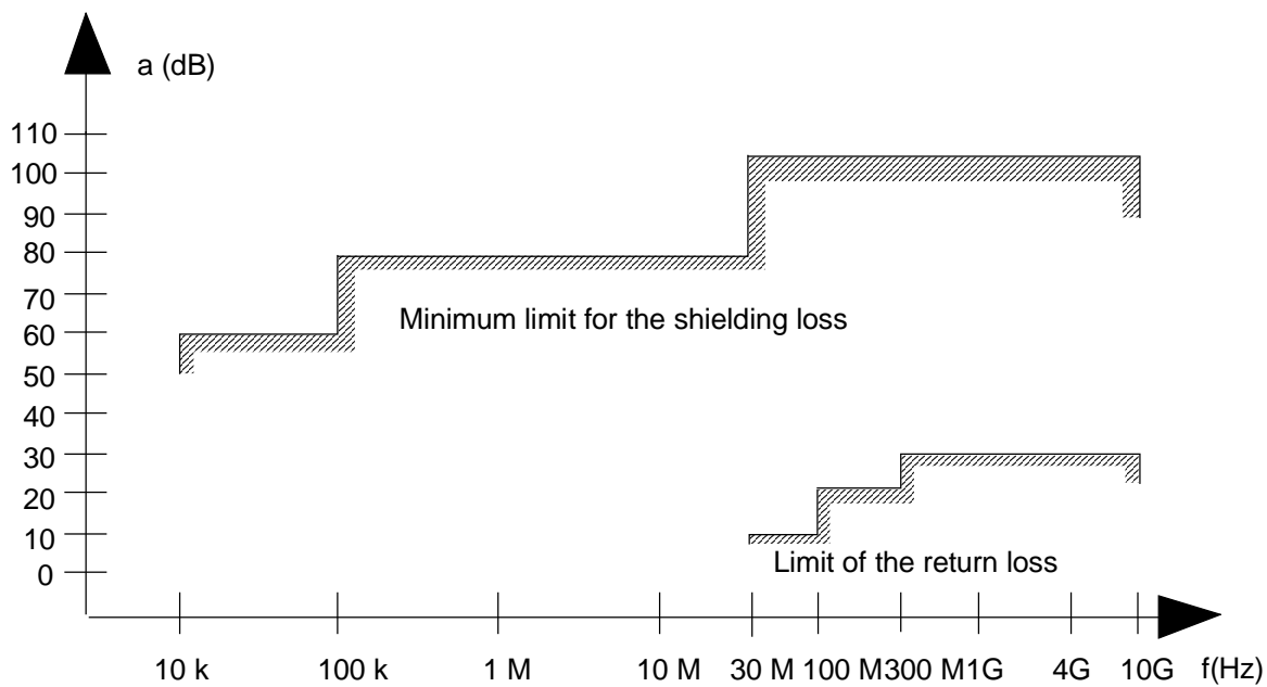
Figure E.3: Specifications for shielding and reflections
