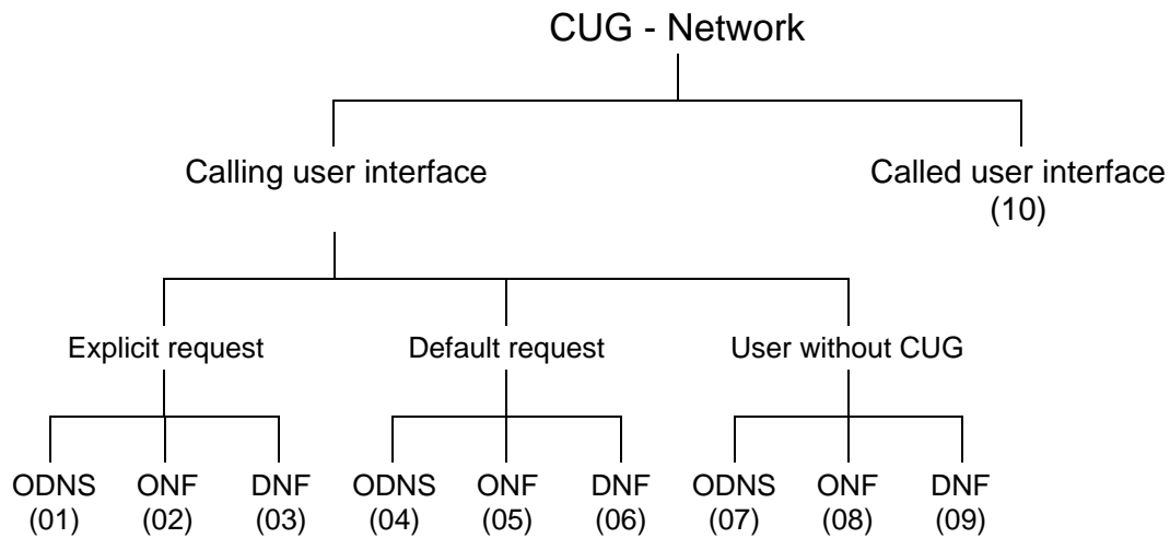
Figure 1: Test suite structure
