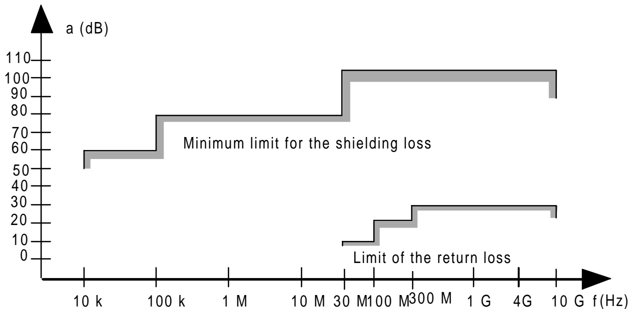
Figure A.3: Specifications for shielding and reflections
