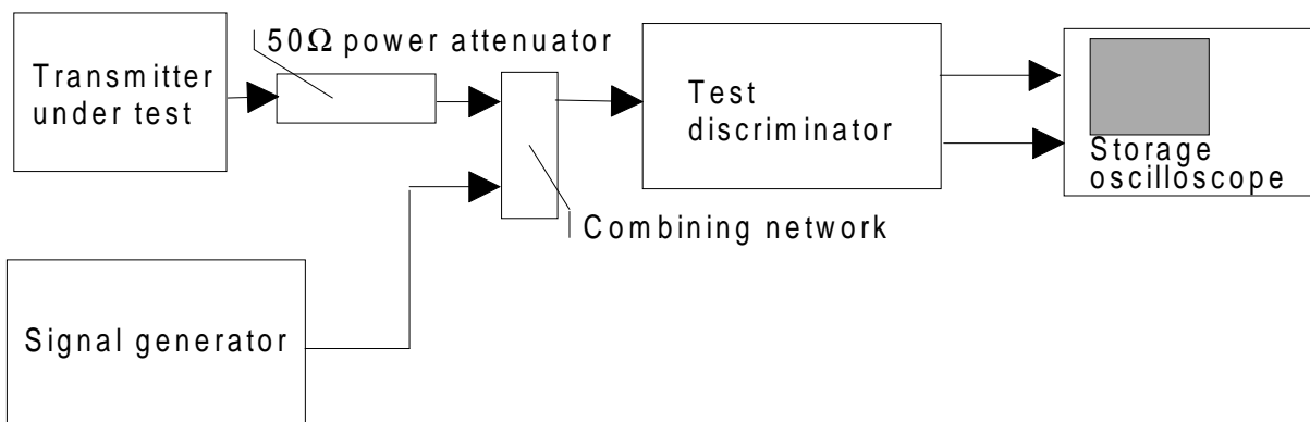
Figure 3: Measurement arrangement.
