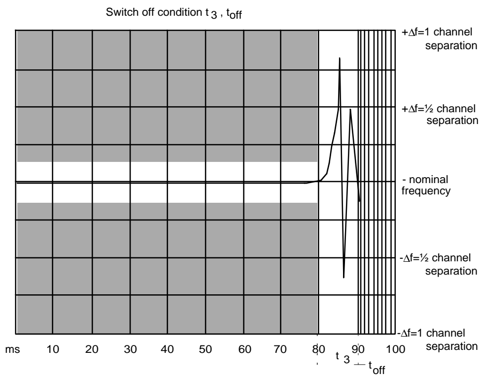
Figure 4: Storage oscilloscope view t_1 , t_2 and t_3
