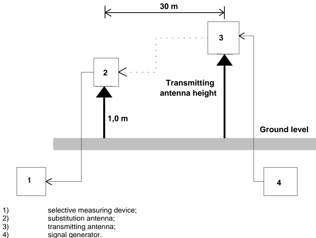
Figure B.3: Measurement arrangement for calibration of open air test site
