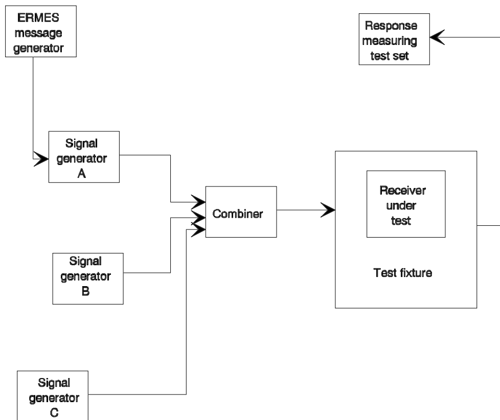
Figure A.2: Measurement arrangement (clause A.6)
