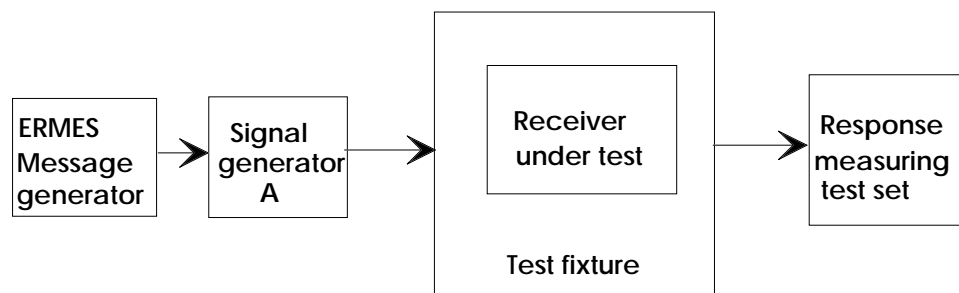
Figure B.1: Receiver in test fixture (see clause B.6)
