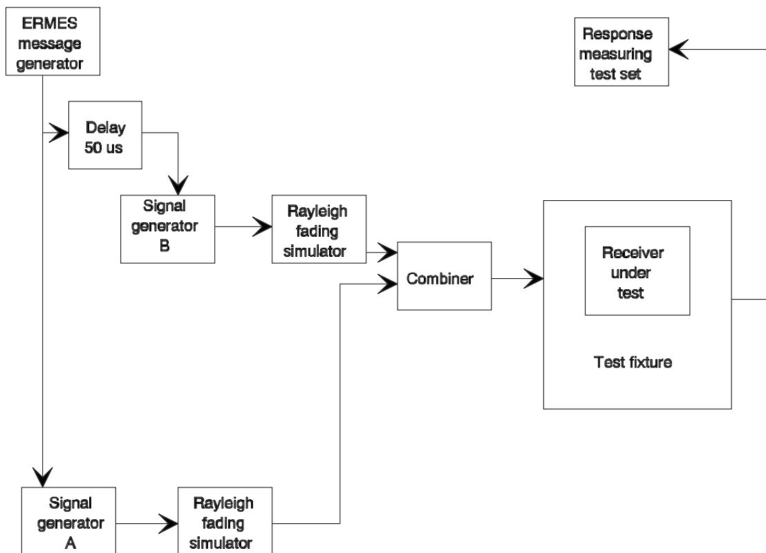
Figure A.3: Measurement set-up (clause A.8)
