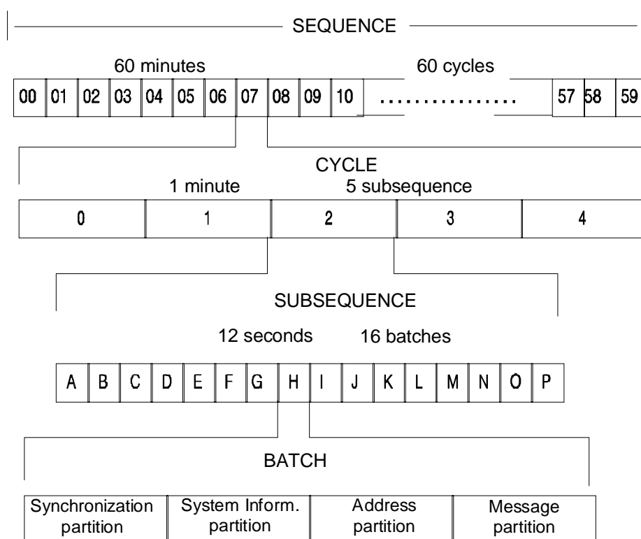
Figure 2: Structure of the radio protocol on channel one
