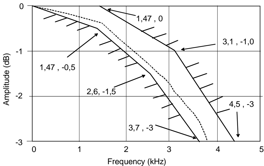
Figure 16(b): Detail expansion of above low pass filter characteristic
