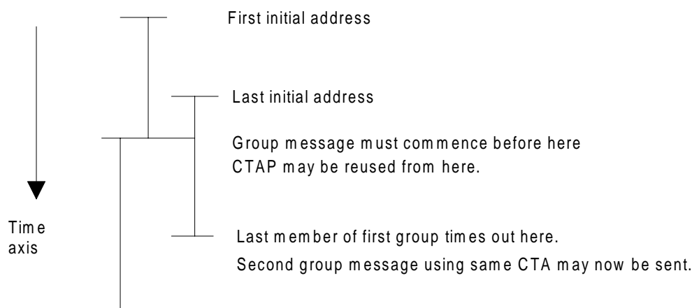
Figure 22: Time-out criteria for group calls
