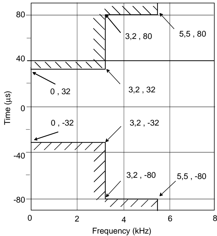
Figure 16(c): Group delay mask for the 4-PAM/FM premodulation filter
