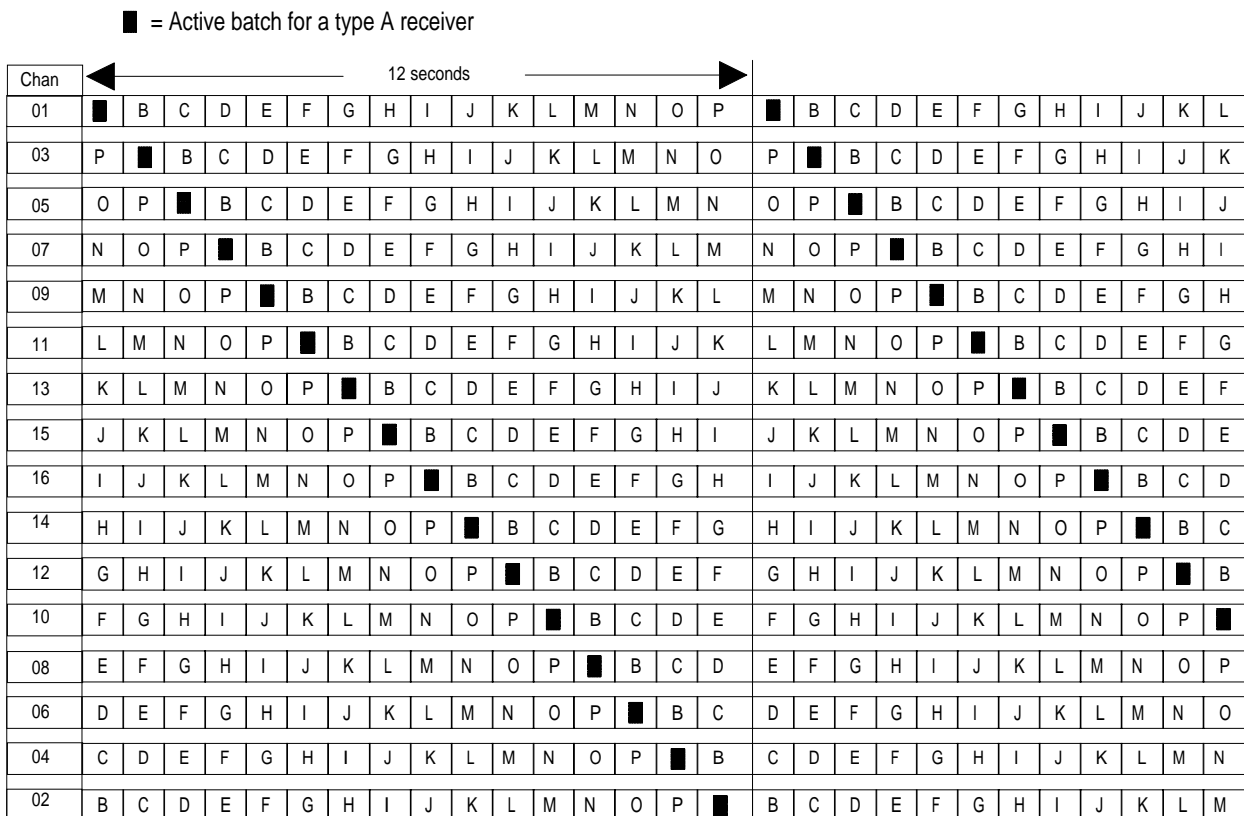
Figure 2: Structure of the radio protocol on channel one
