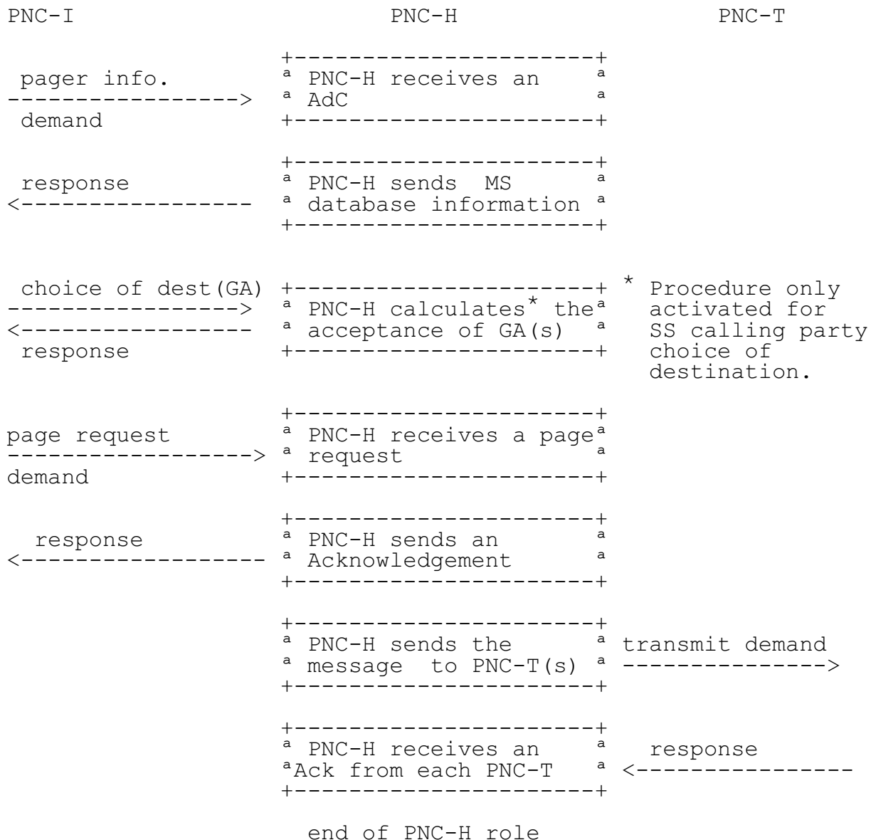
Figure 7: PNC-H processing
