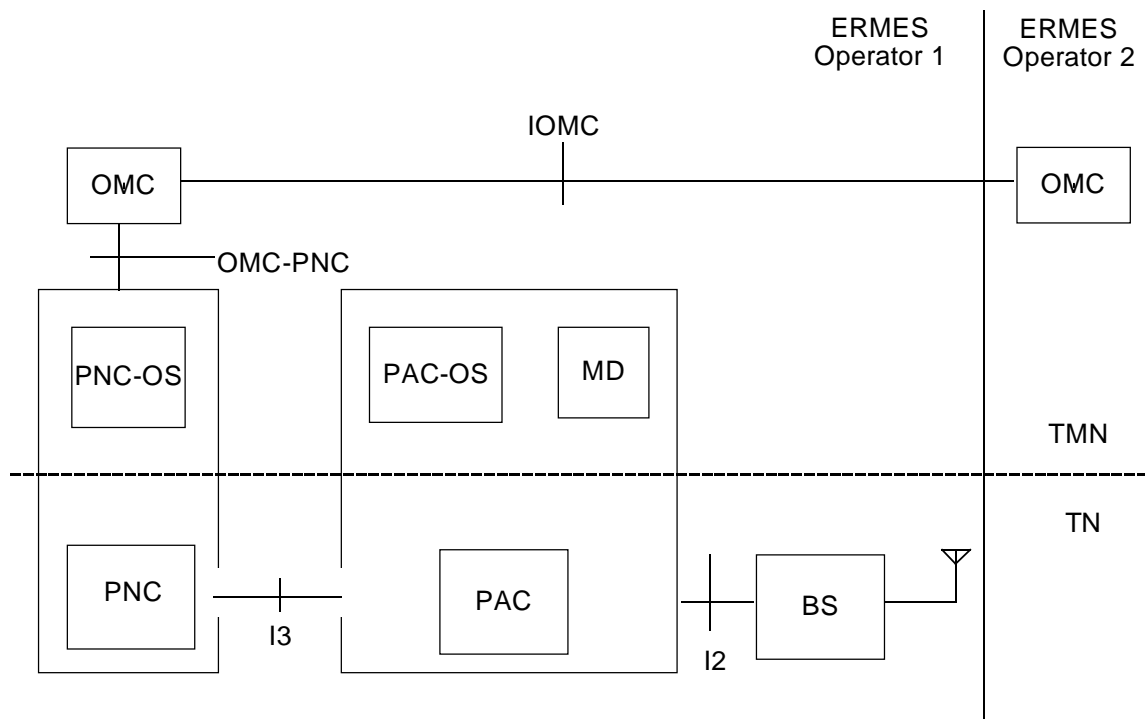
Figure 4: O&M interfaces
