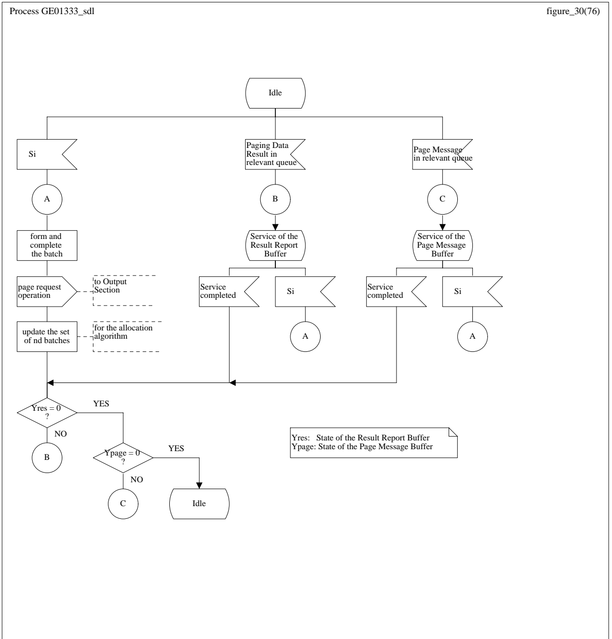
Figure 46: Message queuing and control - SDL diagram
