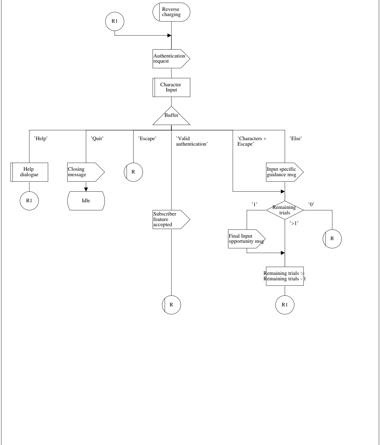
Figure D.3.5: Reverse charging request
