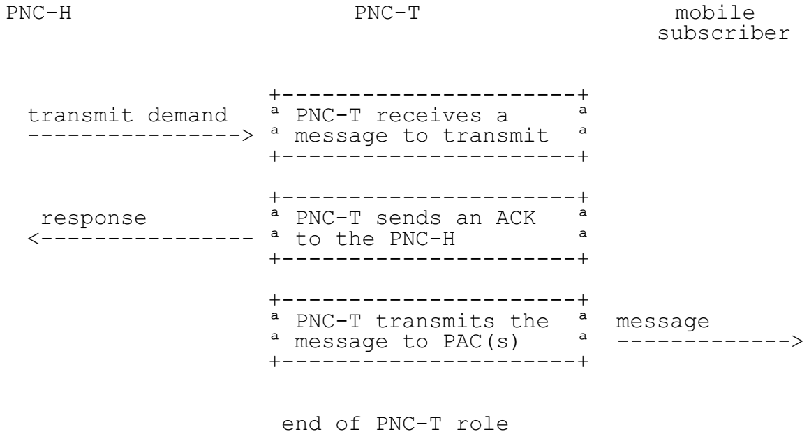
Figure 8: PNC-T processing
