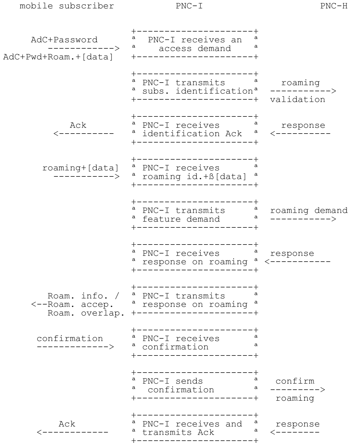
Figure 10: PNC-I processing
