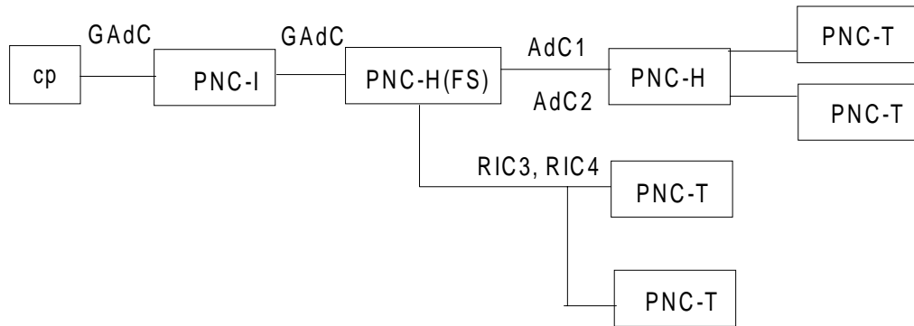
Figure 9: Group call processing
