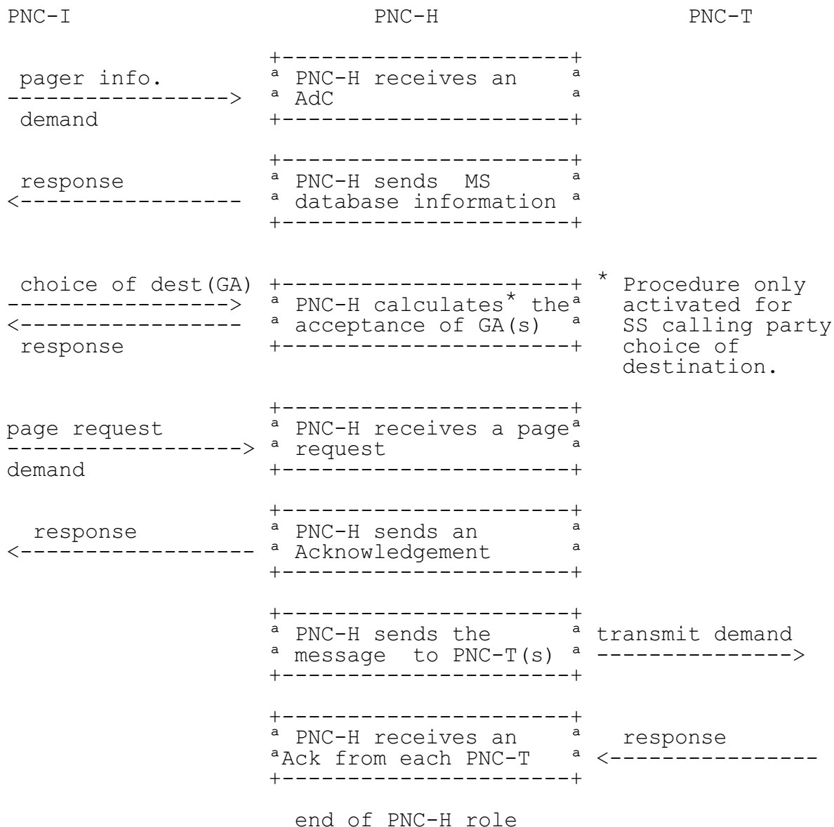
Figure 7: PNC-H processing
