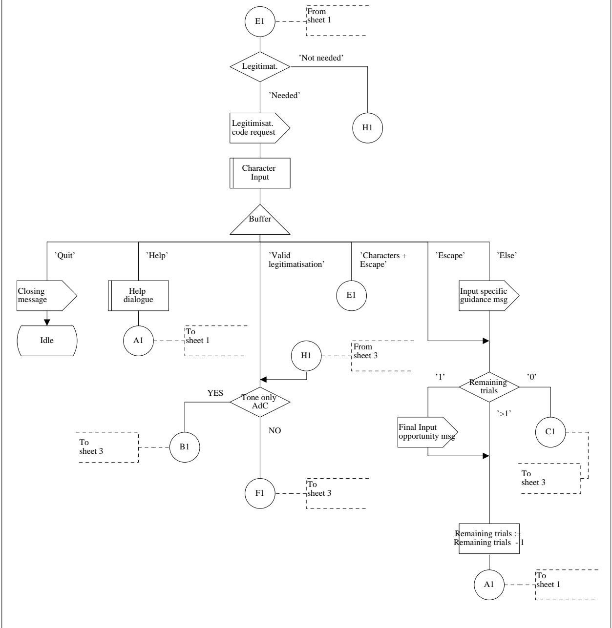
Figure D.2 (sheet 2 of 4): Two-stage selection protocol via service number 1
