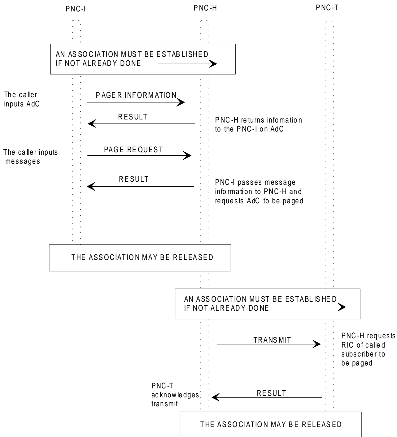
Figure 18: Flow diagram showing call processing for paging
