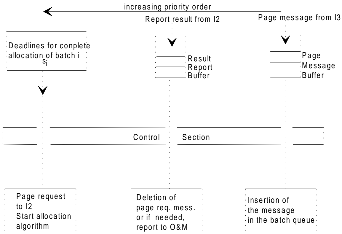
Figure 42: Functionality of the control section
