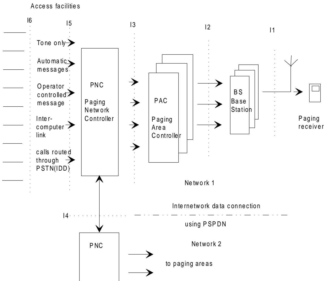
Figure 2: Functional organization of the Telecommunication Network (TN) architecture
