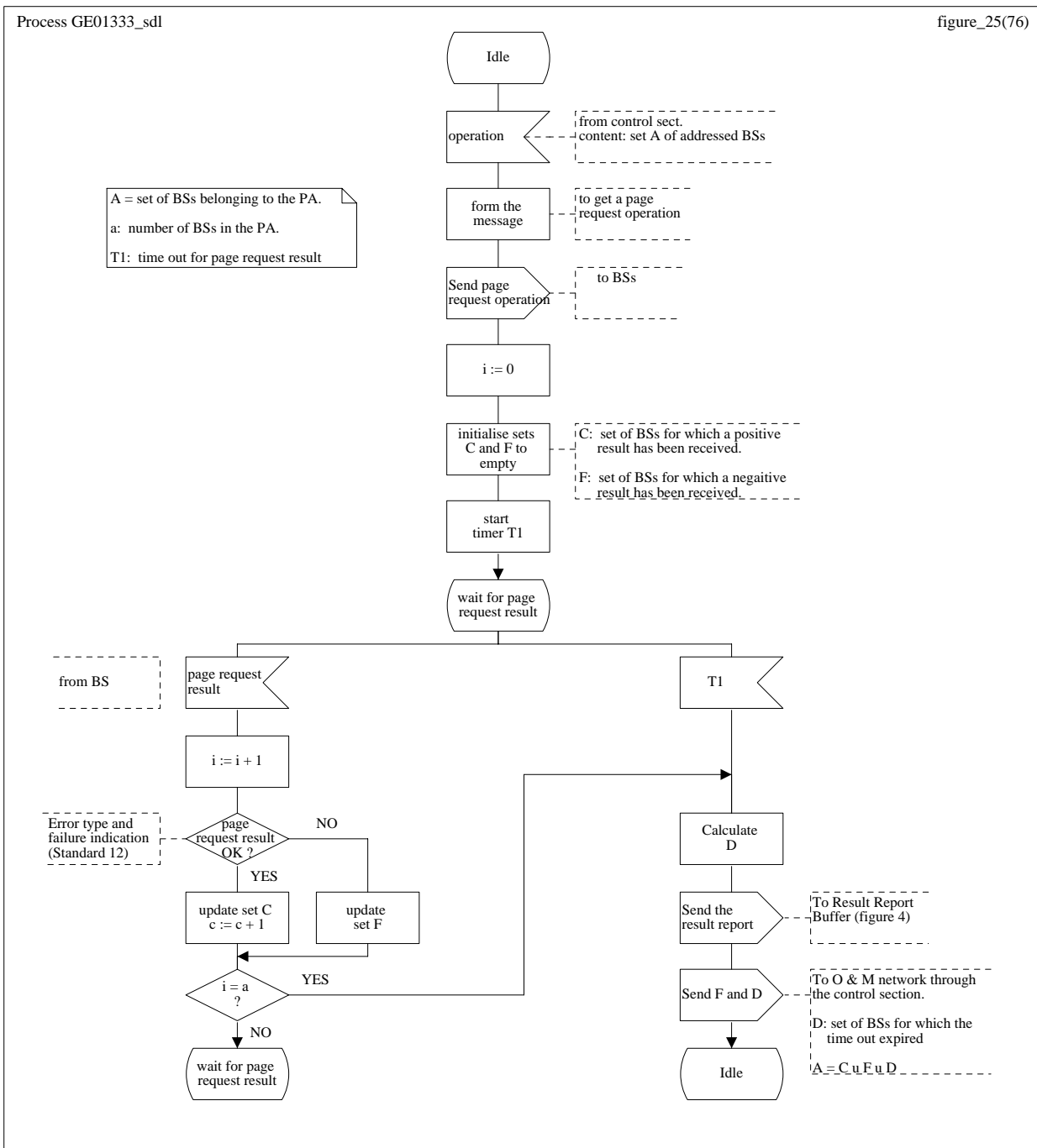
Figure 41: SDL diagram for output section - application functions
