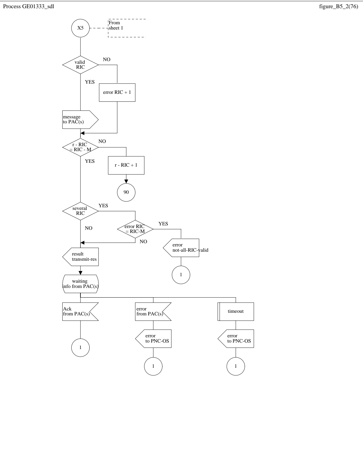
Figure B.5 (sheet 2 of 2): Call processing for page input - external call, PNC-T
