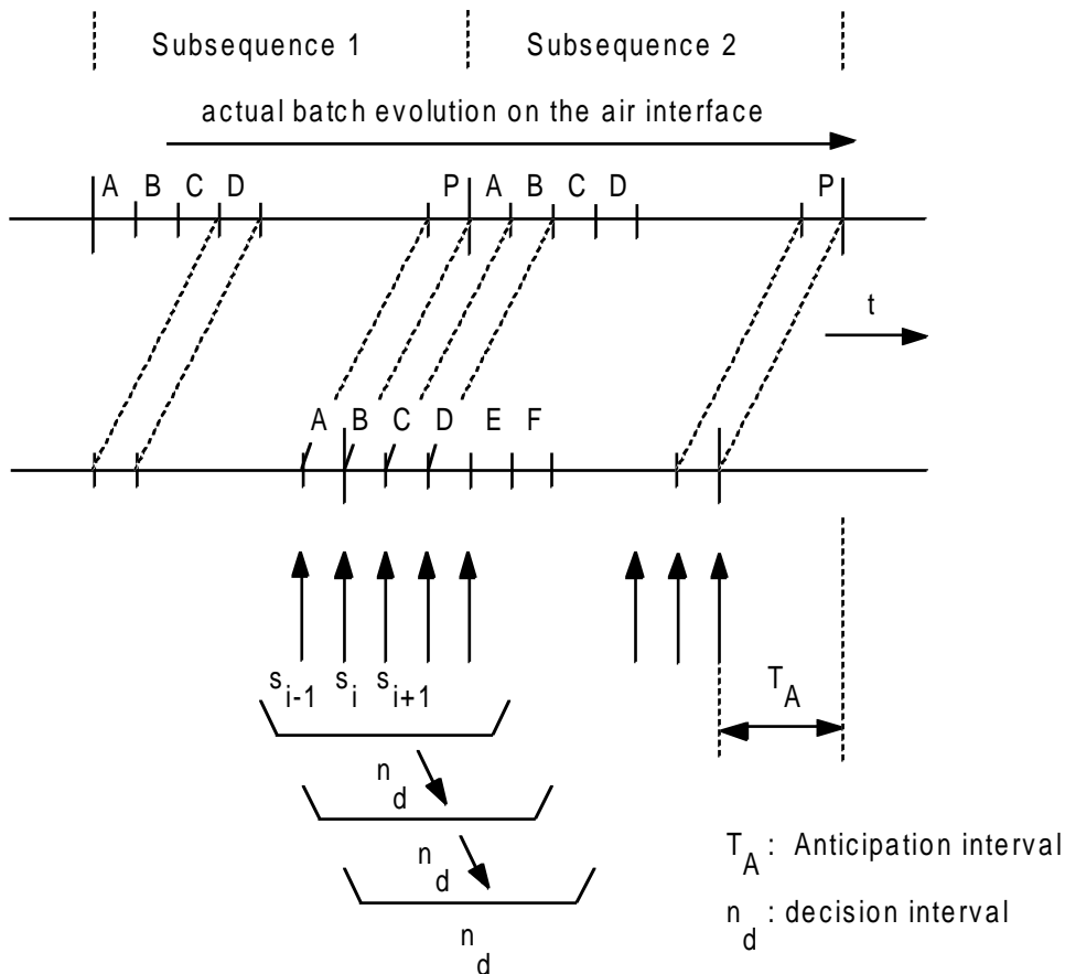
Figure 44: Time anticipation for message transmission and allocation
