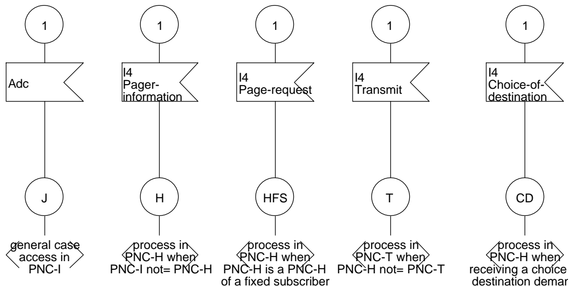
Figure B.1: Call processing for page input
