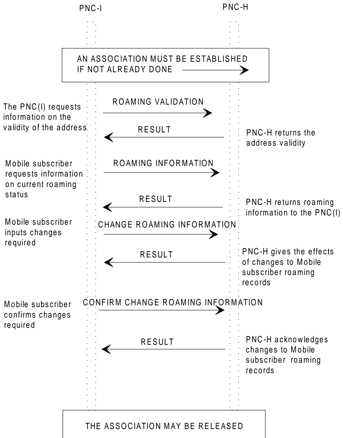
Figure 19: Flow diagram showing call processing for roaming
