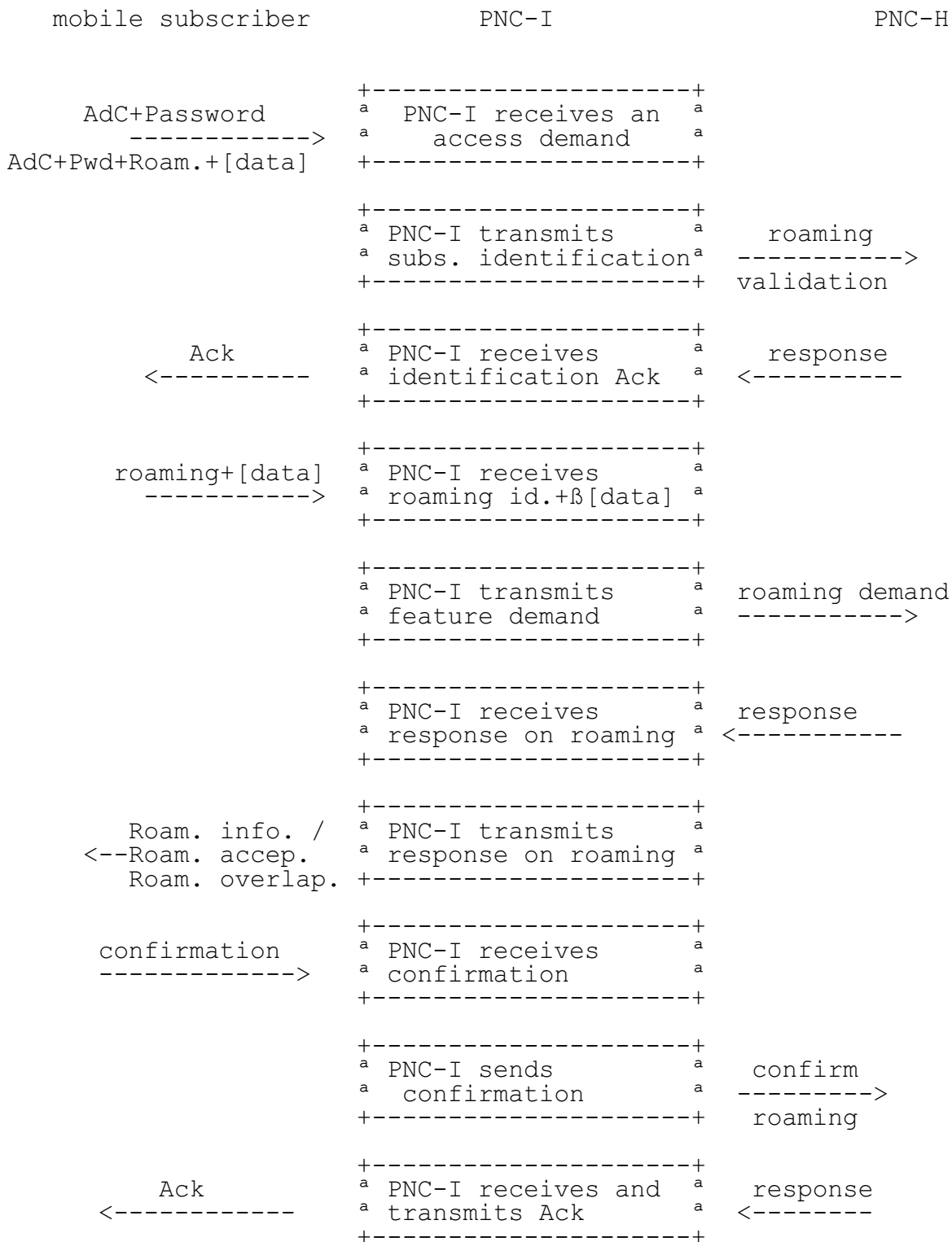
Figure 10: PNC-I processing
