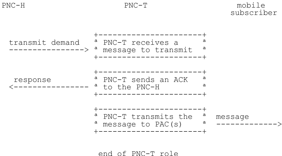
Figure 8: PNC-T processing
