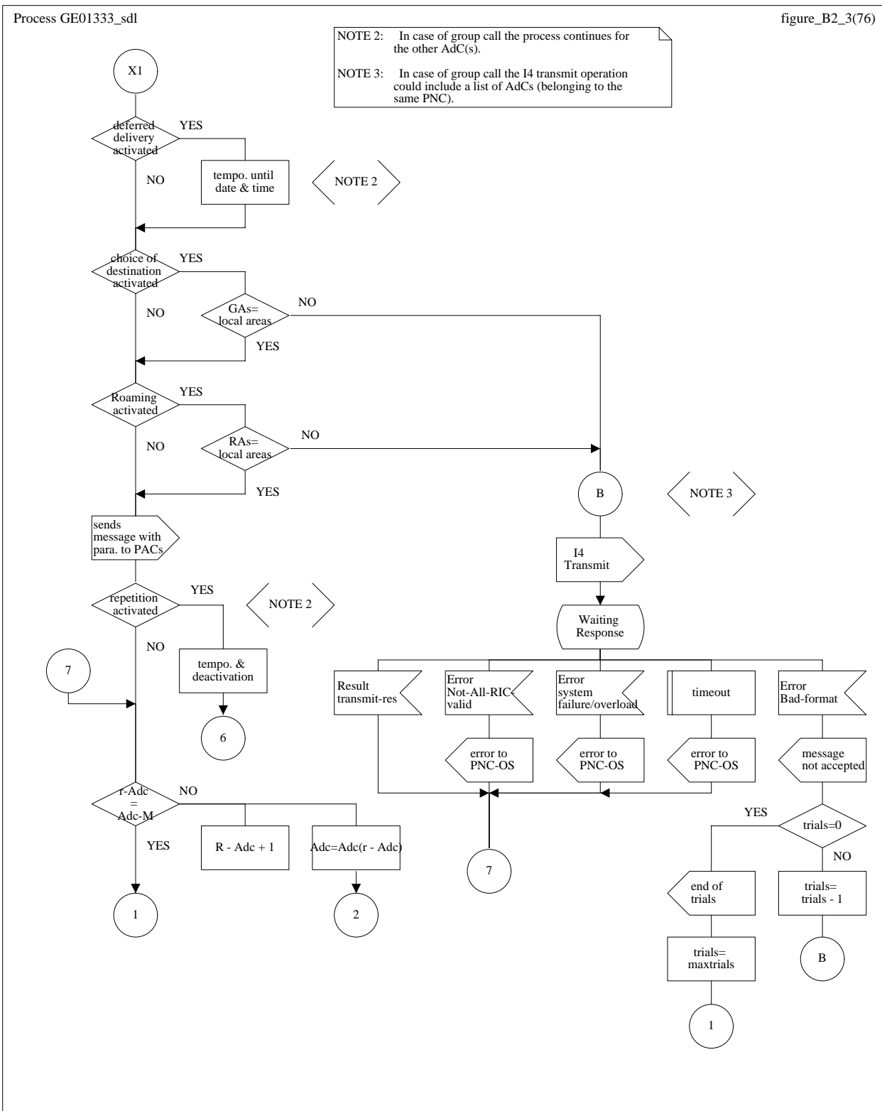
Figure B.2 (sheet 3 of 5): Call processing for page input - local call
