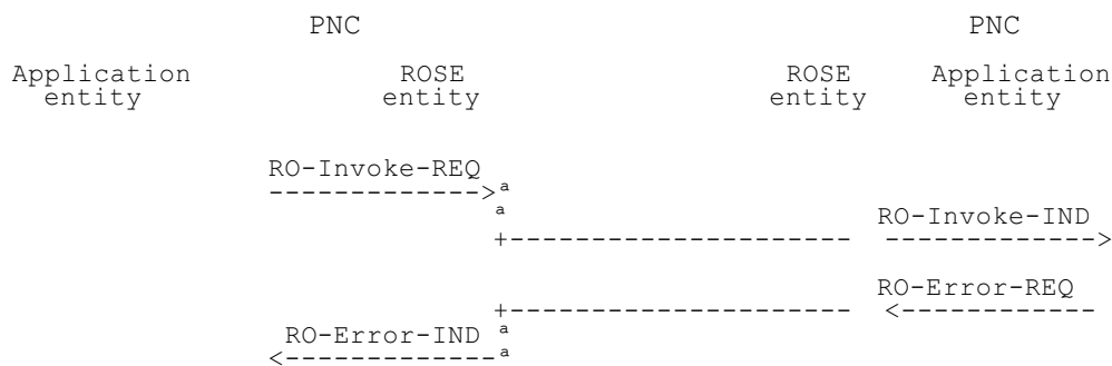
Figure 21: Operation invocation and negative report
