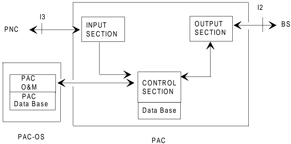
Figure 38: PAC architecture
