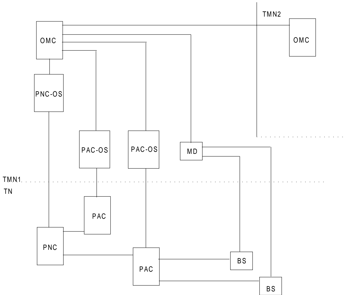
Figure 3: ERMES functional architecture
