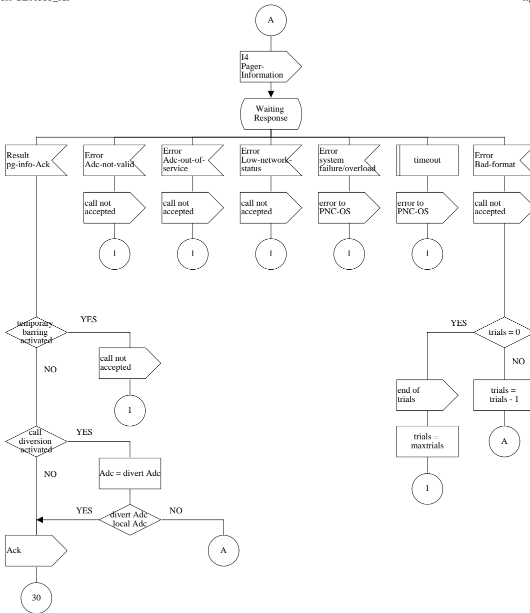
Figure B.3 (sheet 1 of 6): Call processing for page input - distant call, PNC-I
