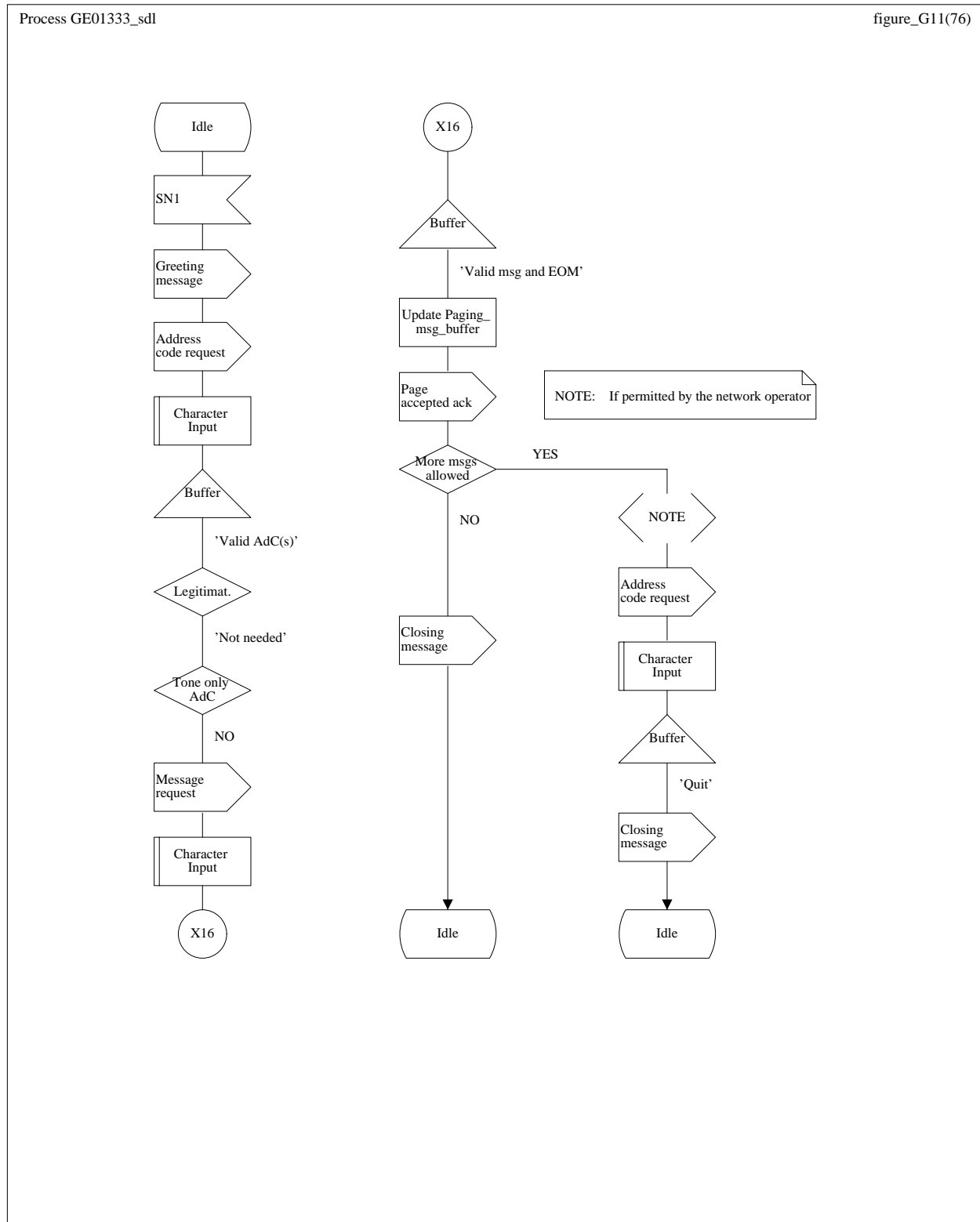
Figure G.1.1: A typical two-stage selection call with no supplementary services
