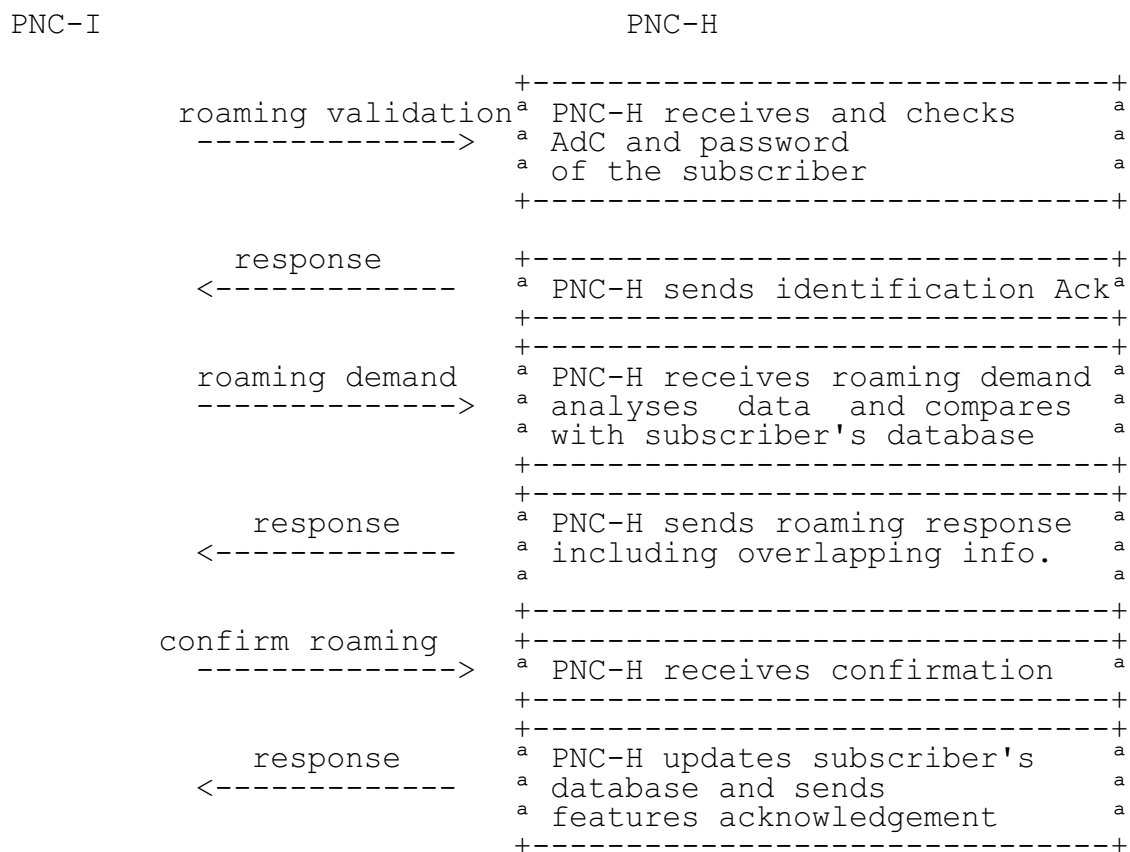
Figure 11: PNC-H processing
