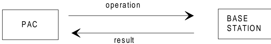
Figure 23: Layer 7 transaction
