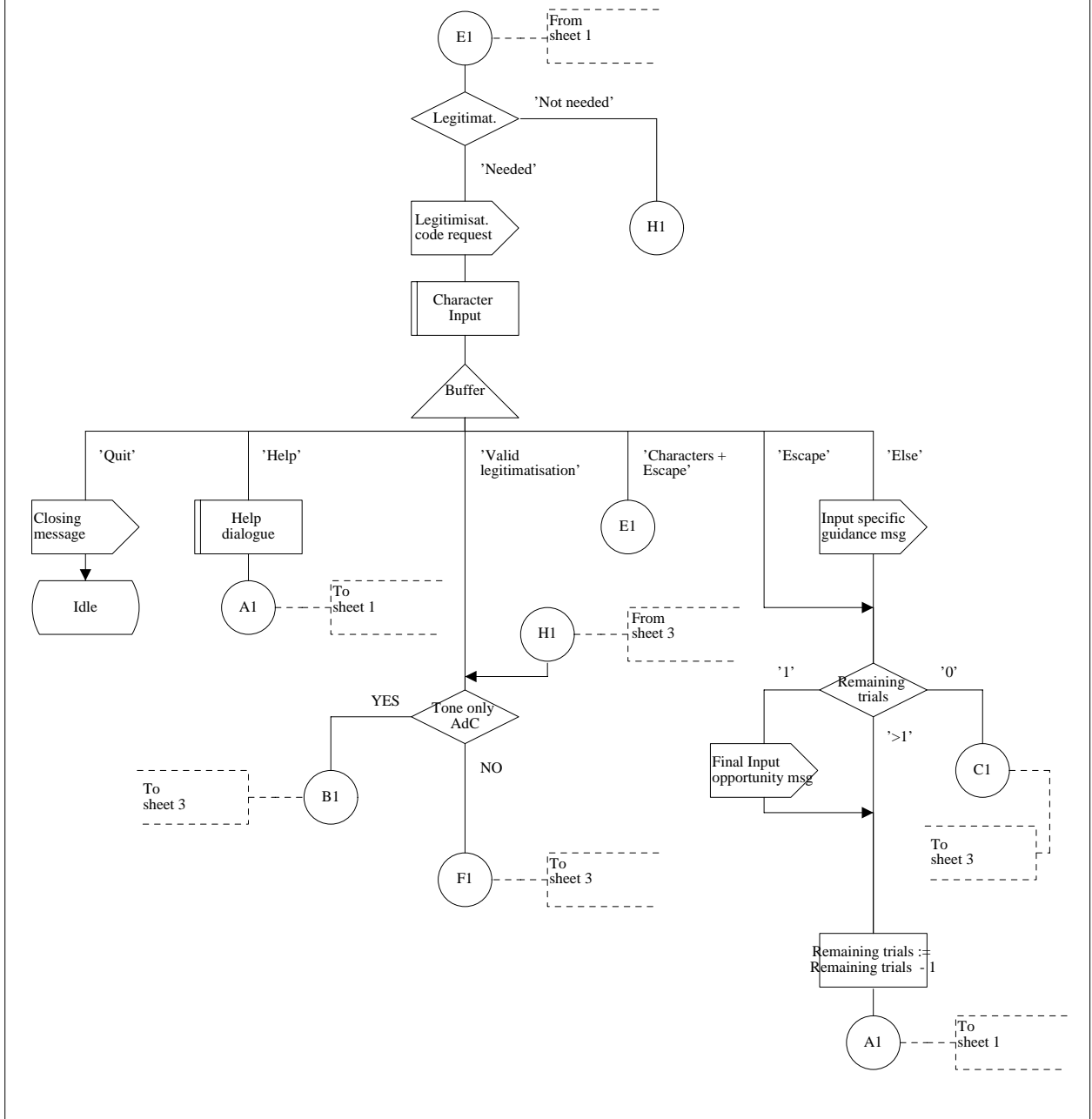
Figure D.2 (sheet 2 of 4): Two-stage selection protocol via service number 1
