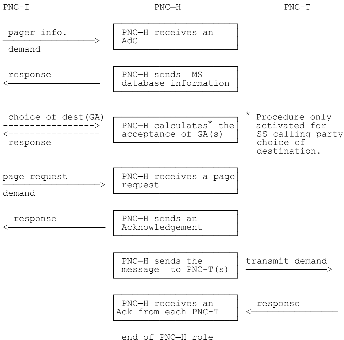
Figure 7: PNC-H processing
