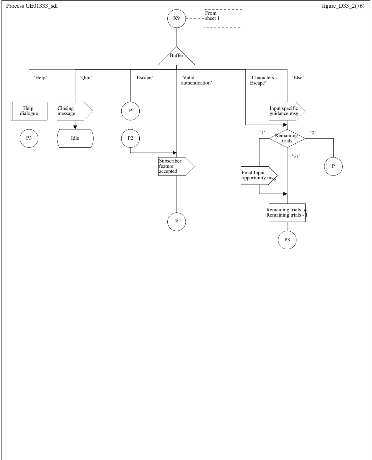
Figure D.3.3 (sheet 2 of 2): Priority
