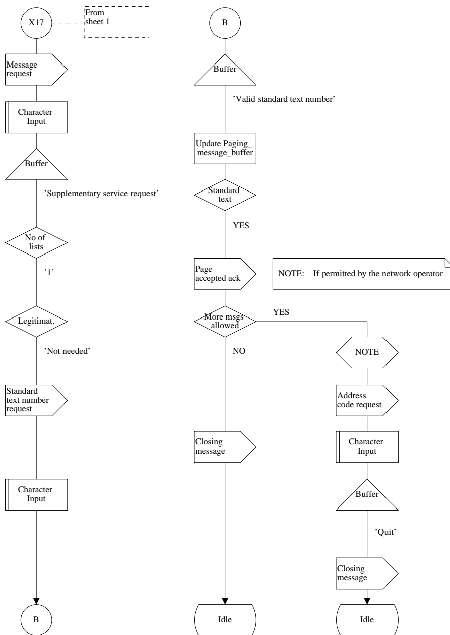
Figure G.1.2 (sheet 2 of 2): A typical two-stage selection call with level 1 priority and standard text
