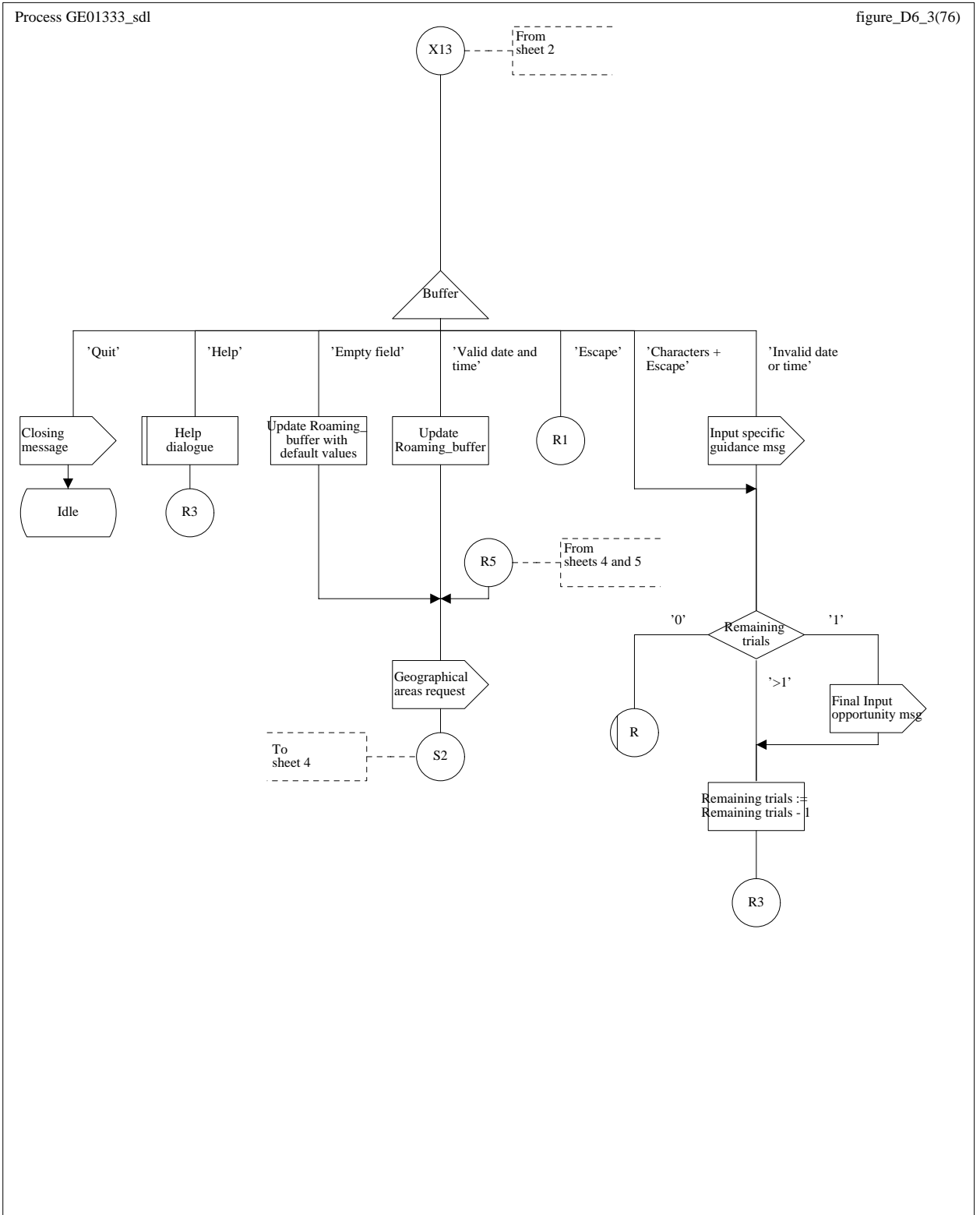
Figure D.6 (sheet 3 of 6): Roaming dialogue
