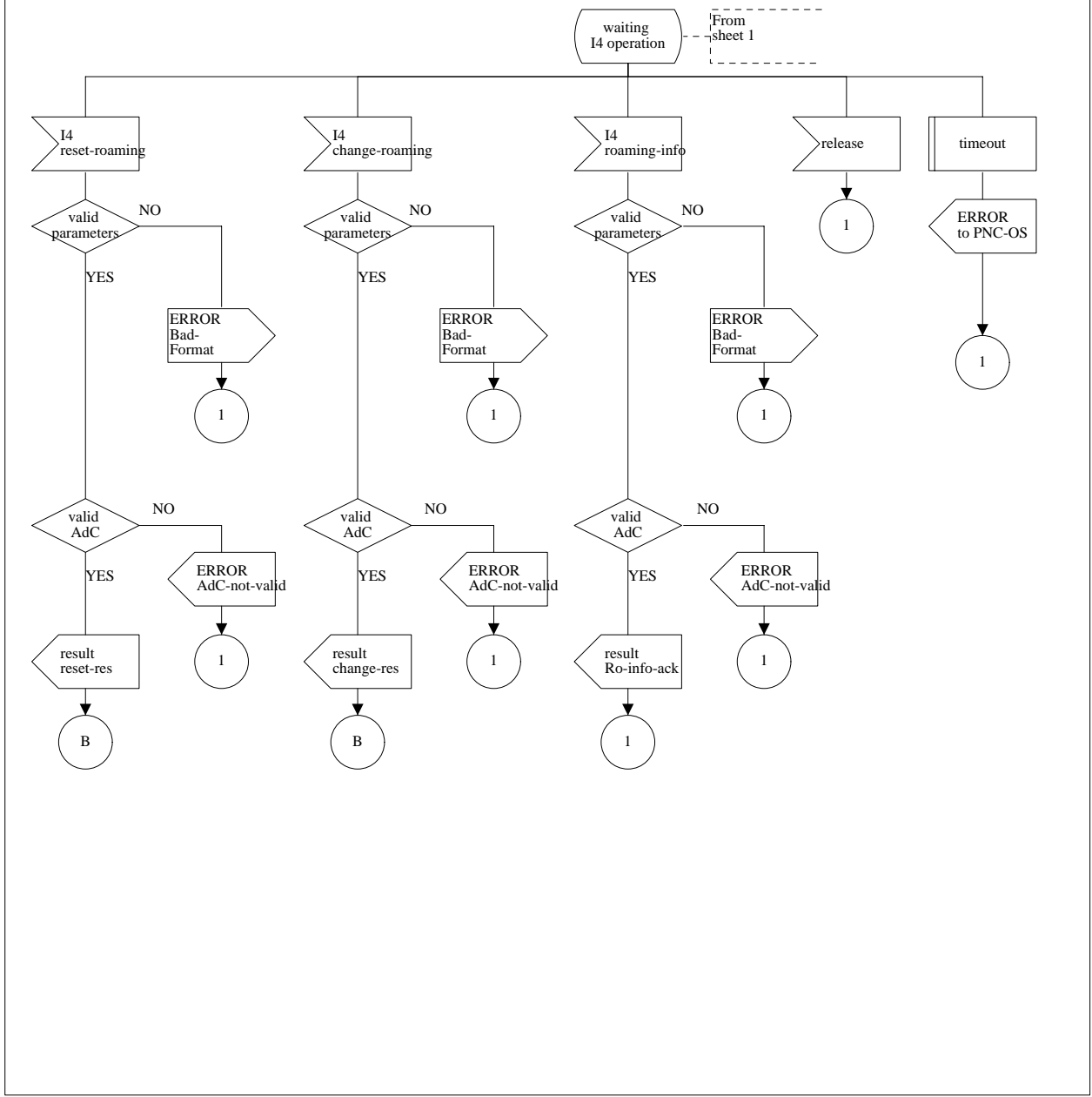
Figure B.10 (sheet 2 of 2): Call processing for roaming - distant call, PNC-H
