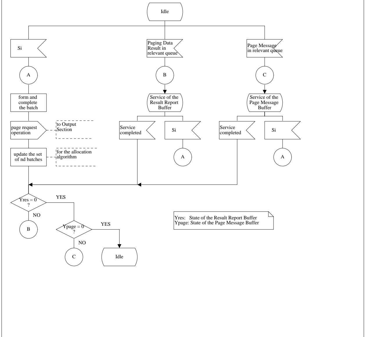
Figure 46: Message queuing and control - SDL diagram
