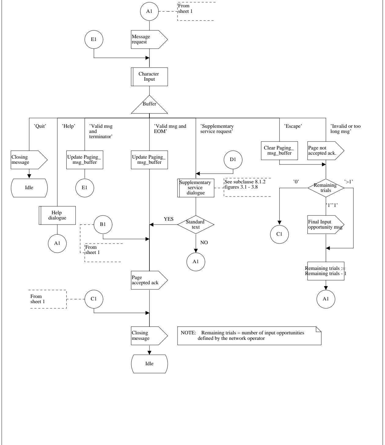
Figure D.4 (sheet 2 of 3): one-stage selection protocol for page input - interactive mode
