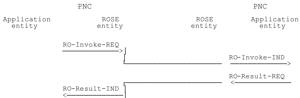
Figure 20: Operation invocation and positive report
