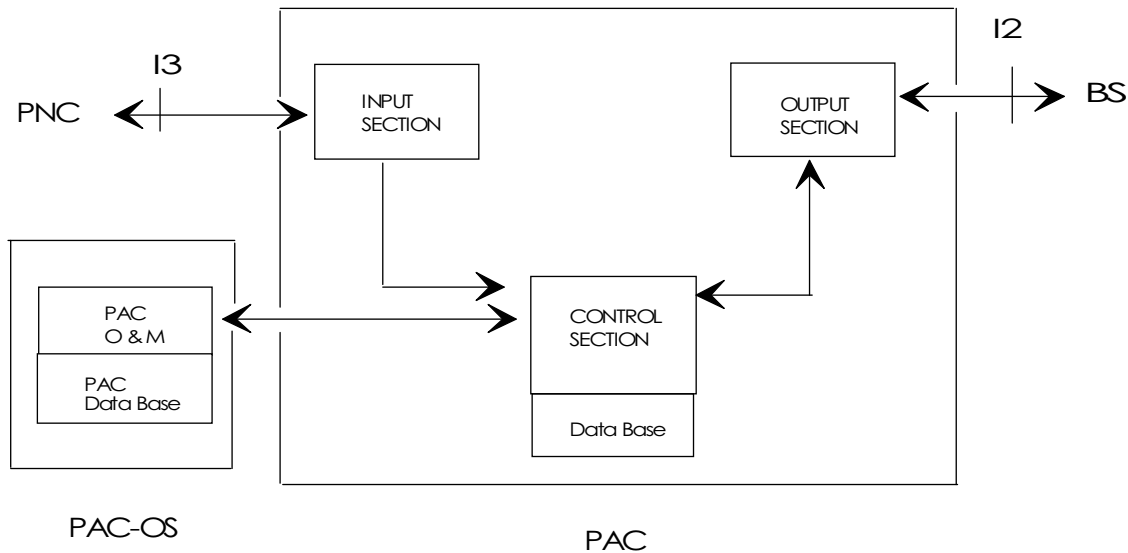
Figure 38: PAC architecture
