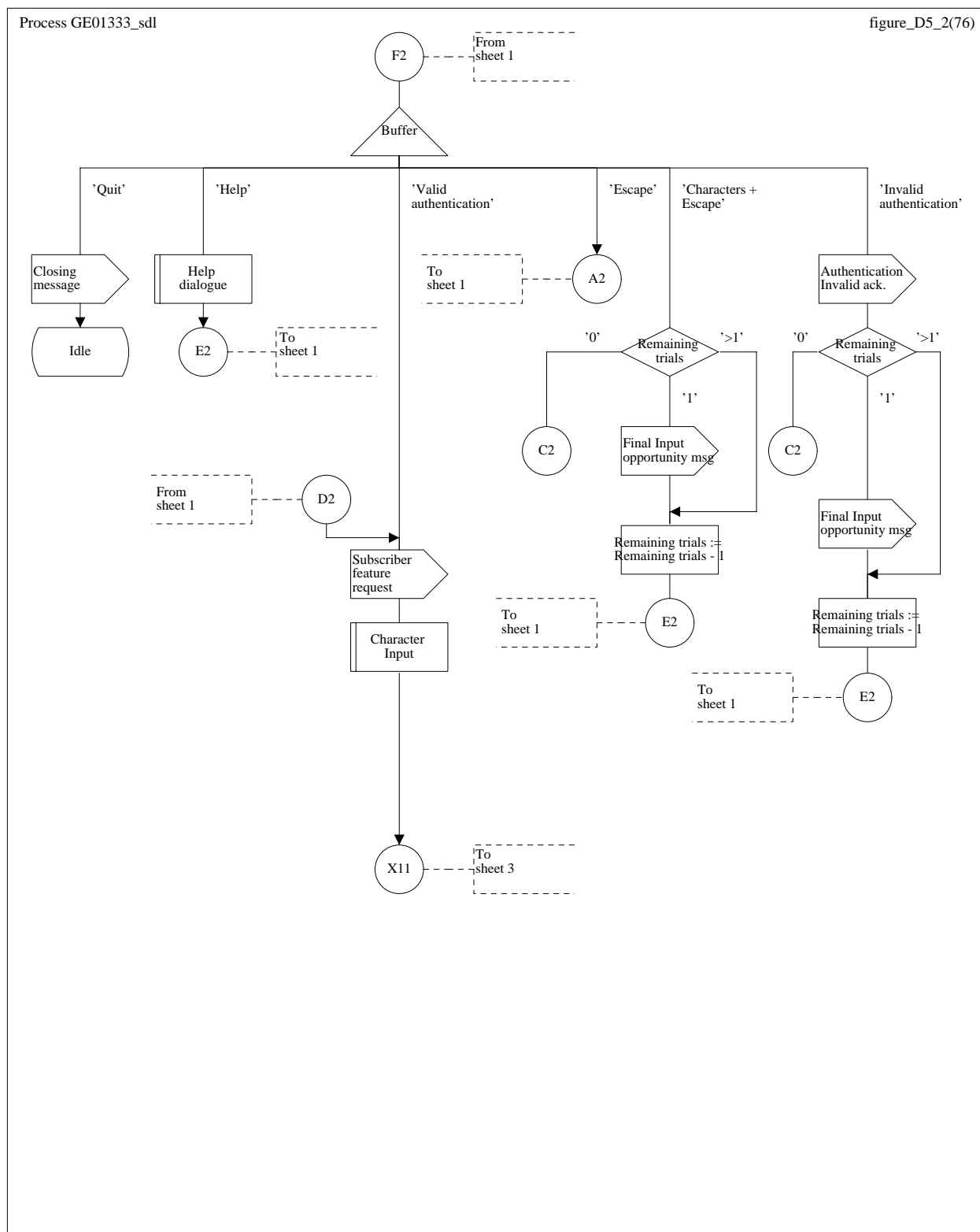
Figure D.5 (sheet 2 of 2): Two-stage selection protocol via service number 2
