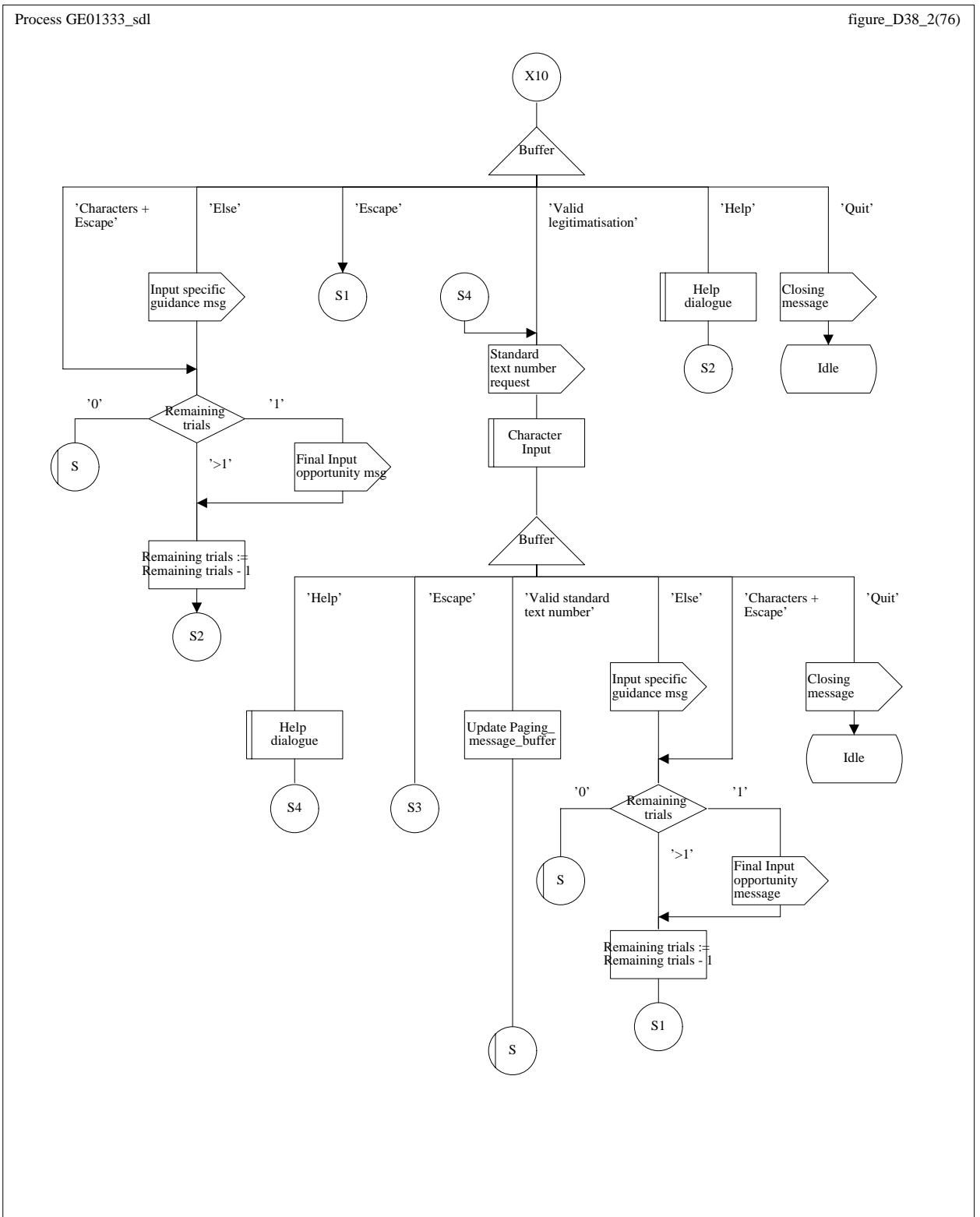
Figure D.3.8 (sheet 2 of 2): Standard text dialogue
