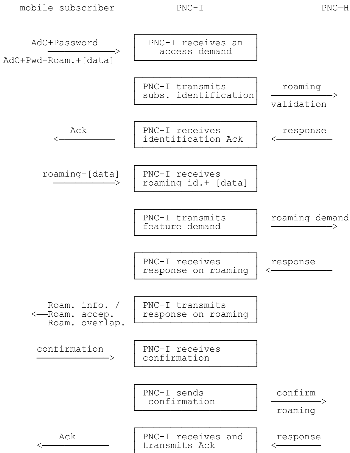
Figure 10: PNC-I processing
