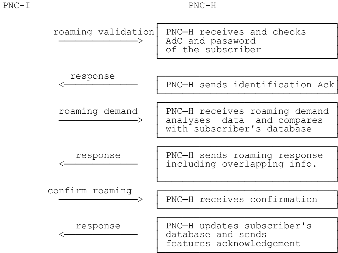
Figure 11: PNC-H processing
