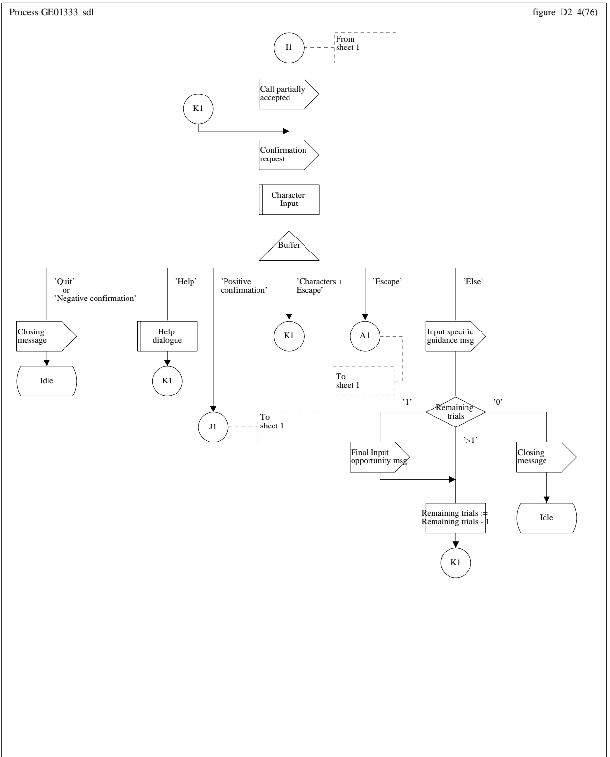
Figure D.2 (sheet 4 of 4): Two-stage selection protocol via service number 1
