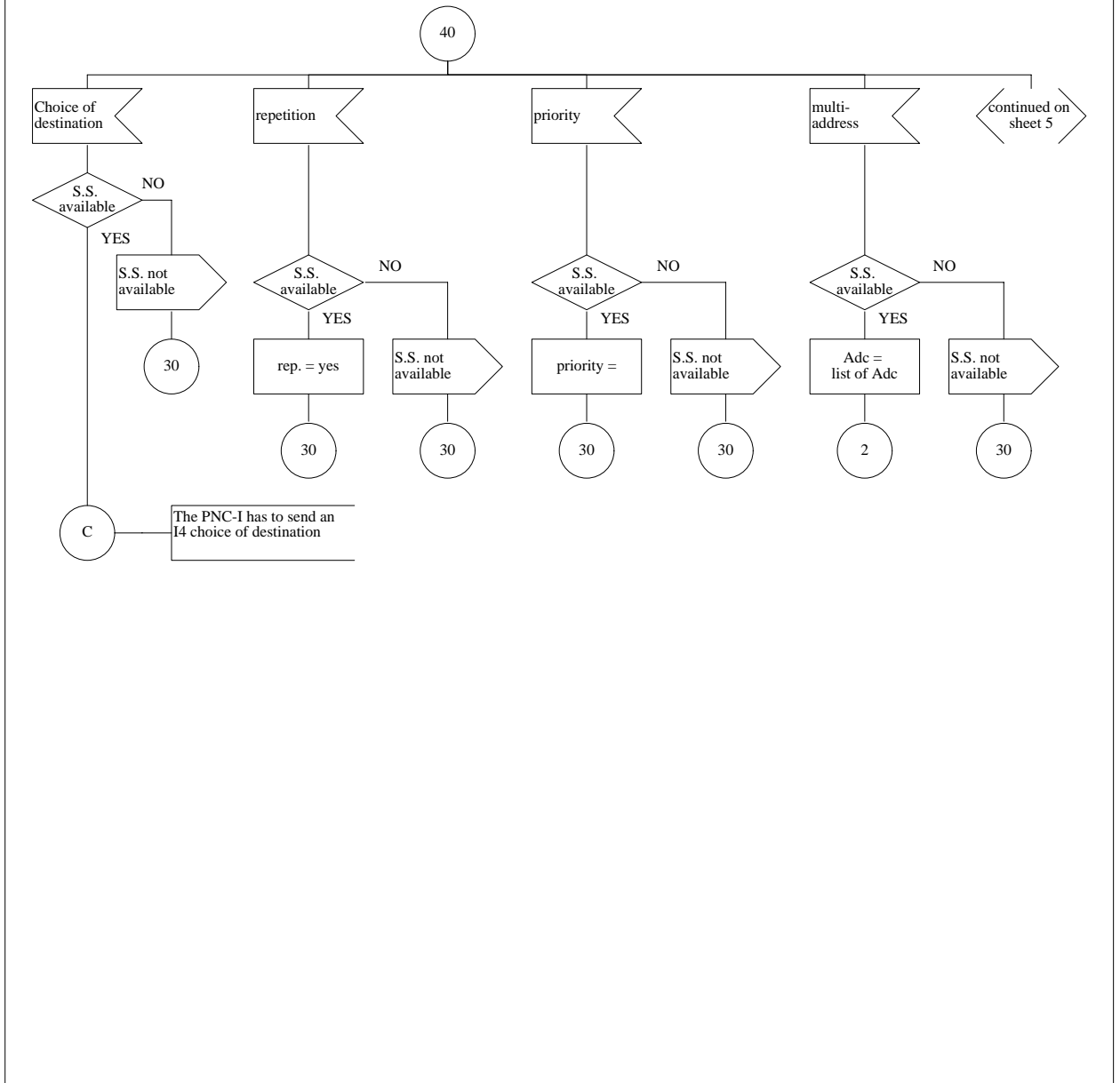
Figure B.3 (sheet 4 of 6): Call processing for page input - distant call, PNC-I
