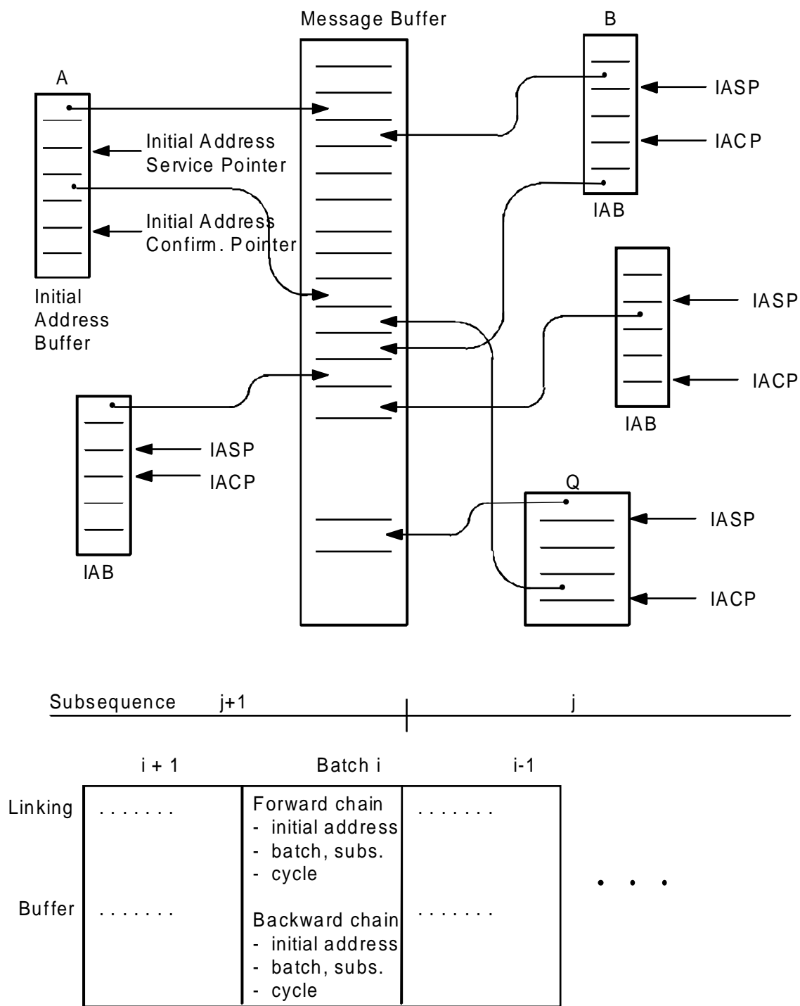
Figure 45: Message queuing and control - conceptual representation
