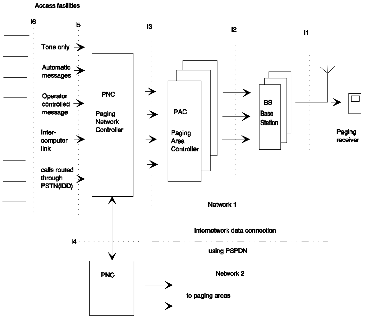
Figure 2: Functional organization of the telecommunication network architecture
