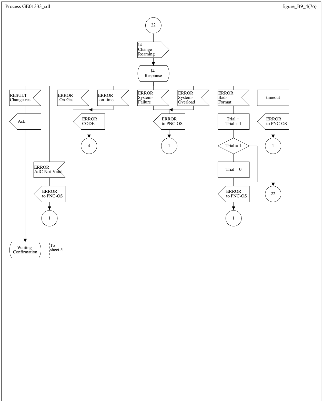
Figure B.9 (sheet 3 of 5): Call processing for roaming - distant call, PNC-I
