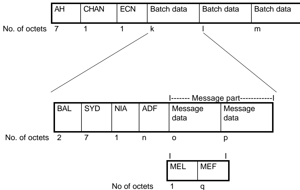
Figure 25: Page request frame structure
