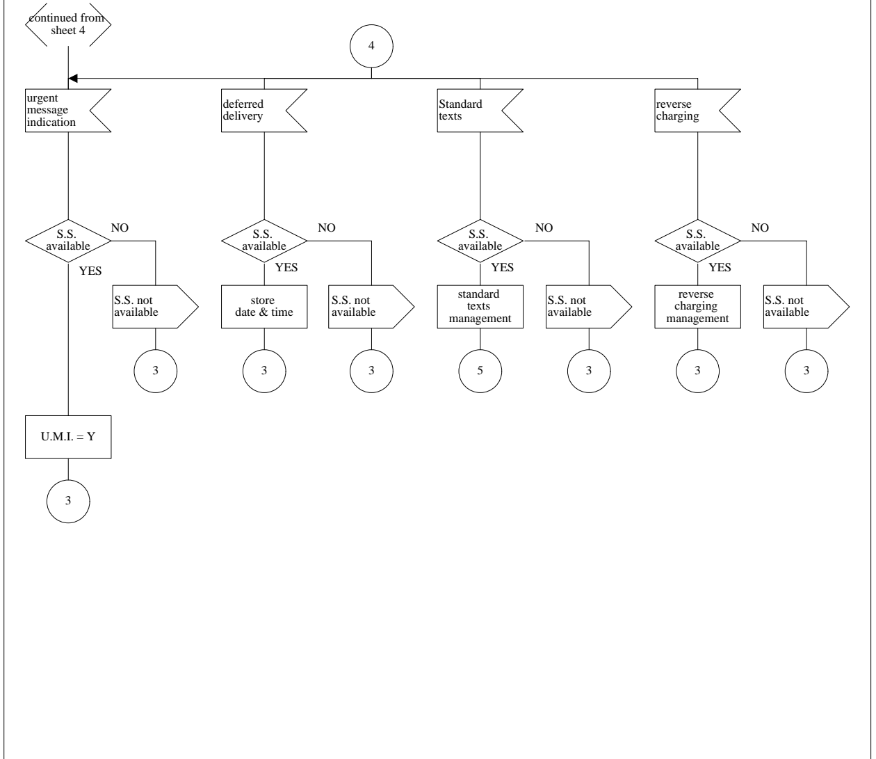
Figure B.2 (sheet 5 of 5): Call processing for page input - local call
