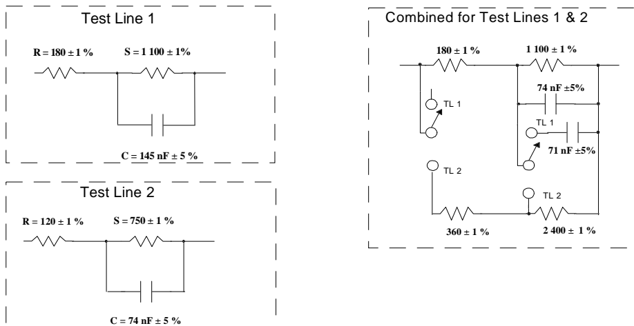
Figure C.4: Hybrid characteristics
