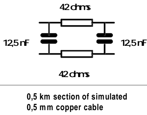
Figure C.3: Local line simulators - schematic
