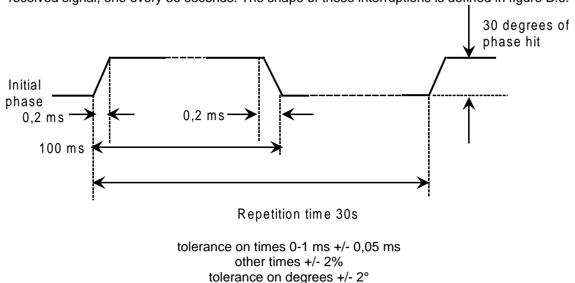
Figure B.3: Phase hits
