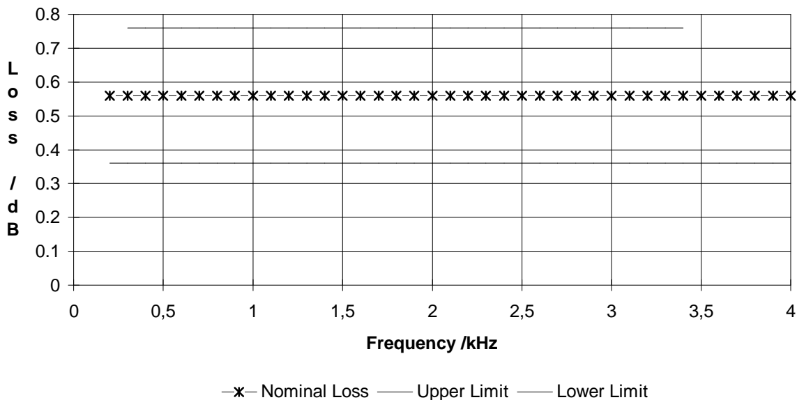
Figure C.14: Test Line 2 - Trunk network simulator - insertion loss frequency characteristic
