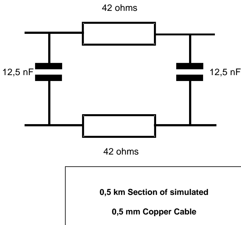
Figure C.3: Local line simulators - schematic
