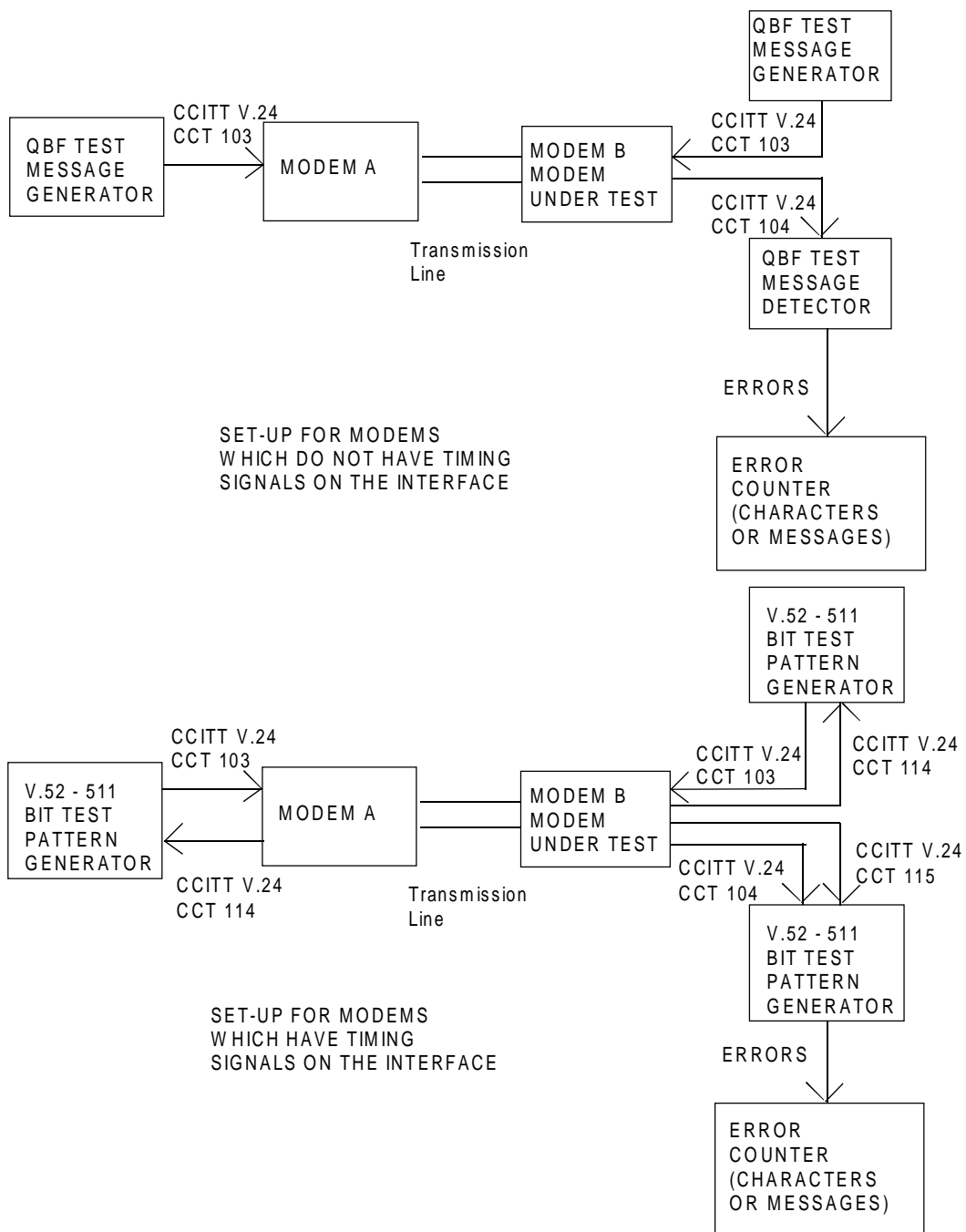
Figure B.2: Set-up for modem connection to the test generator
