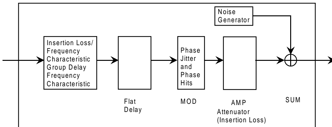
Figure C2: Trunk Network Simulator
