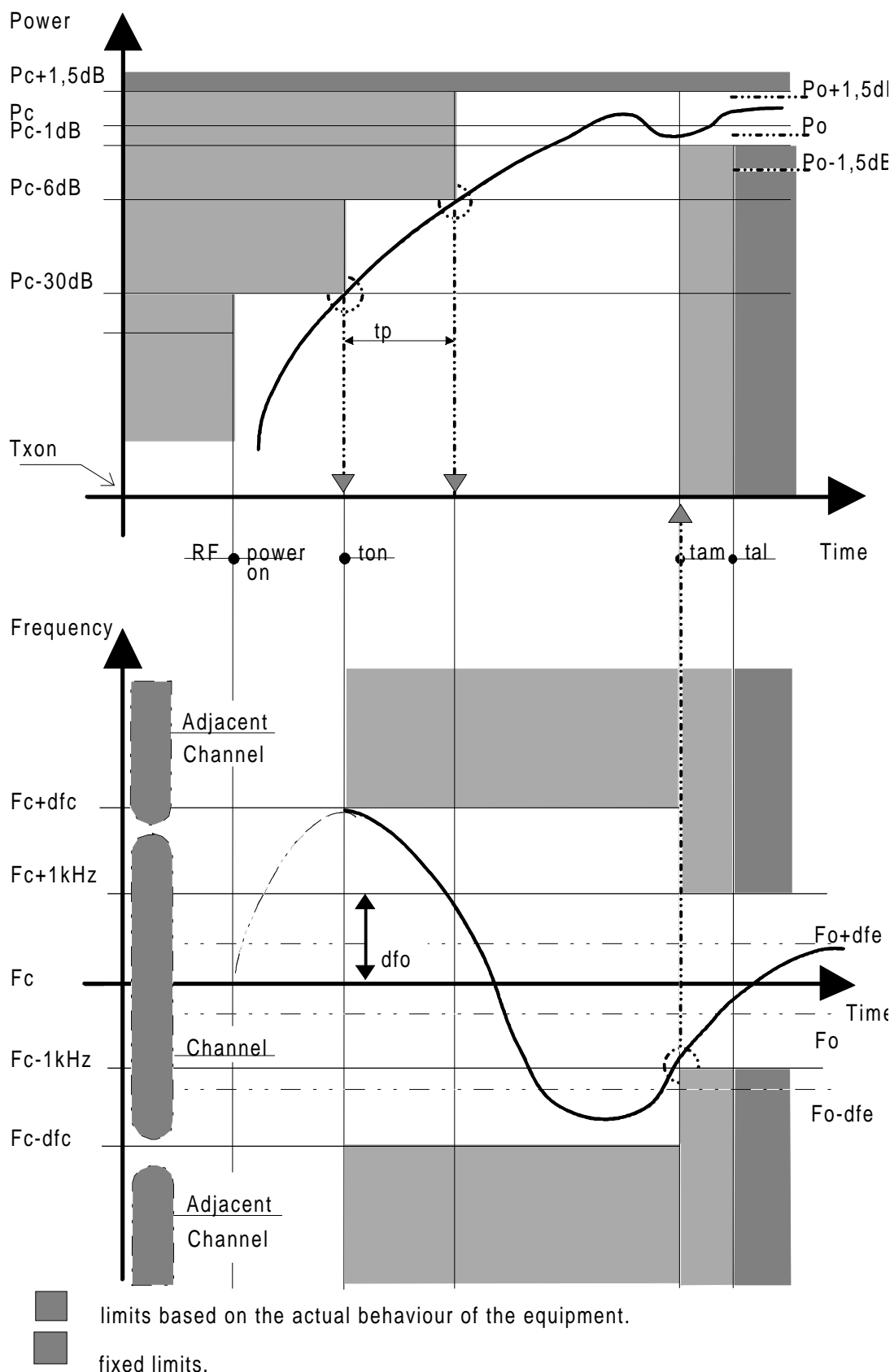
Figure 13: Transmitter attack time according to subclause 8.8.1 b) and transient behaviour during switch-on. (Case where the attack time is given by the behaviour of the frequency)
