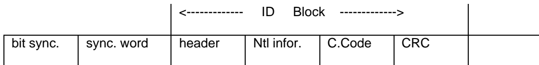
Figure C.1: ID block organisation
