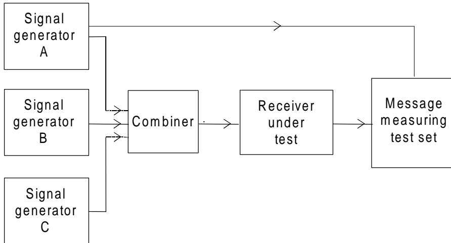
Figure 27: Measurement arrangement
