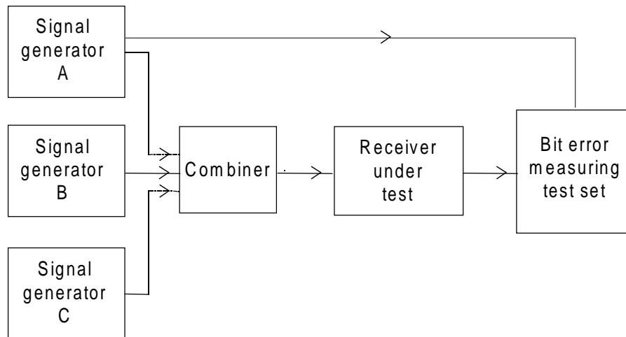
Figure 28: Measurement arrangement
