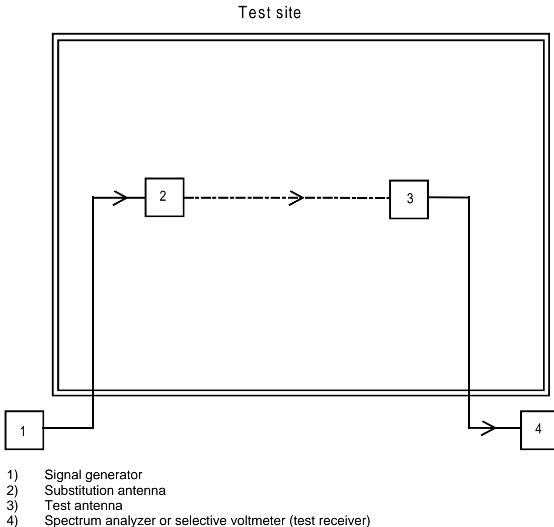
Figure 10: Measurement arrangement
