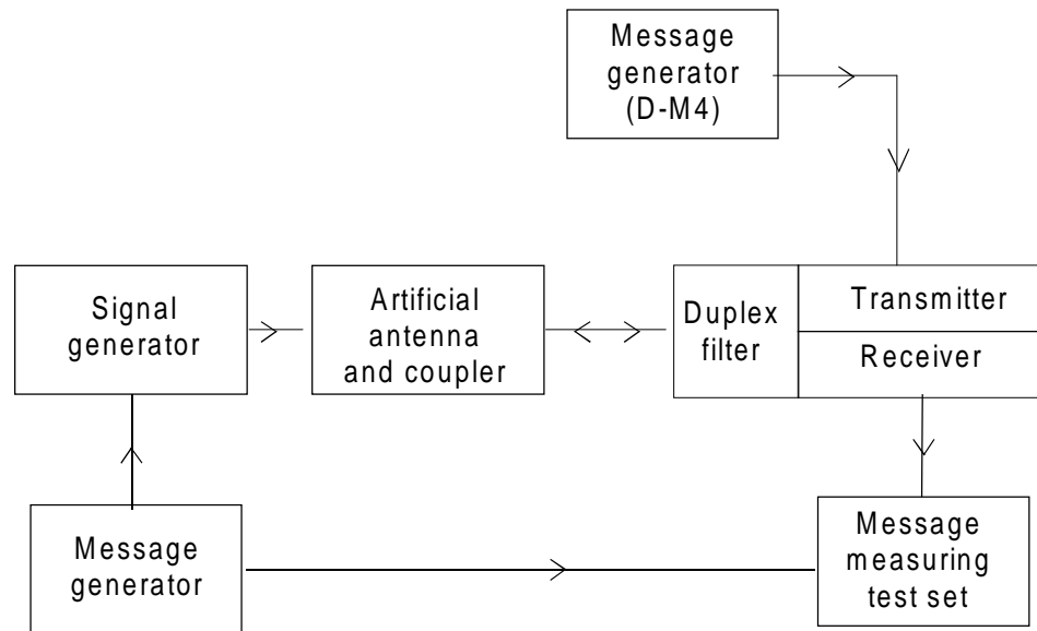
Figure 35: Measurement arrangement
