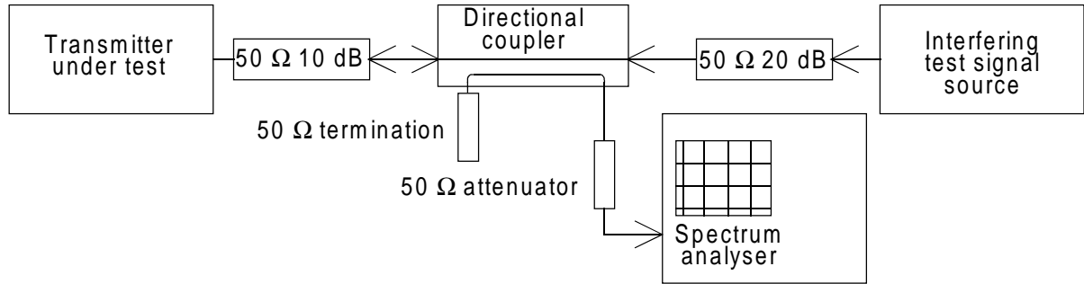
Figure 11: Measurement arrangement
