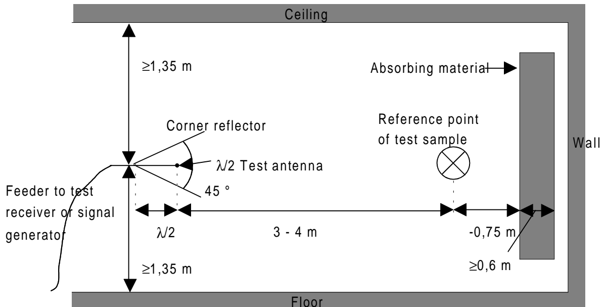
Figure A.2: Indoor site arrangement (shown for horizontal polarisation).
