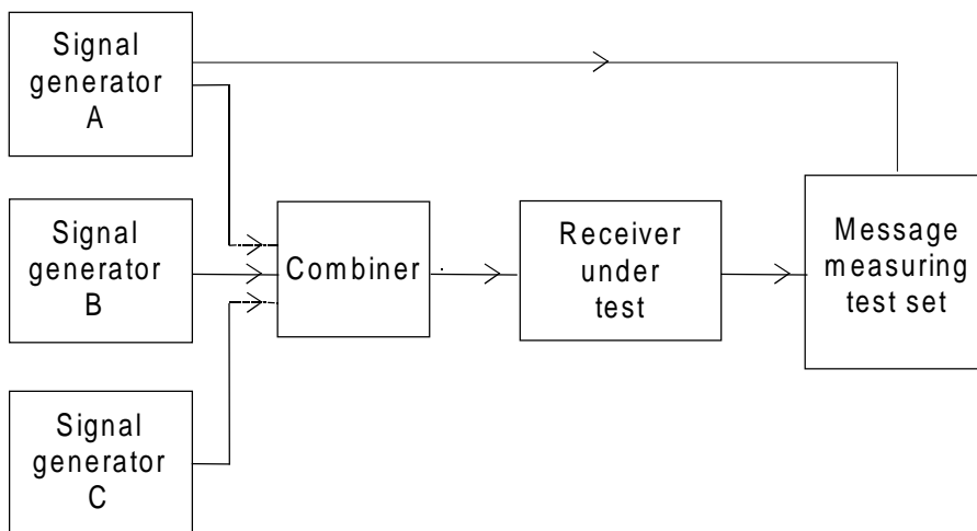
Figure 29: Measurement arrangement
