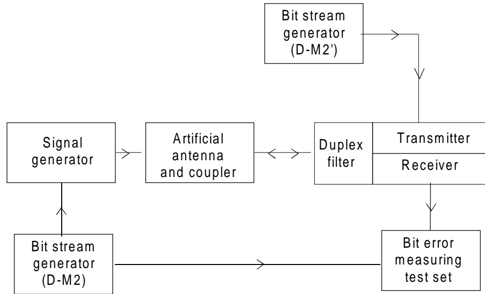
Figure 33: Measurement arrangement
