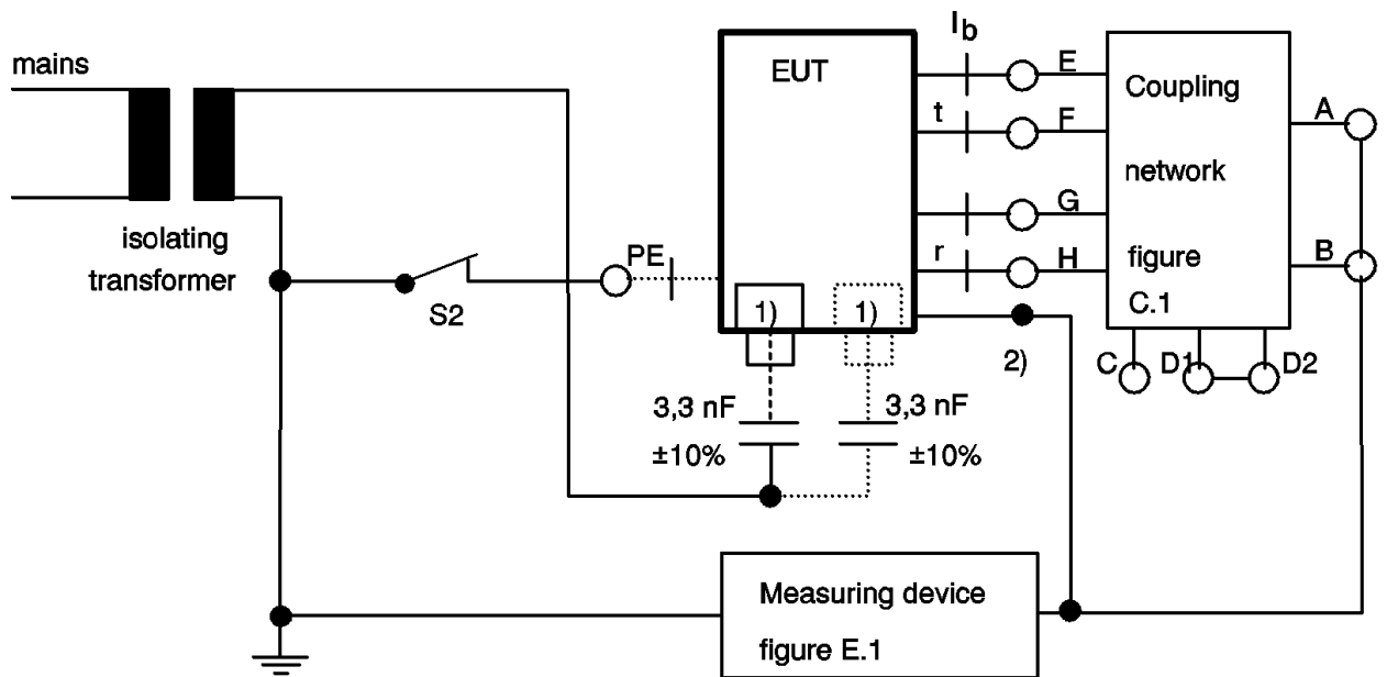
Figure 2: Touch current test circuit for mains powered equipment having auxiliary interfaces
