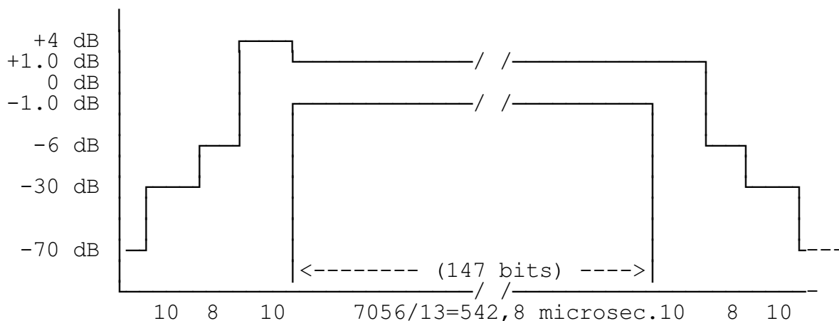
Fig.II.3.3. Power/time template. For a transmitter carrier power lower than 3423 dBm, where the level of -70 dB is lower than - 3647 dBm, the -70 dB shall be replaced by a value which is equivalent to - 3647 dBm.
