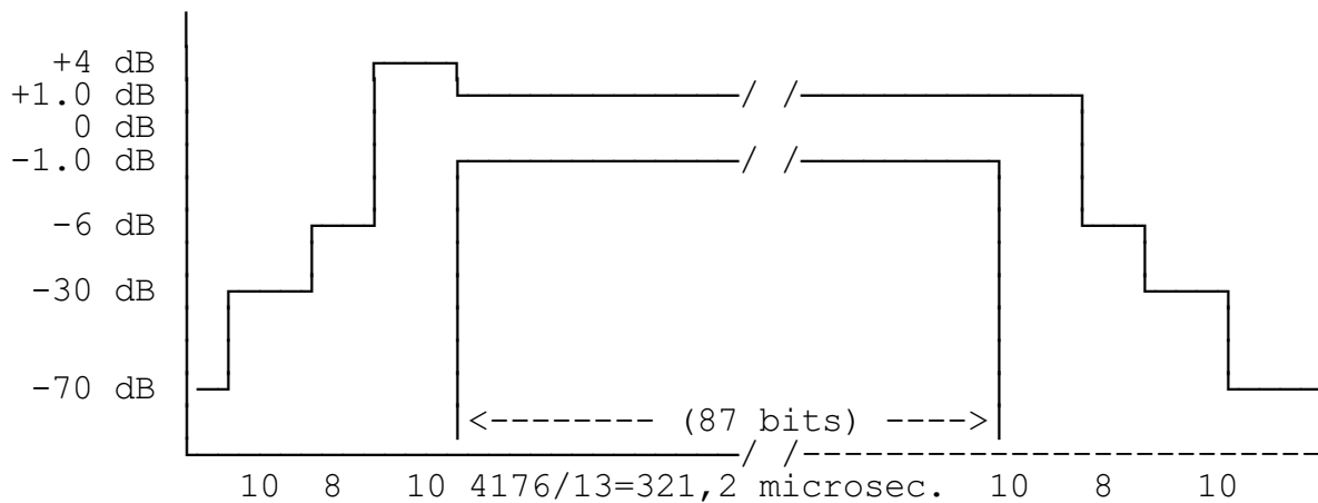
Fig. II.3.4: Power/Time Template for Access Burst. For a transmitter carrier power lower than 3423 dBm, where the level of -70 dB is lower than -3647 dBm, the -70 dB shall be replaced by a value which is equivalent to -3647 dBm.
