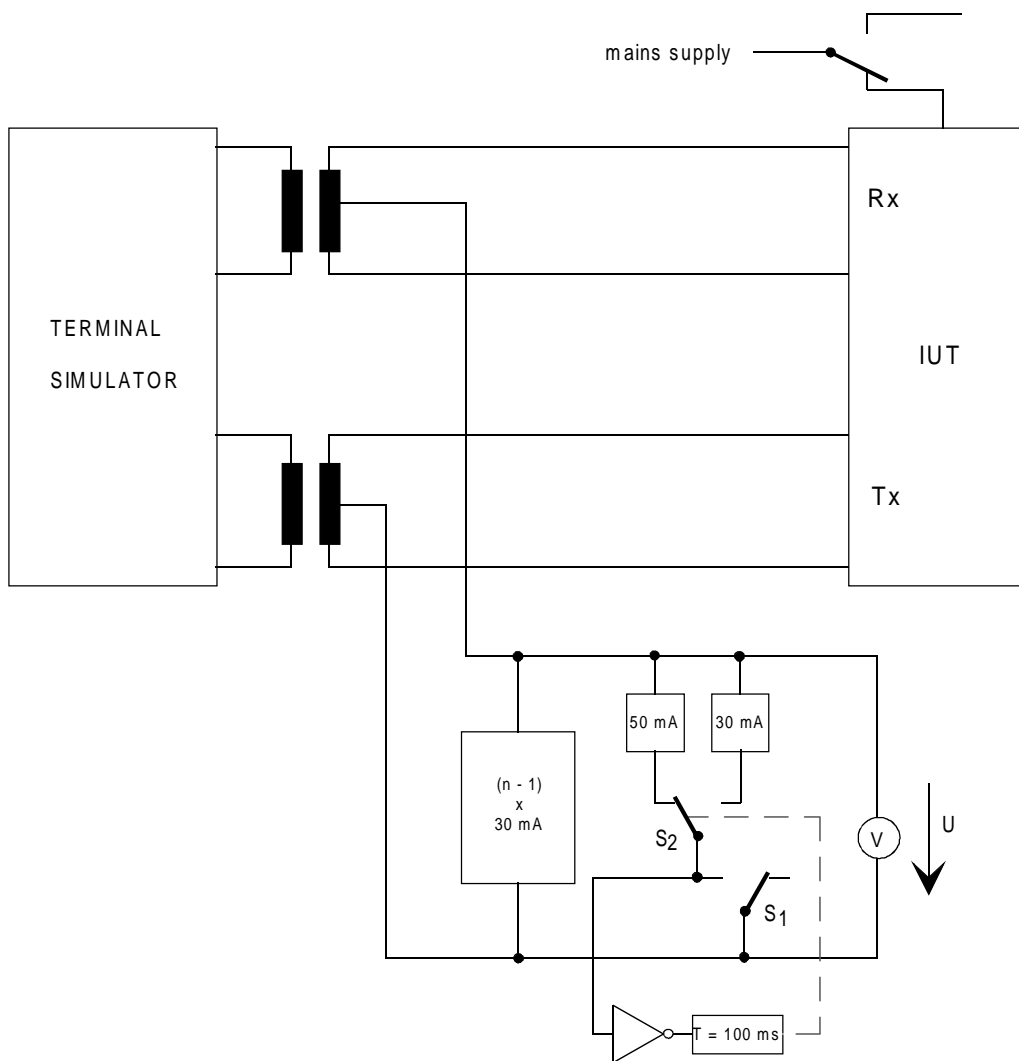
Figure 42: Test configuration
