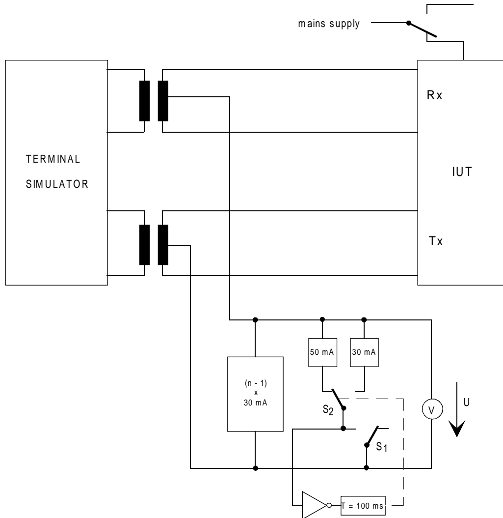
Figure 34: Test configuration
