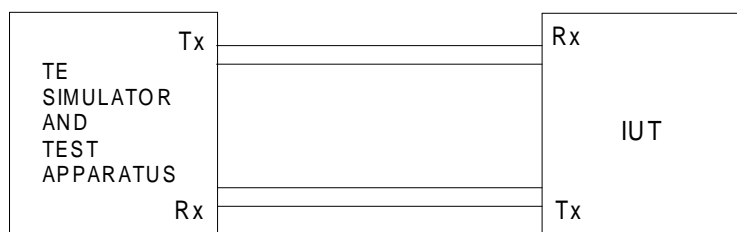
Figure 1: Test configuration
