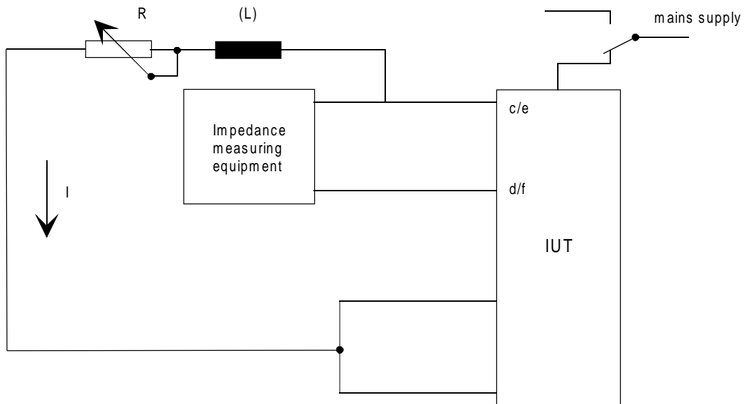
Figure 43: Test configuration
