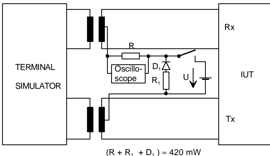
Figure 44: Test configuration
