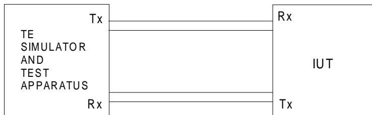
Figure 4: Test configuration
