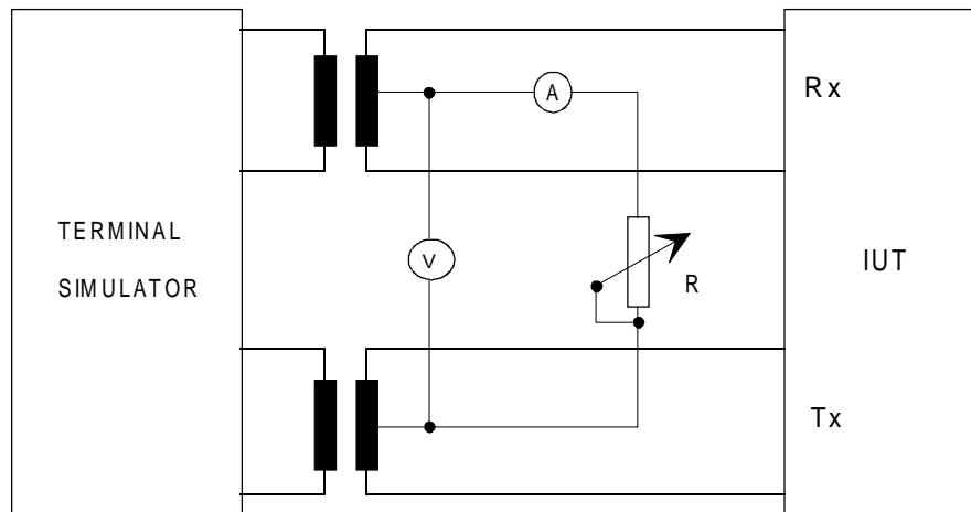
Figure 26: Test configuration
