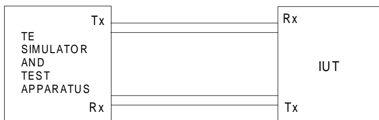
Figure 2: Test configuration
