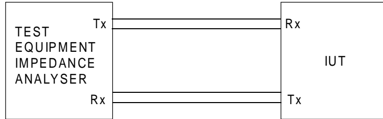
Figure 14: Test configuration
