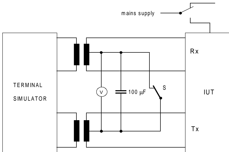
Figure 31: Test configuration
