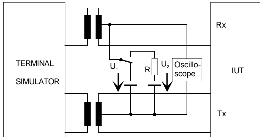
Figure 45: Test configuration
