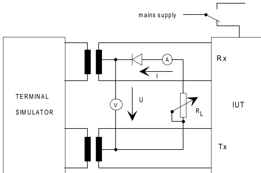
Figure 28: Test configuration
