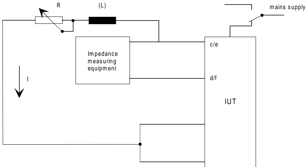
Figure 36: Test configuration
