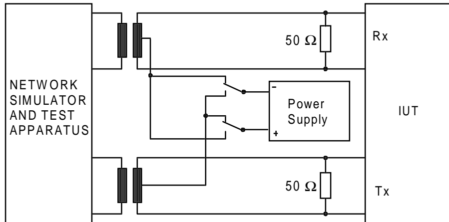
Figure 60: Test configuration
