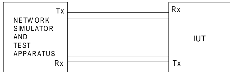
Figure 19: Test configuration
