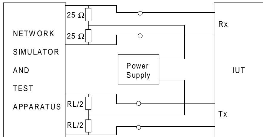
Figure 23: Test configuration
