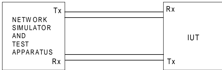
Figure 7: Test configuration
