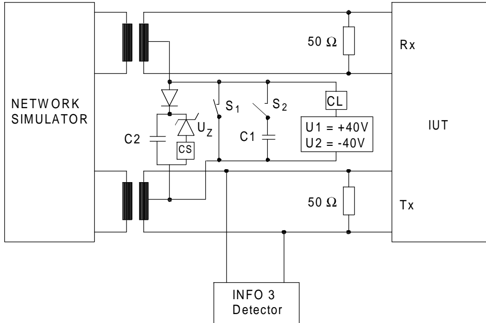
Figure 54: Test configuration
