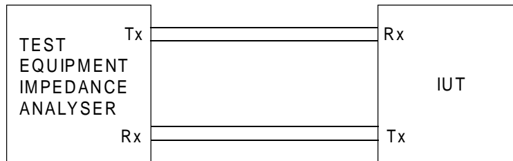
Figure 22: Test configuration
