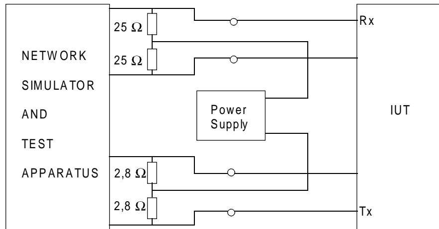
Figure 31: Test configuration
