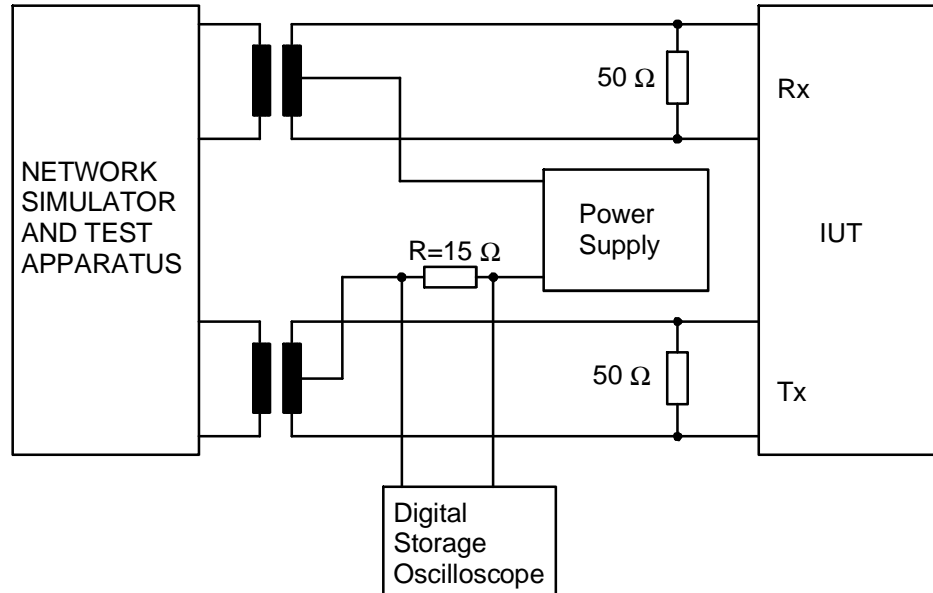
Figure 50: Test configuration
