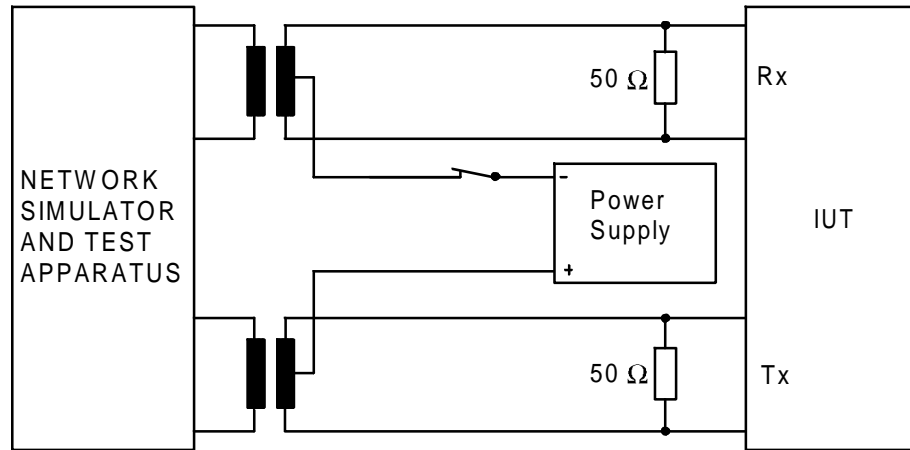
Figure 56: Test configuration
