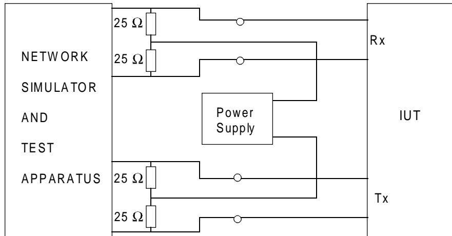
Figure 29: Test configuration
