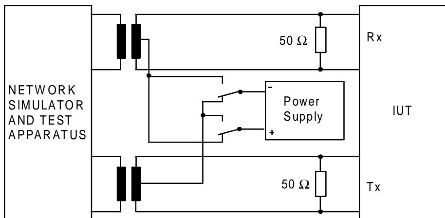
Figure 62: Test configuration
