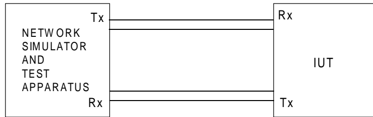
Figure 18: Test configuration
