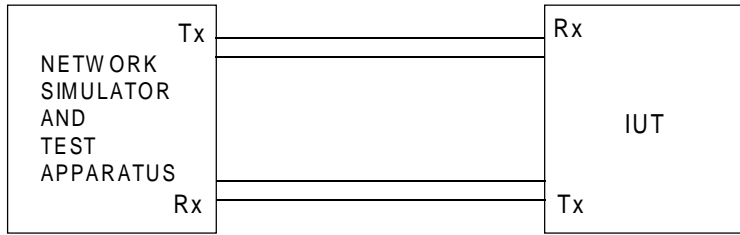
Figure 11: Test configuration
