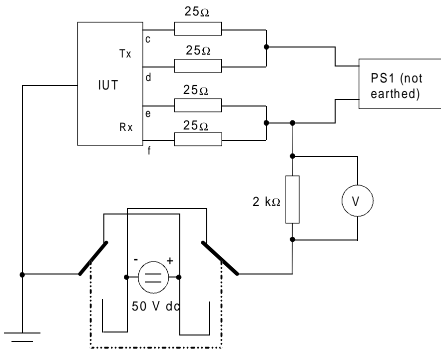
Figure 68: Test configuration
