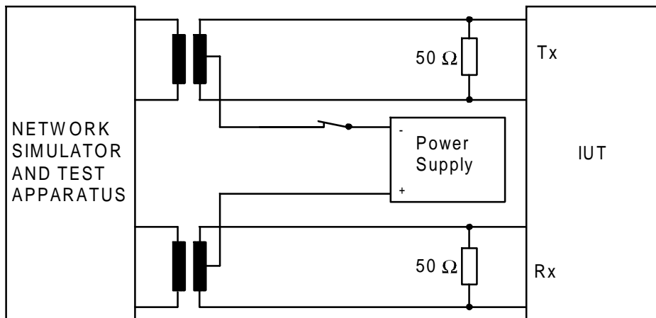
Figure 58: Test configuration
