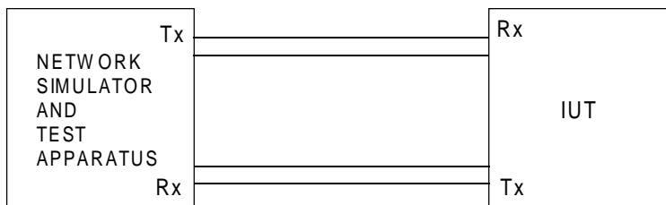
Figure 1: Test configuration
