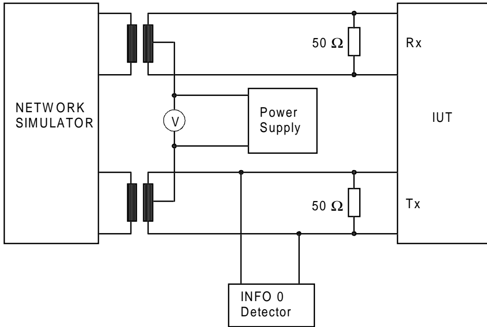
Figure 53: Test configuration
