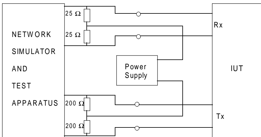
Figure 30: Test configuration
