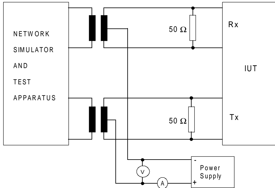
Figure 48: Test configuration
