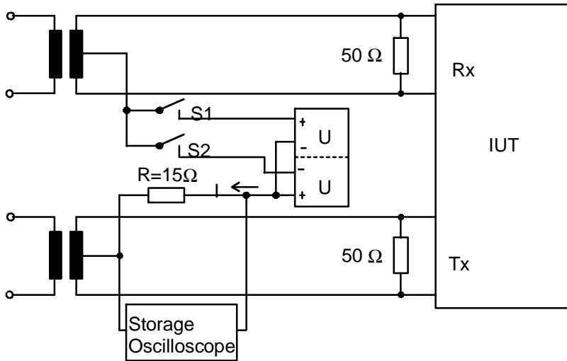
Figure 51: Test configuration
