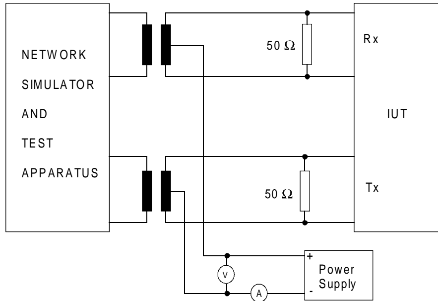
Figure 44: Test configuration
