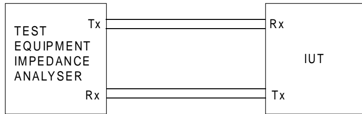
Figure 35: Test configuration
