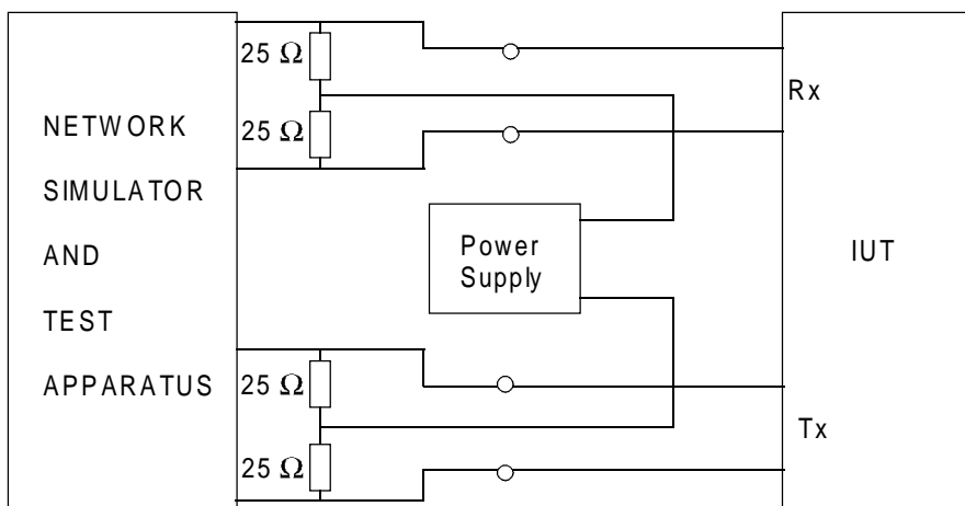
Figure 38: Test configuration
