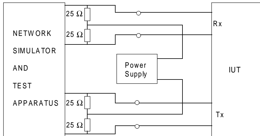
Figure 27: Test configuration
