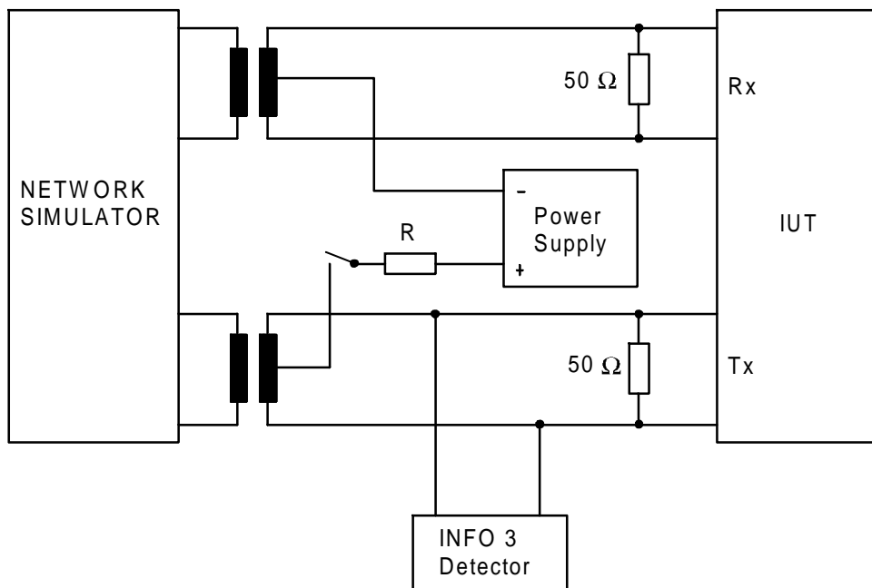
Figure 55: Test configuration
