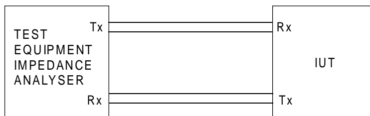
Figure 66: Test configuration 2
