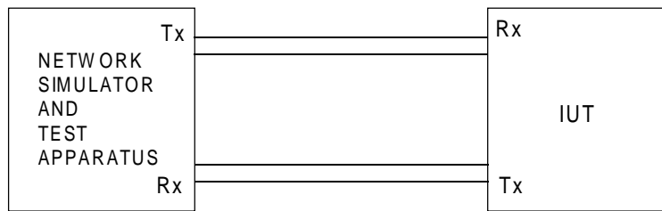
Figure 17: Test configuration
