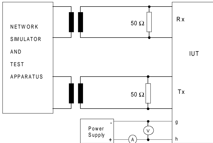
Figure 67: Test configuration
