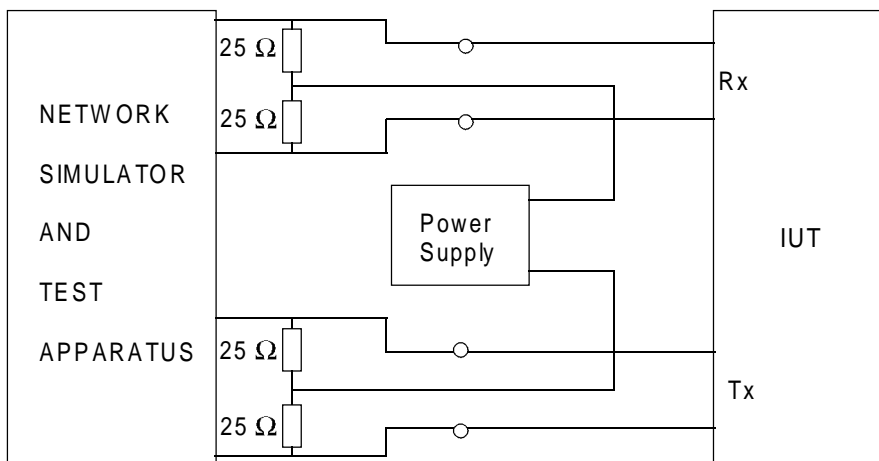
Figure 28: Test configuration
