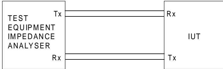
Figure 26: Test configuration
