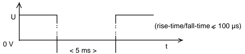
Figure 57: Characteristics of PS1 voltage
