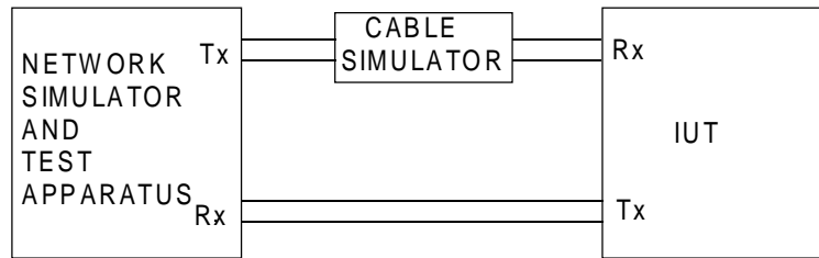
Figure 37: Test configuration
