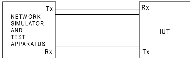
Figure 8: Test configuration
