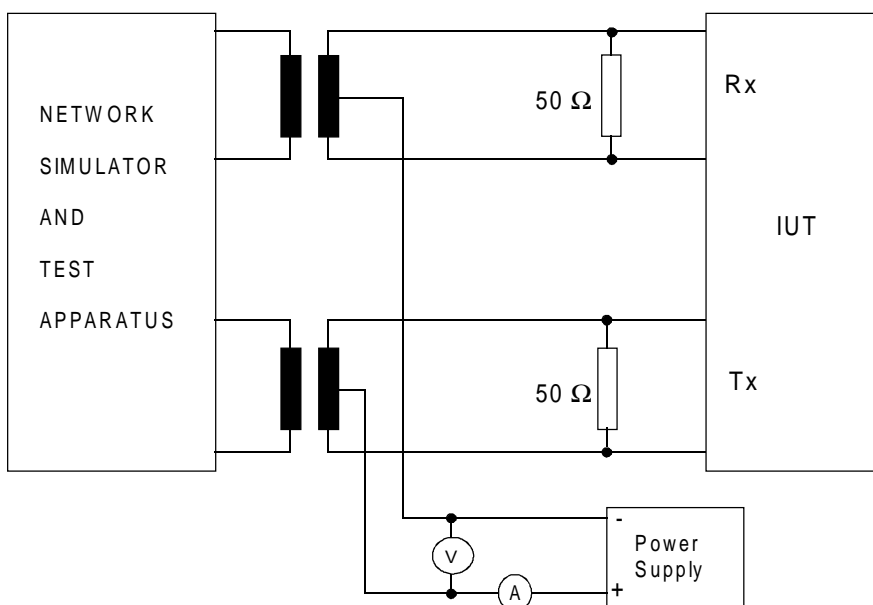
Figure 39: Test configuration
