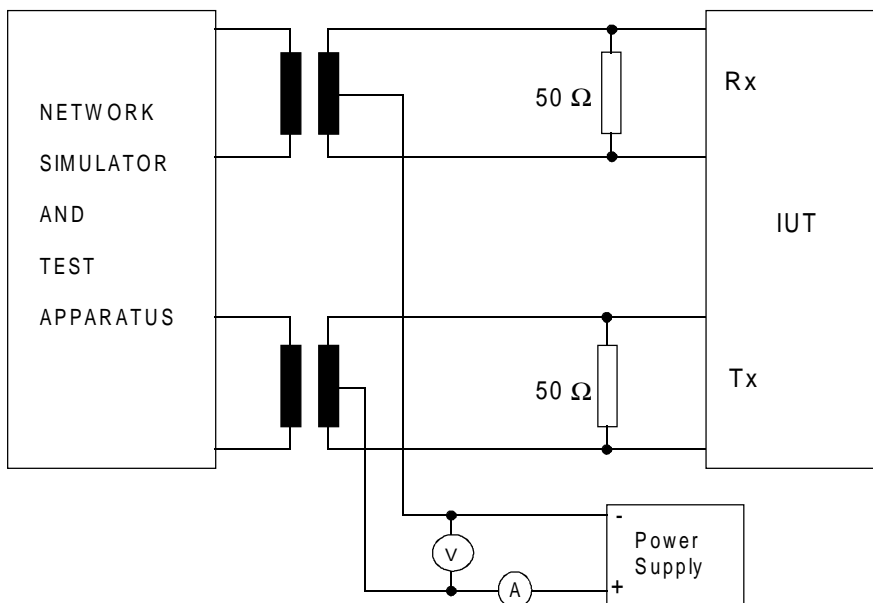
Figure 43: Test configuration
