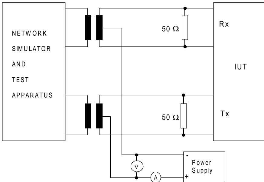
Figure 41: Test configuration
