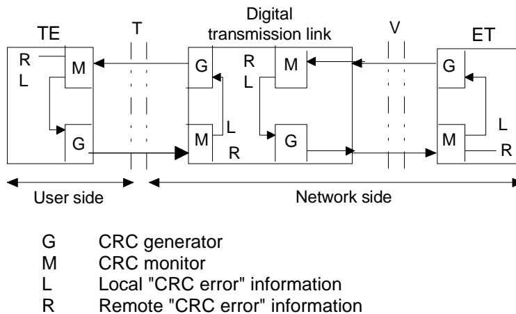
Figure 7: Localization of CRC processing functions for a subscriber access with CRC processing in the transmission link
