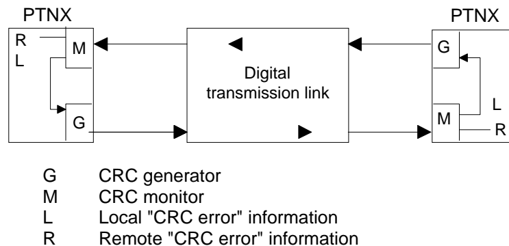
Figure 6: Localization of CRC processing functions for PTNX interconnection when the transmission link does not process the CRC
