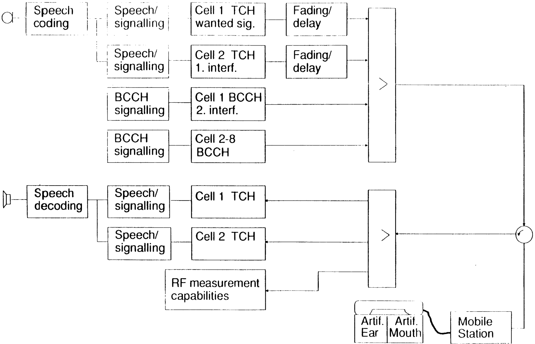
General configuration for some signalling tests and radio measurements
