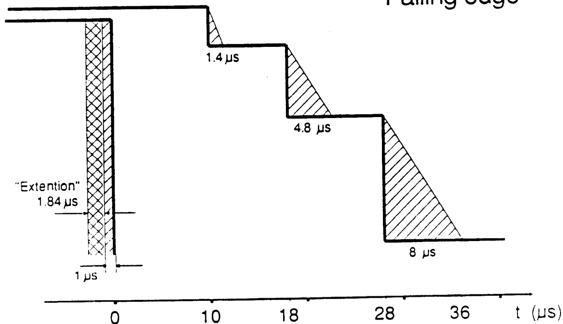
FIGURE App.3-1 / GSM 11.40 : Time Measurement Uncertainty for the Power Time Mask
