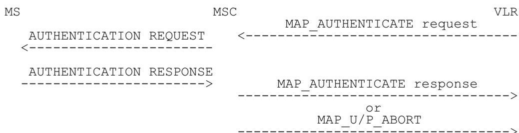
Figure 2: Authentication operation
