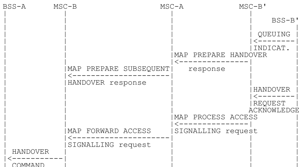
Figure 17: Signalling for Subsequent Inter-MSC Handover to third MSC (MSC-B') execution (Positive outcome)
