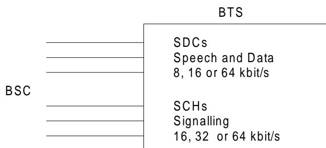
Figure 6.1/08.52: Communication Channel Types
