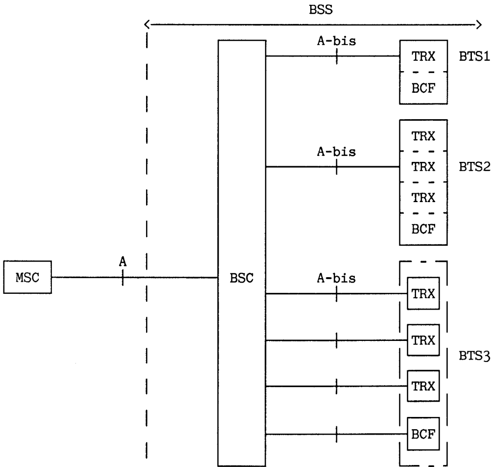
Figure 3.1/08.52. BSS Subdivision and Interfaces.
