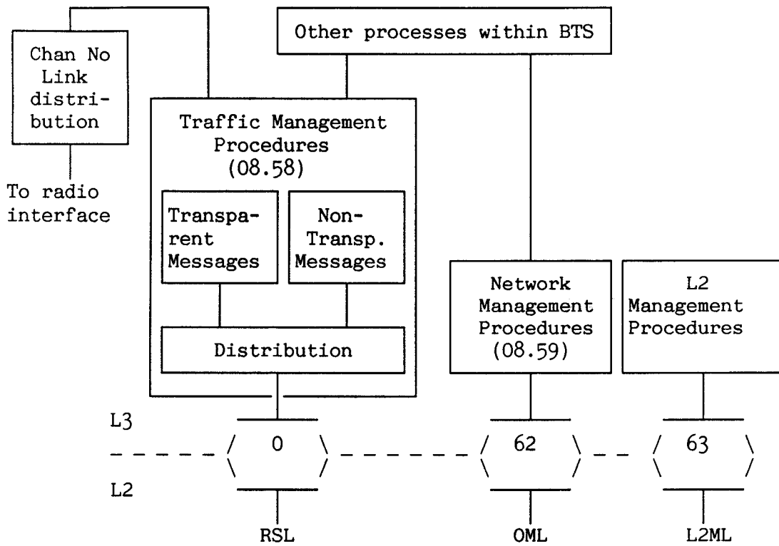
Figure 6.4/08.52 L3 model.
