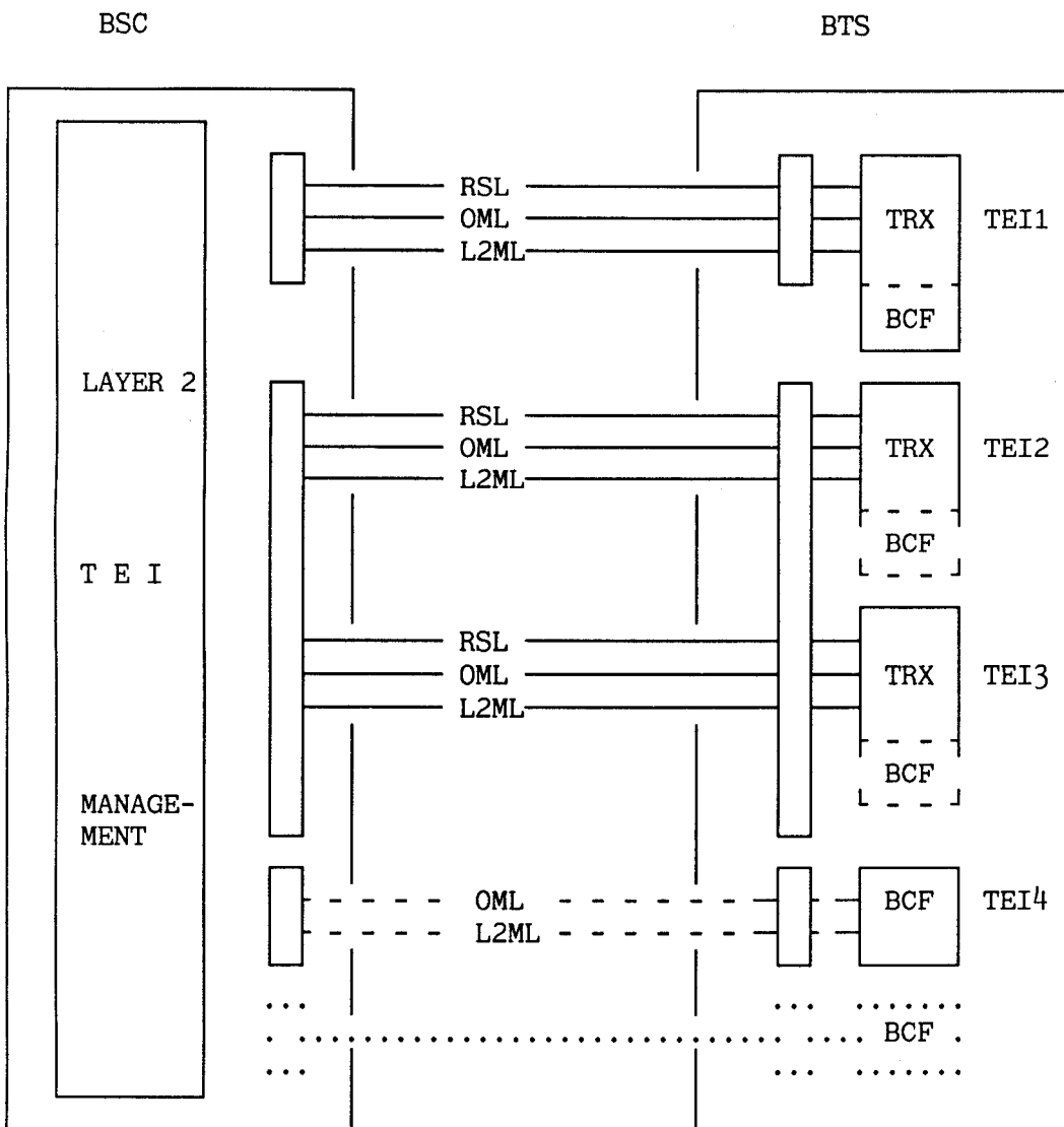
Figure 6.2/08.52 Logical L2 links of A-bis interface.
