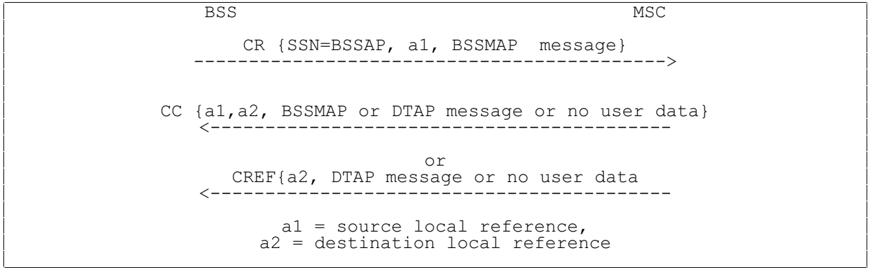
Figure 1/08.06 Set-up of SCCP connections on the first BSS/MSC interface
