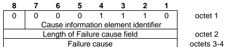
Figure 2.5.16/GSM 07.05: TP-Failure Cause information element
