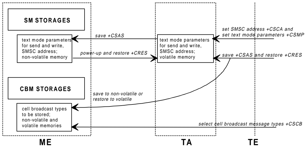
Figure 1: Message service parameter procedures
