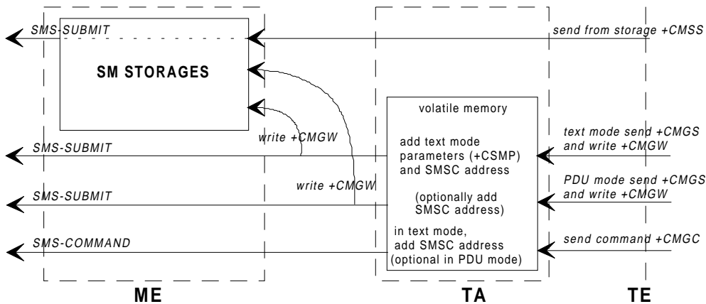
Figure 4: Message service send and write procedures
