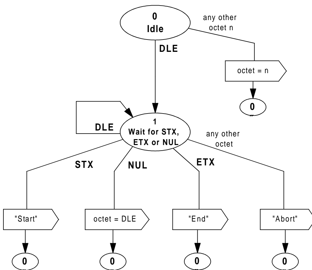
State transitions in Stage 1
