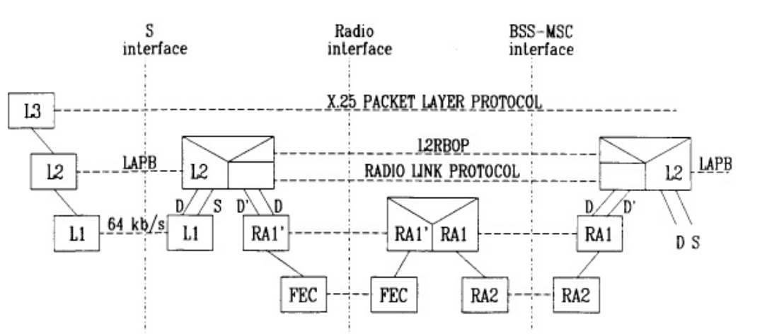
Figure 9: X.25 access at S-interface using Flag Stuffing
