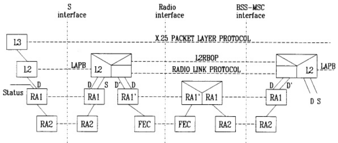
Figure 8: X.25 access at S-interface
