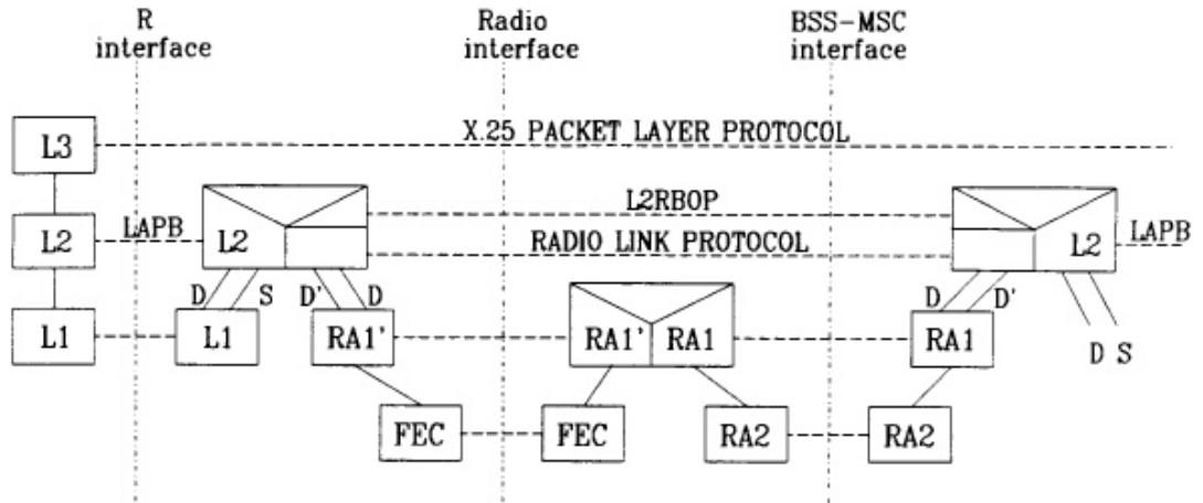
Figure 7: X.25 access at R-interface
