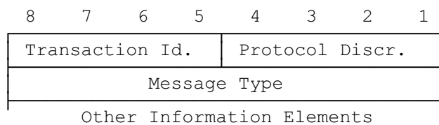
Figure 8.1/GSM 04.11.
