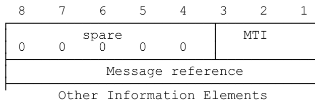
Figure 8.4/GSM 04.11.
