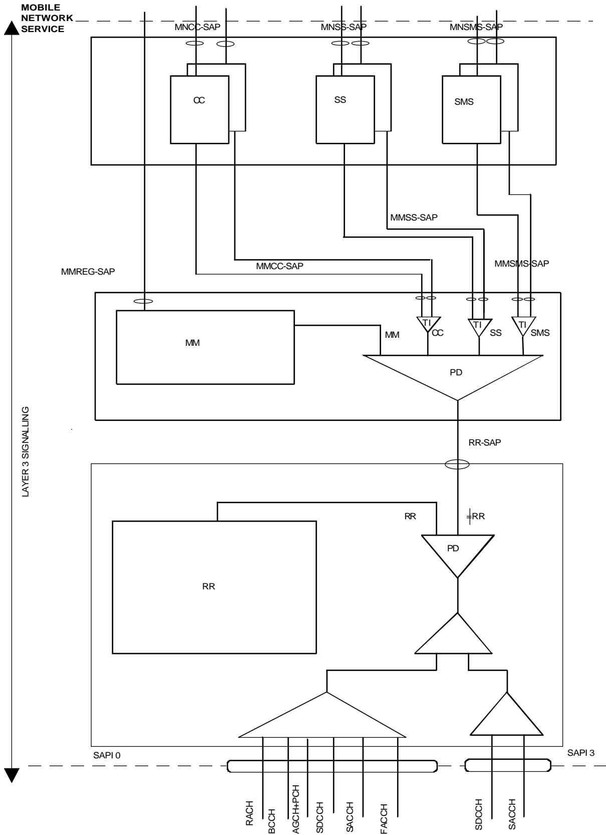
Figure 5.1/GSM 04.07 Protocol Architecture of Signalling Layer 3 - Mobile Station side
