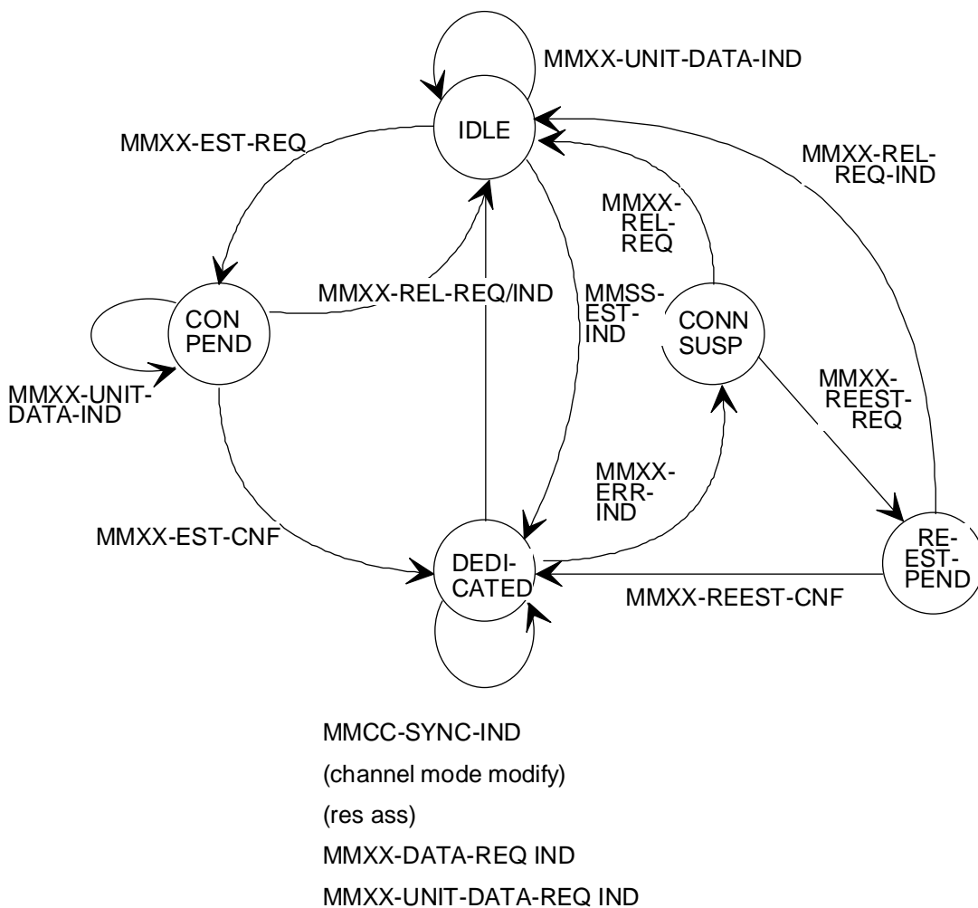
Figure 9.4/GSM 04.07 Service graph of the Mobility Management entity - Mobile Station side
