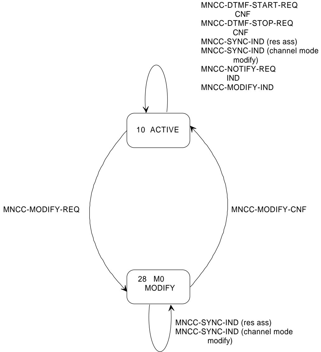
Figure 6.2/GSM 04.07 Service graph of Call Control entity - Mobile Station side Active state (page 2 of 2)
