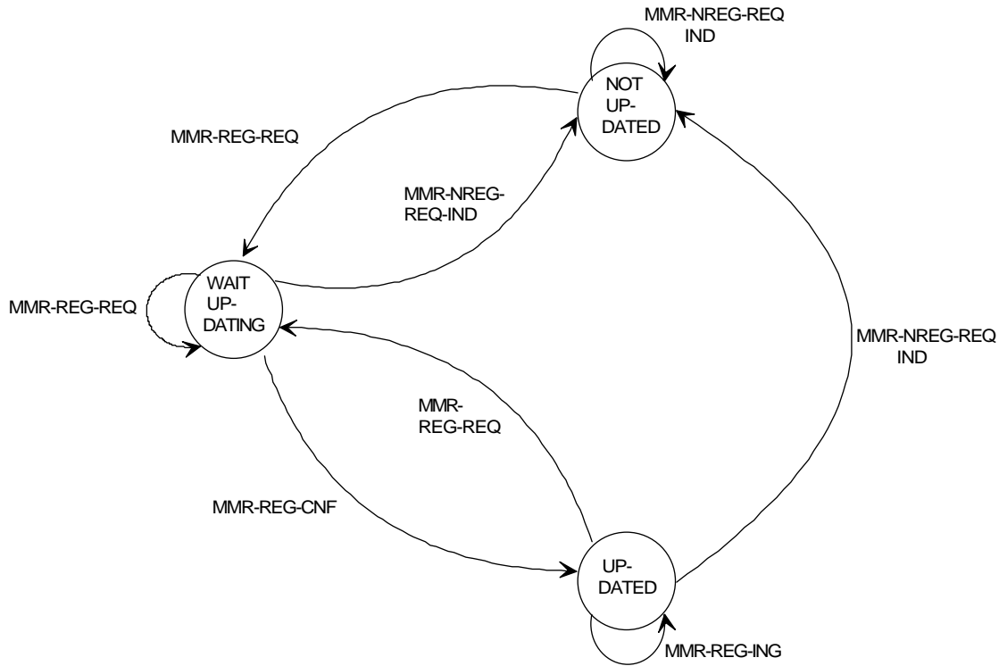
Figure 6.1/GSM 04.07 Registration services provided at MMREG-SAP - Mobile Station side
