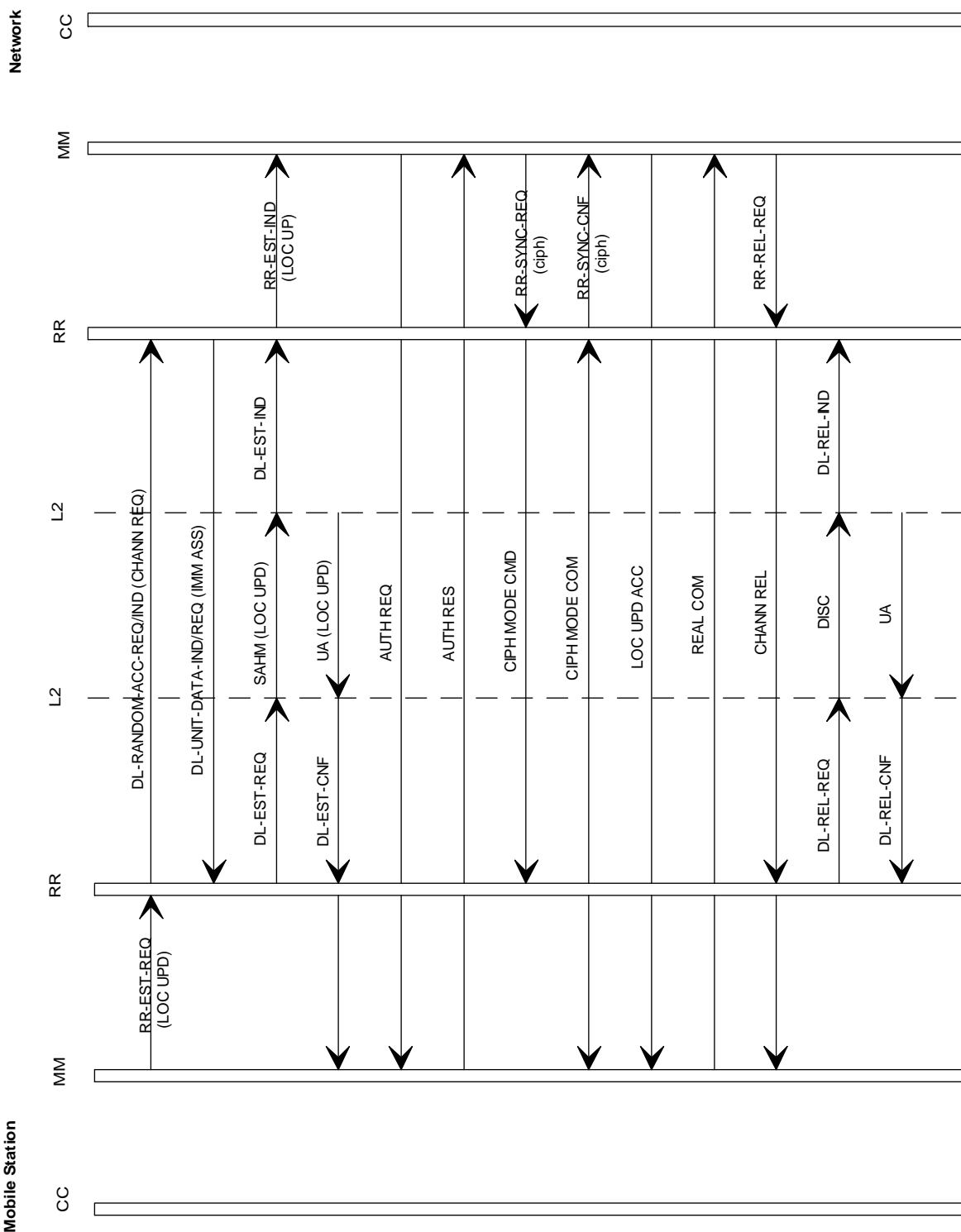
Figure A.4 Location updating. Successful case.
