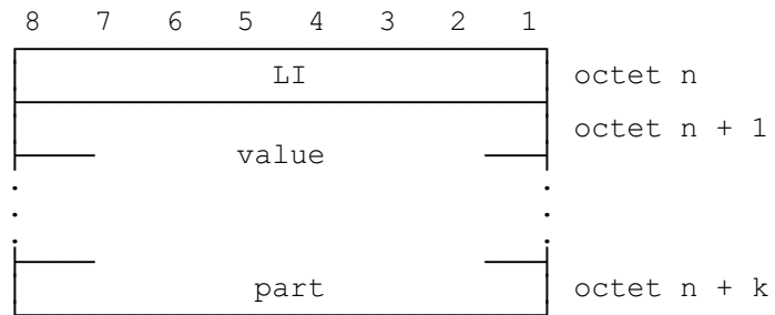
Figure 11.7/GSM 04.07 Type 4 IE of format LV (k = 0, 1, 2, ...)
