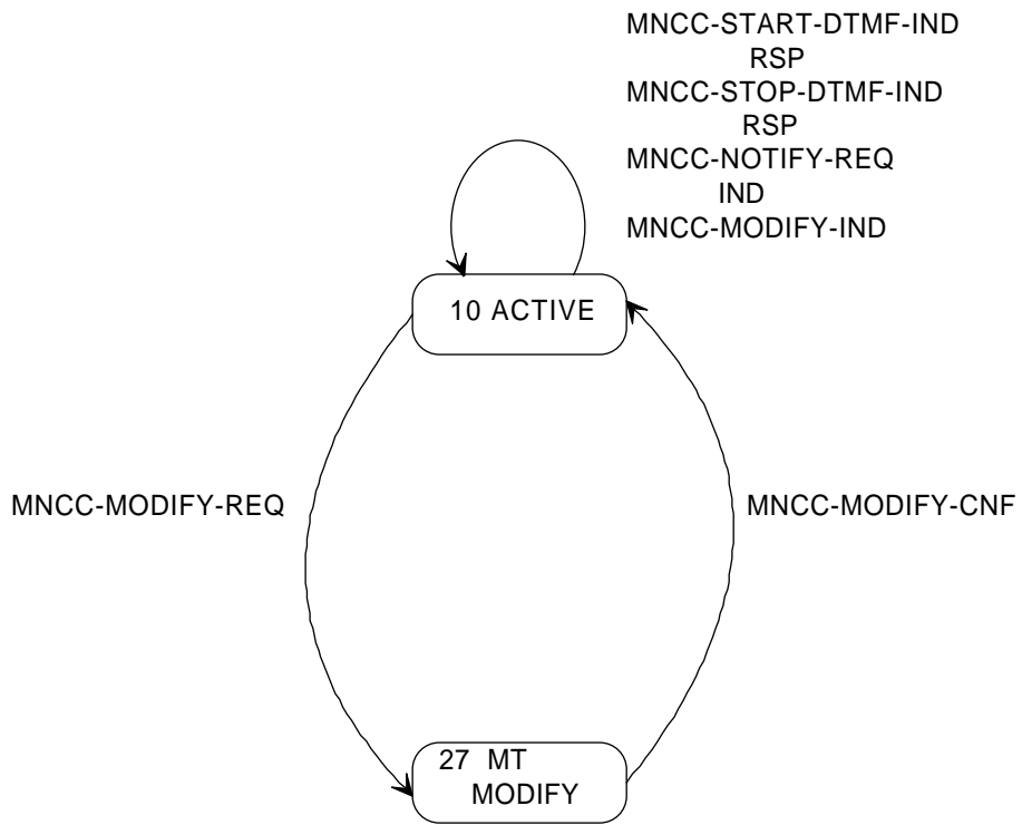
Figure 7.1/GSM 04.07 (page 2 of 2) Service graph of Call Control entity - Network side
