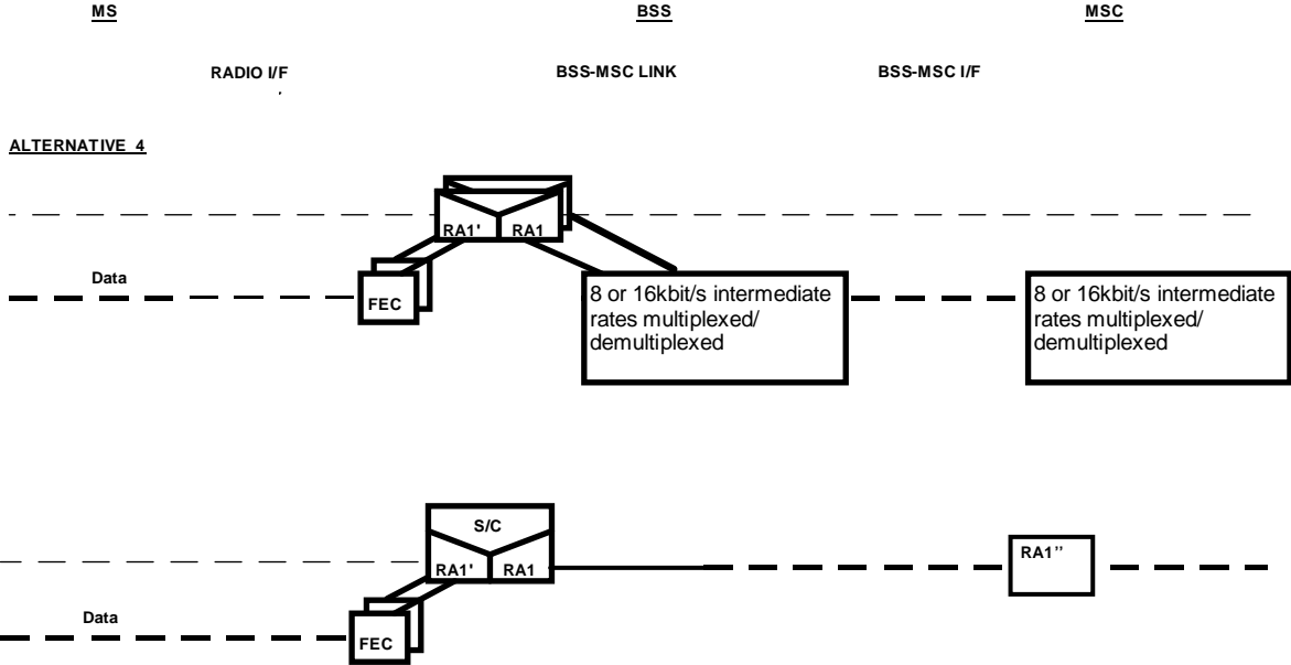
Figure 7 (concluded): Location of transcoding and rate adaptation
