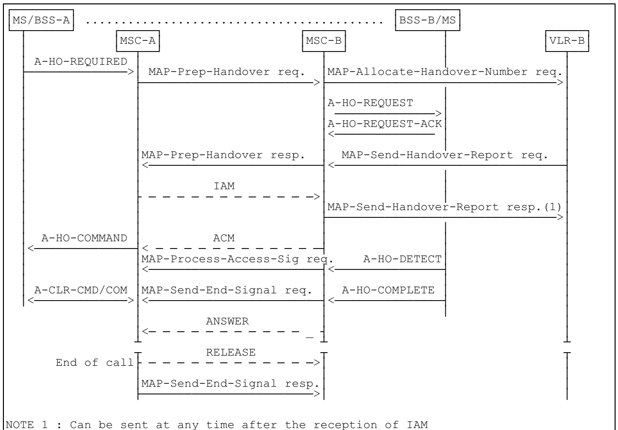
Figure 5: Basic Handover Procedure requiring a circuit connection
