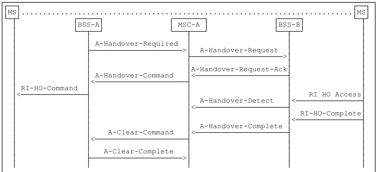
Figure 4: Basic External Intra-MSC Handover Procedure
