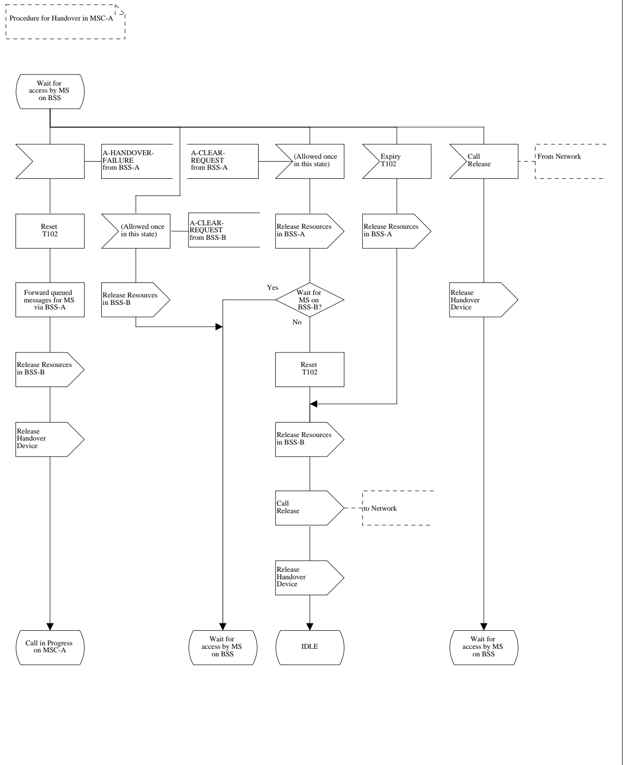
Figure 13 (Sheet 4 of 26): Handover control procedure in MSC-A
