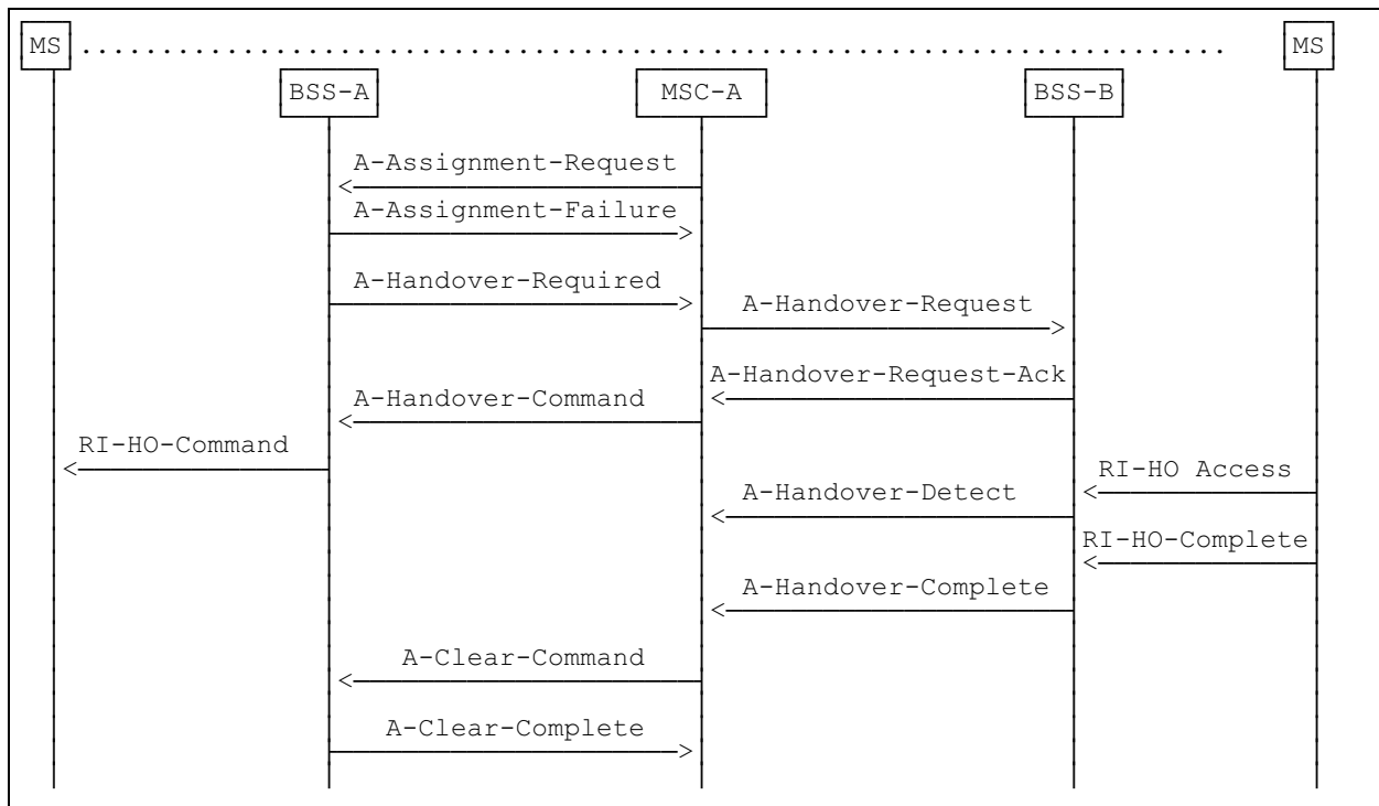
Figure 12: Example of a Directed Retry Intra-MSD Handover Procedure
