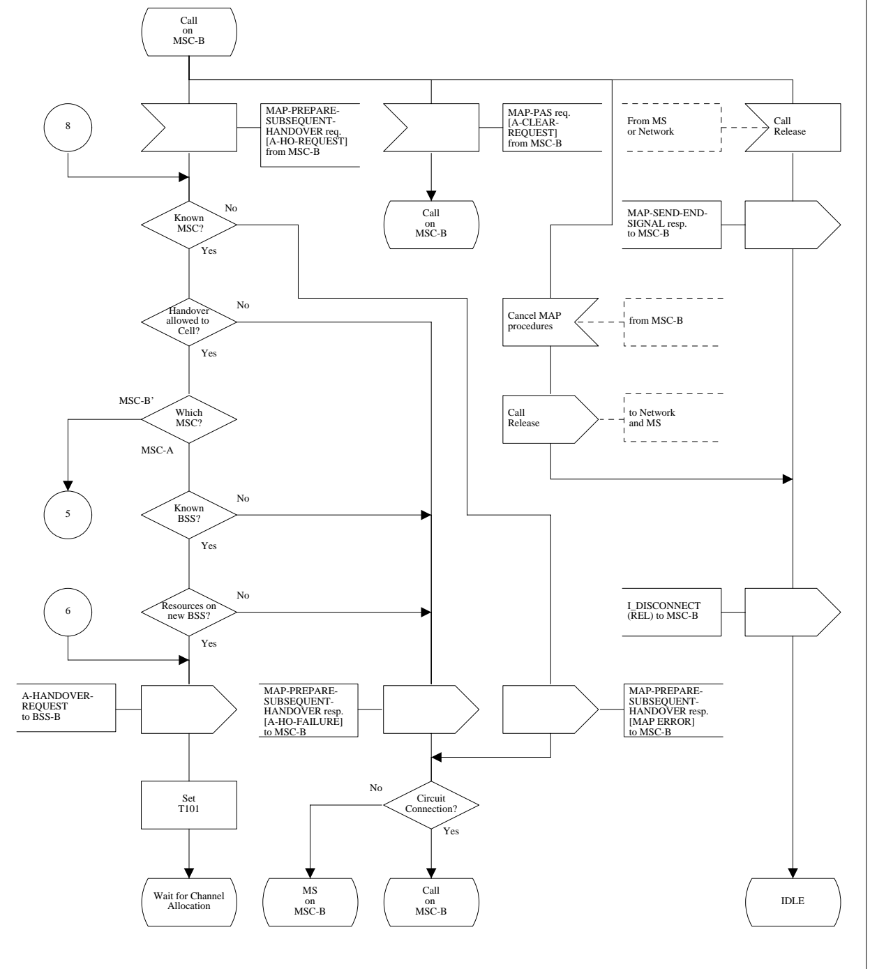
Figure 13 (Sheet 10 of 26): Handover control procedure in MSC-A
