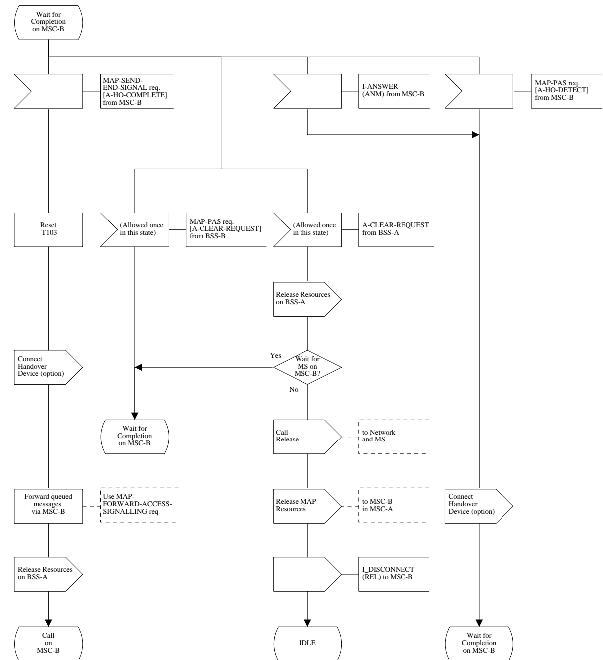
Figure 13 (Sheet 8 of 26): Handover control procedure in MSC-A
