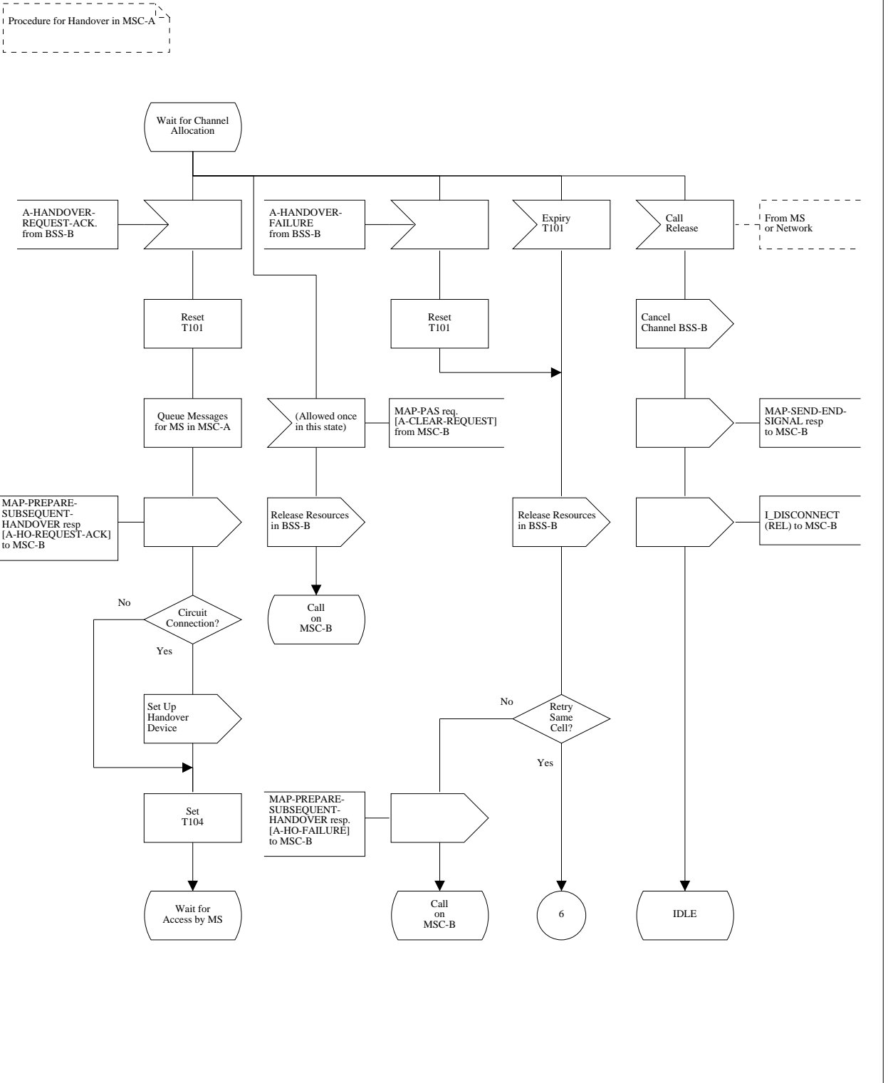
Figure 13 (Sheet 11 of 26): Handover control procedure in MSC-A
