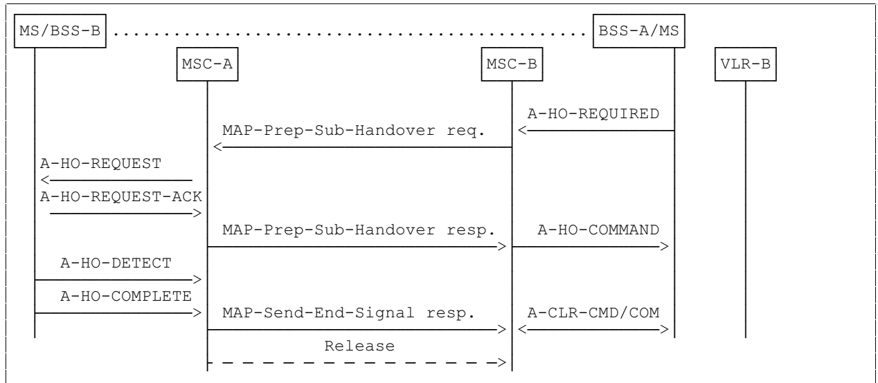
Figure 7: Subsequent handover procedure i):successful handover from MSC-B to MSC-A using a circuit connection
