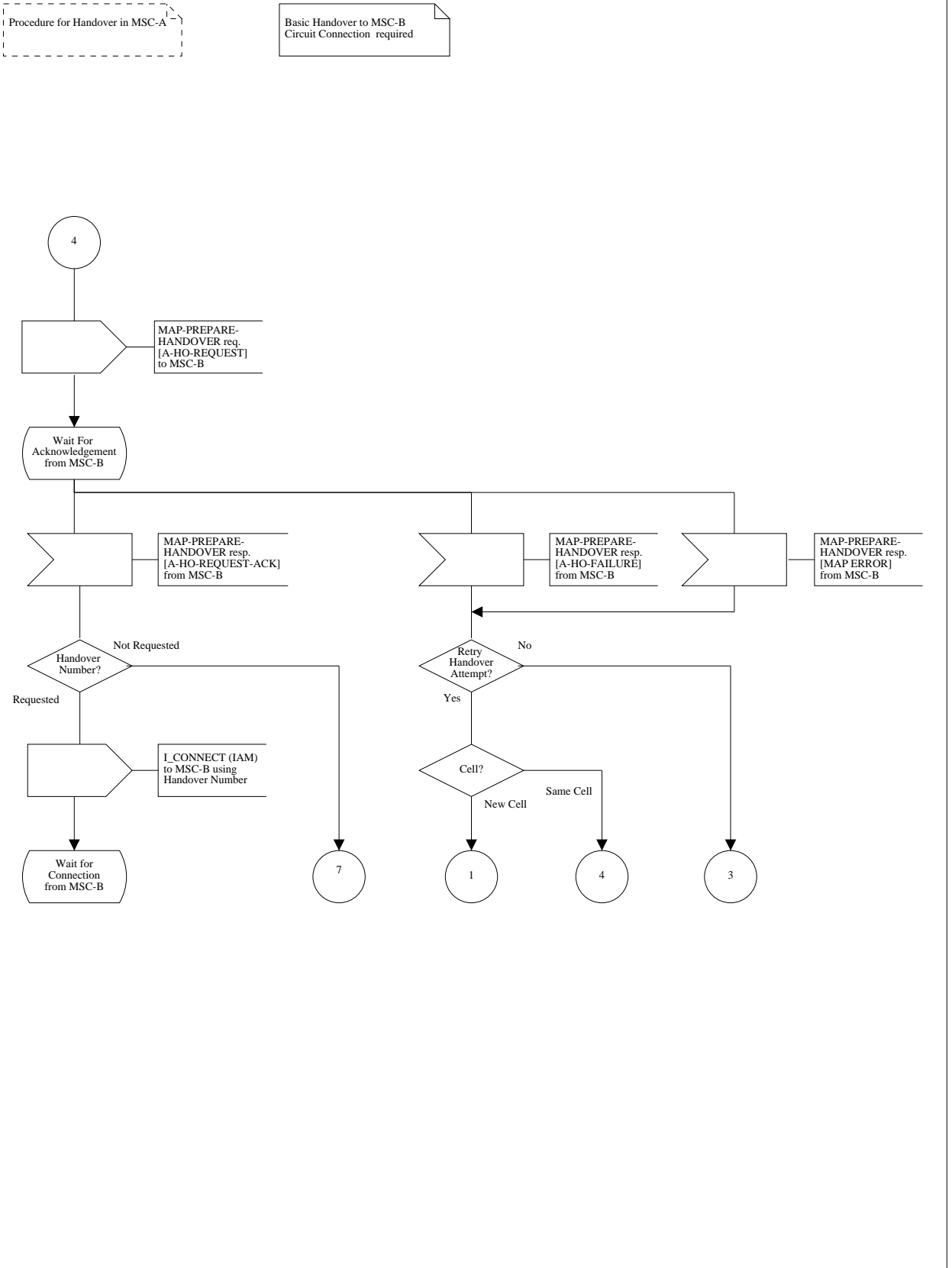
Figure 13 (Sheet 5 of 26): Handover control procedure in MSC-A
