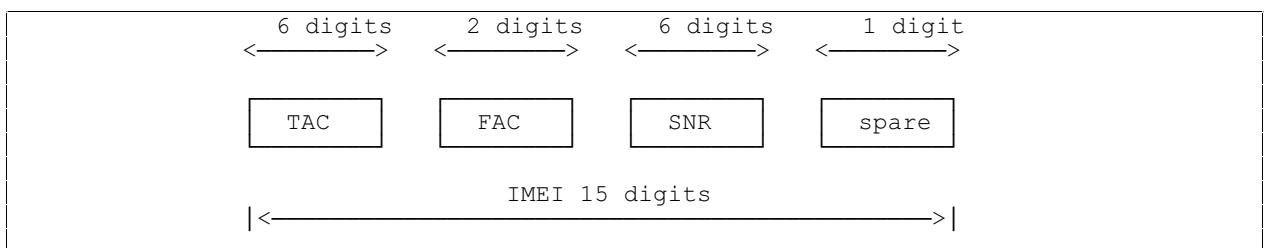
Figure 8: Structure of IMEI
