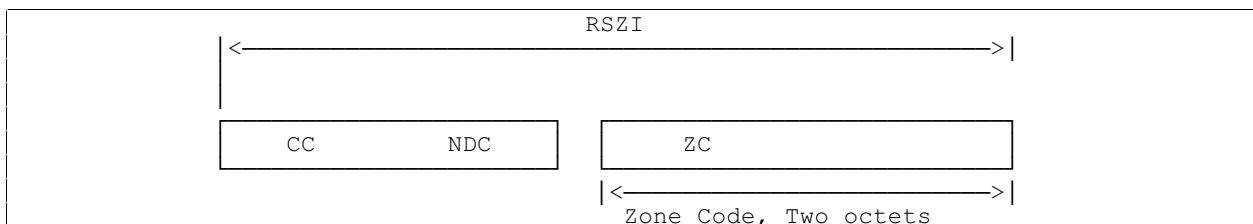
Figure 6: Structure of Regional Subscription Zone Identity (RSZI)
