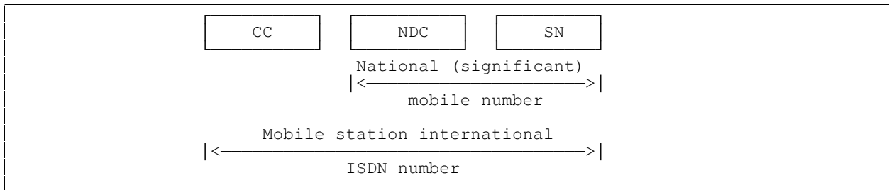
Figure 2: Number Structure of MSISDN
