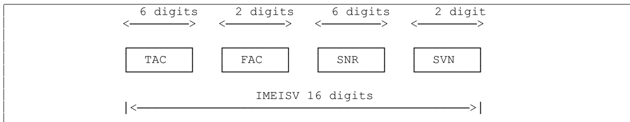
Figure 9: Structure of IMEISV
