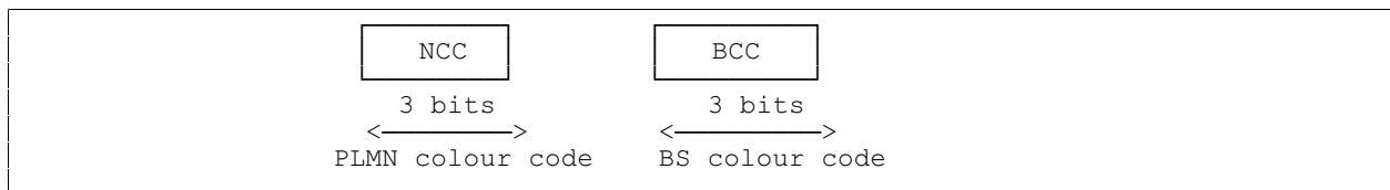
Figure 5: Structure of BSIC
