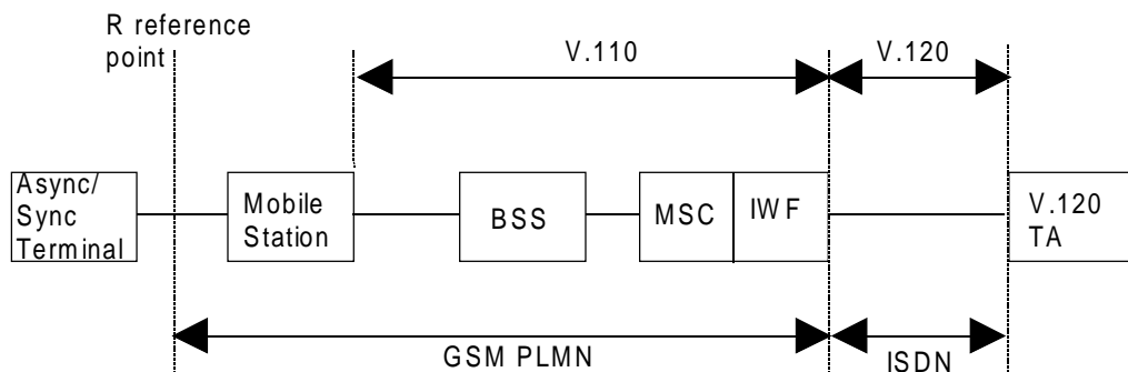
Figure 2/GSM 02.02: Model of GSM V.120 Interworking
