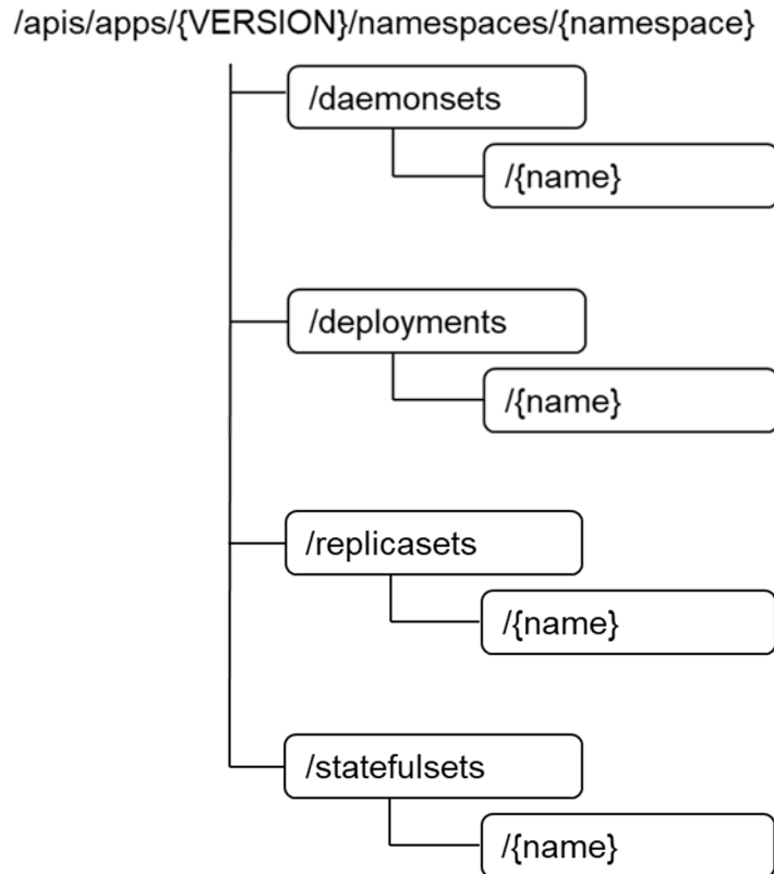
Figure 8.3-2: Resource URI structure of DaemonSet, Deployment, ReplicaSet, StatefulSet resource objects for the OS container compute management service interface
