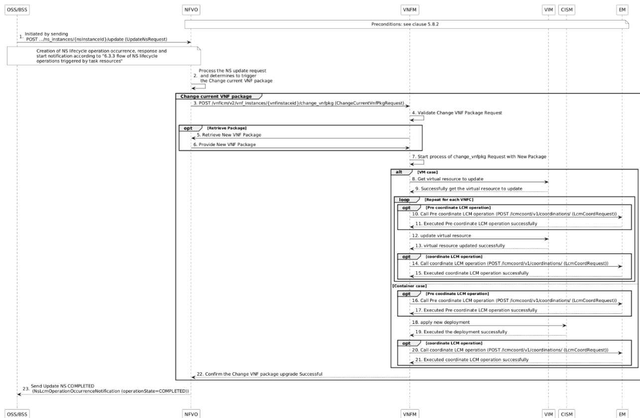
Figure 5.8.3.2-1: Procedure flow of Change current VNF package using Rolling upgrade
