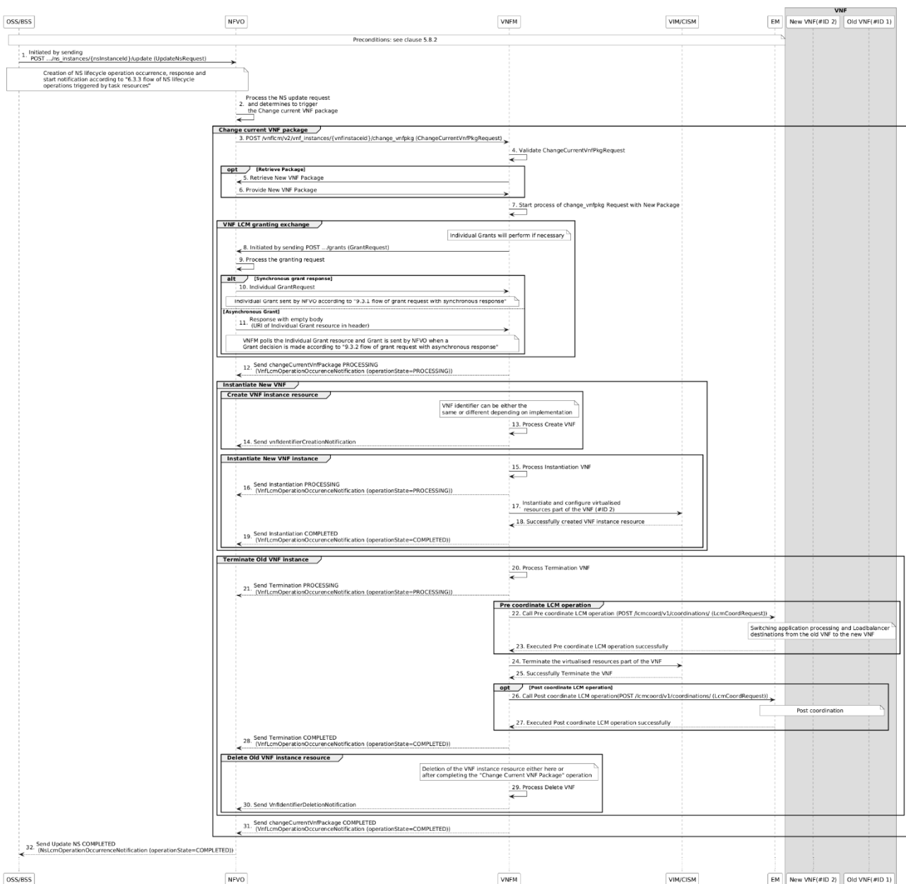
Figure 5.8.3.3-1: Procedure flow of Change current VNF package using Blue-green
