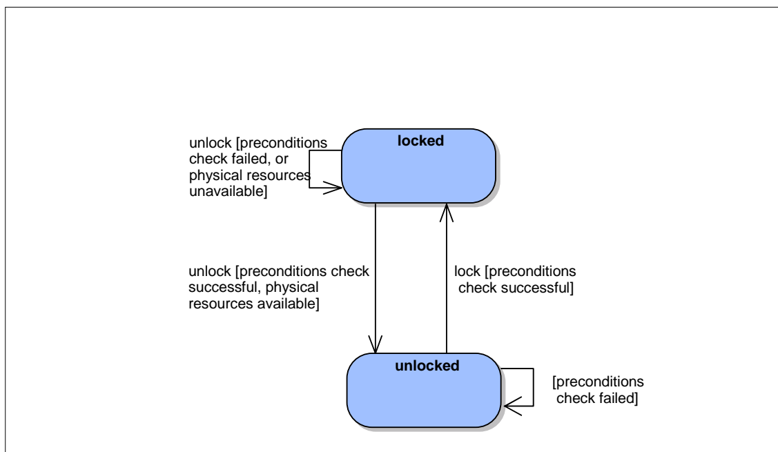
Figure 6.7.1.1-1: AST state transition diagram
